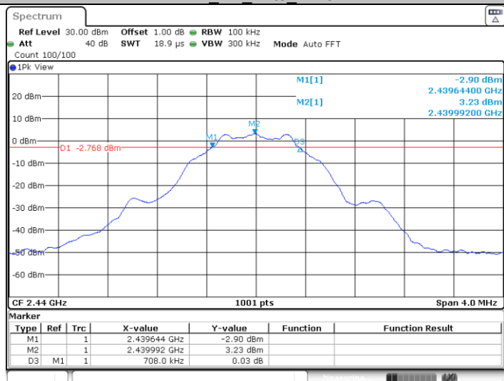
BLE_1M_Ant0_2440
