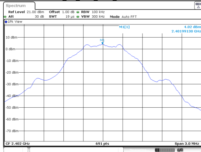
BLE_1M_Ant0_2402_0-Reference
