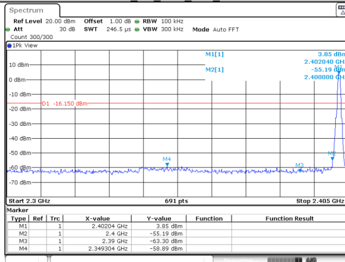
BLE_1M_Ant0_Low_2402
