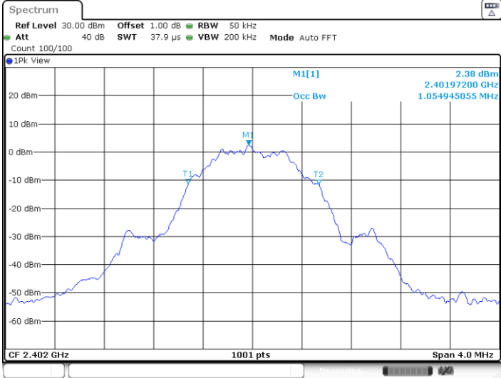
BLE_1M_Ant0_2402
