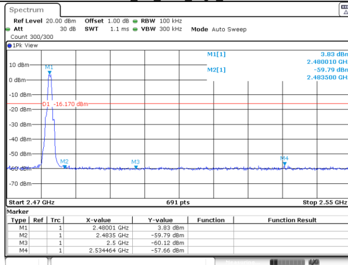
BLE_1M_Ant0_High_2480
