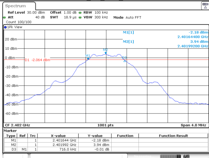
BLE_1M_Ant0_2402
