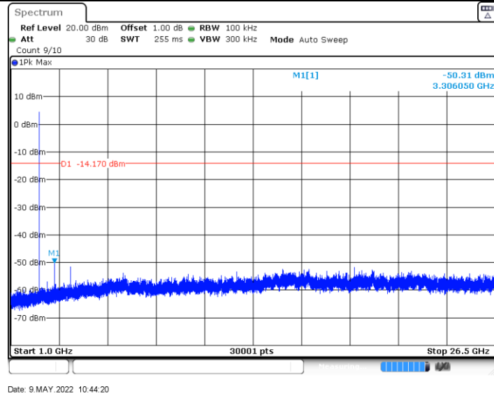
2DH5_Ant0_2402_0~Reference
