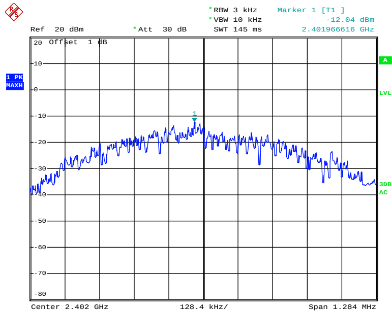
Power Spectral Density, BLE-1M Low Channel
