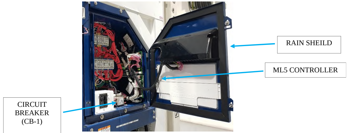
Figure 1: Control Box with Door Open
