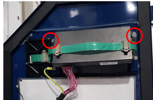
Figure 2b: Screws reinstalled
