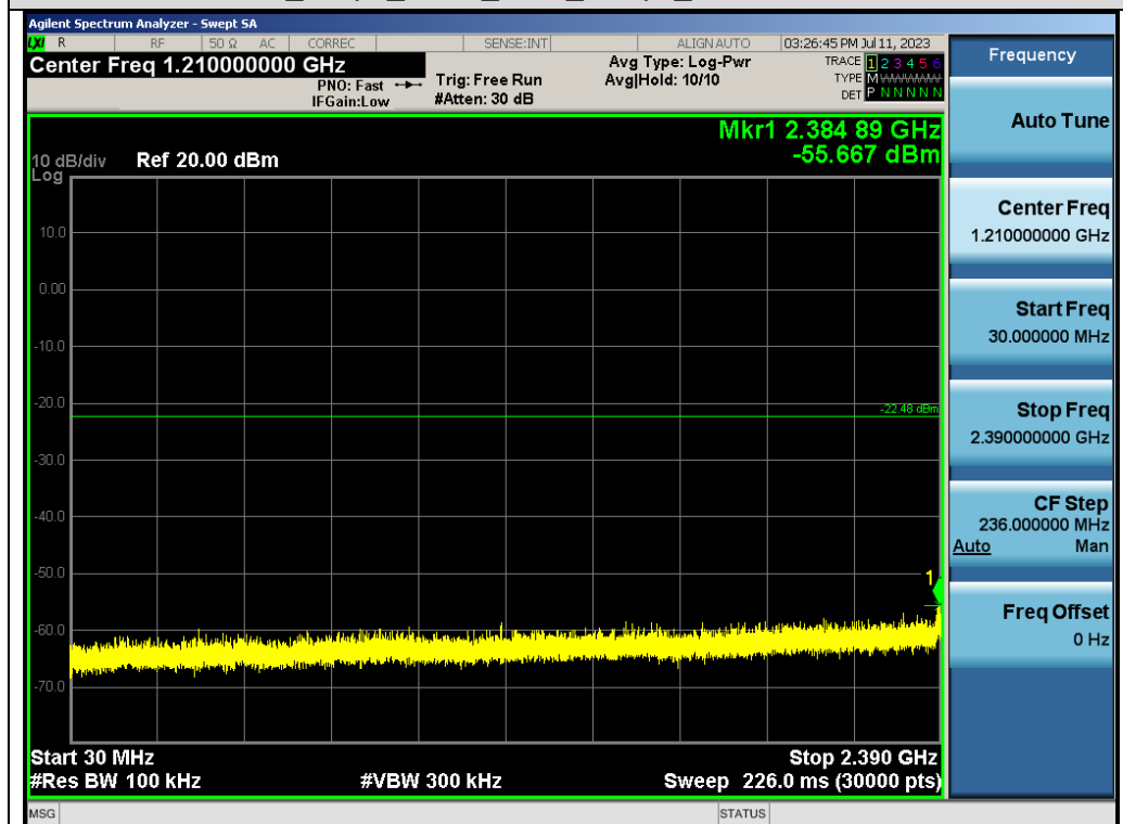
Test_Graph_ANT1_2402_1Mbps_Lower Band Emissions
