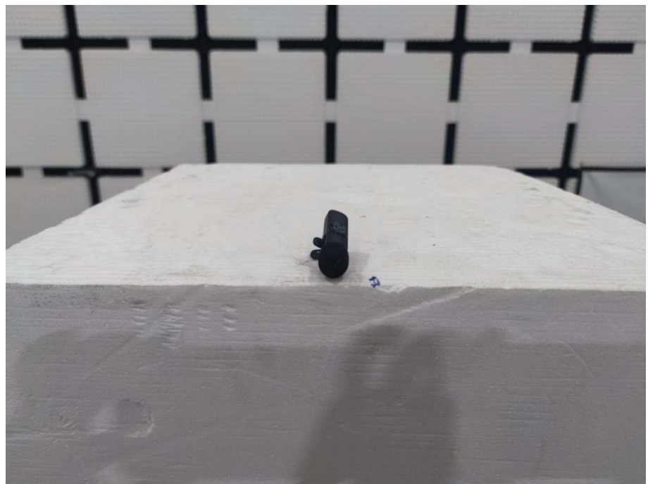
Radiation Emission Test Setup View
