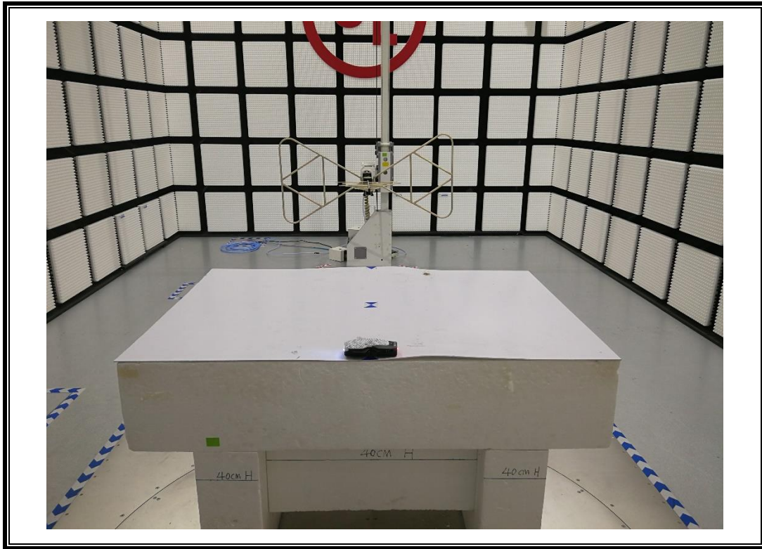
RADIATED RF MEASUREMENT SETUP for 2.4G function (30MHz ~ 1 GHz)
