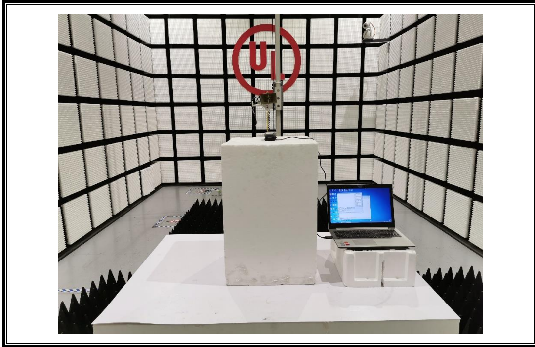
RADIATED RF MEASUREMENT SETUP for 2.4G WiFi function (Above 1G – X axis)
