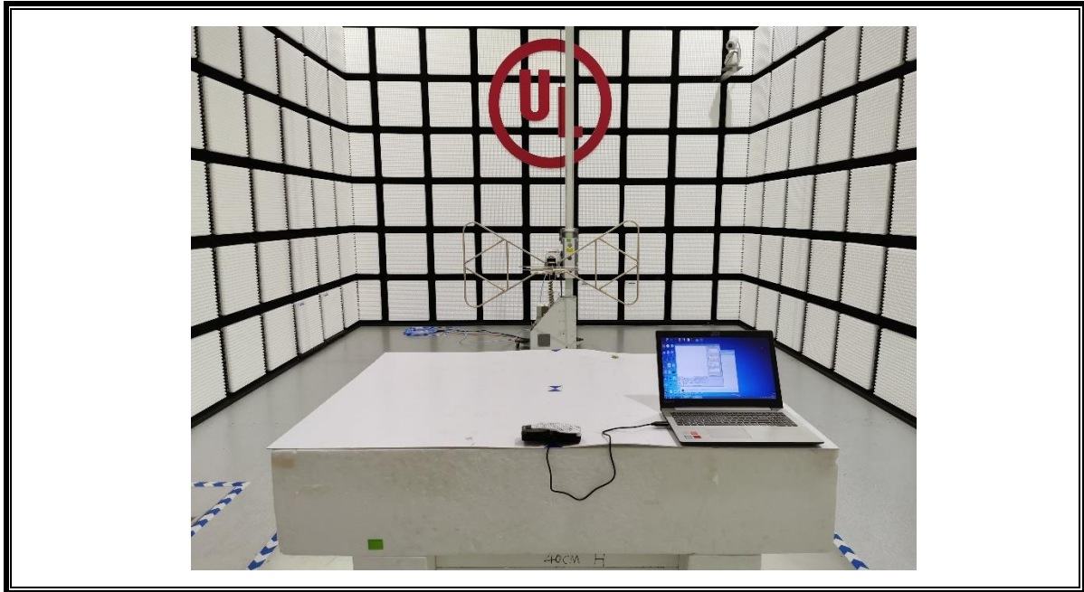
RADIATED RF MEASUREMENT SETUP for 2.4G WiFi function (30MHz ~ 1 GHz)
