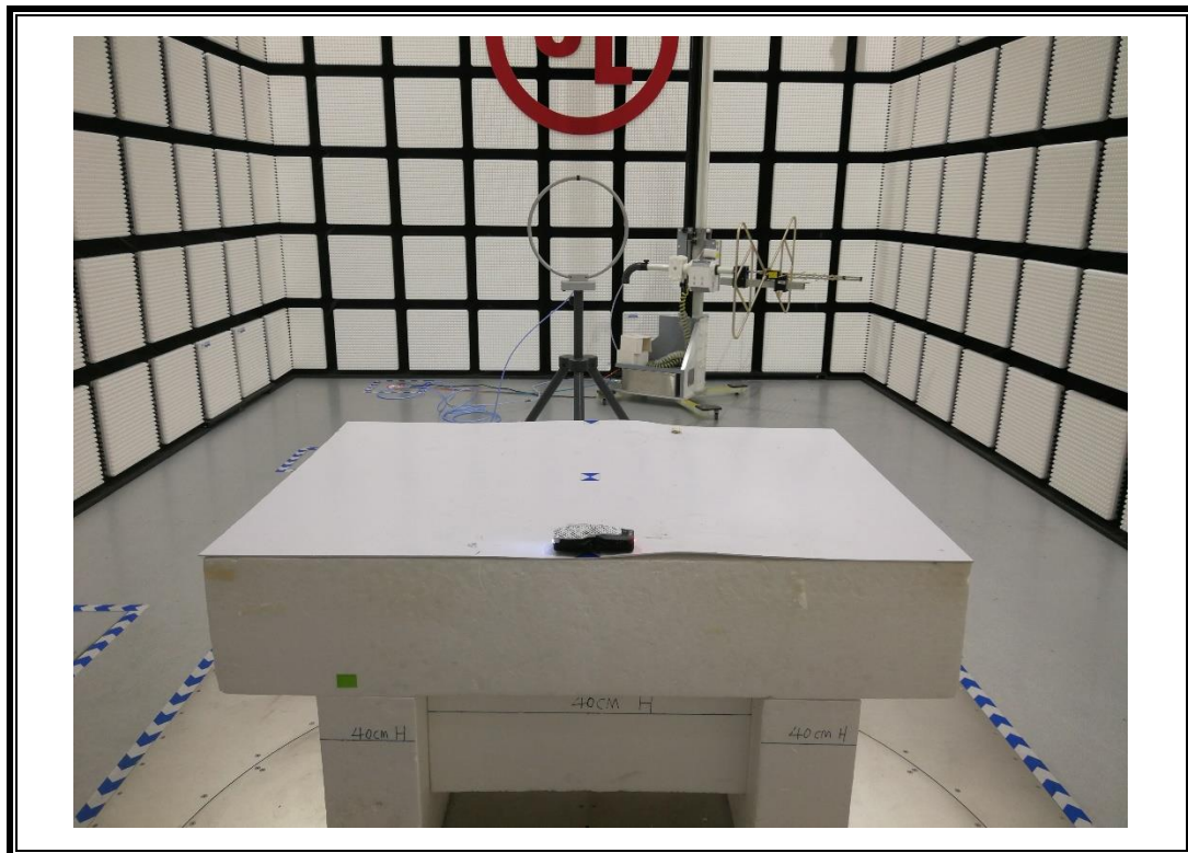
RADIATED RF MEASUREMENT SETUP for 2.4G function (Below 30MHz)
