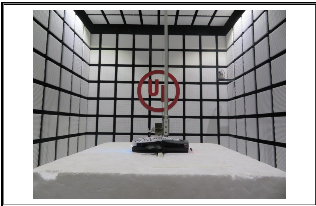
RADIATED RF MEASUREMENT SETUP for 2.4G function (Above 1G – X axis)
