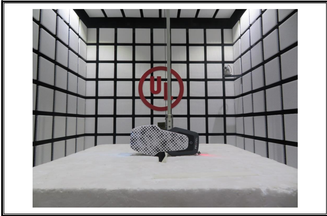
RADIATED RF MEASUREMENT SETUP for 2.4G function (Above 1G – Z axis)
