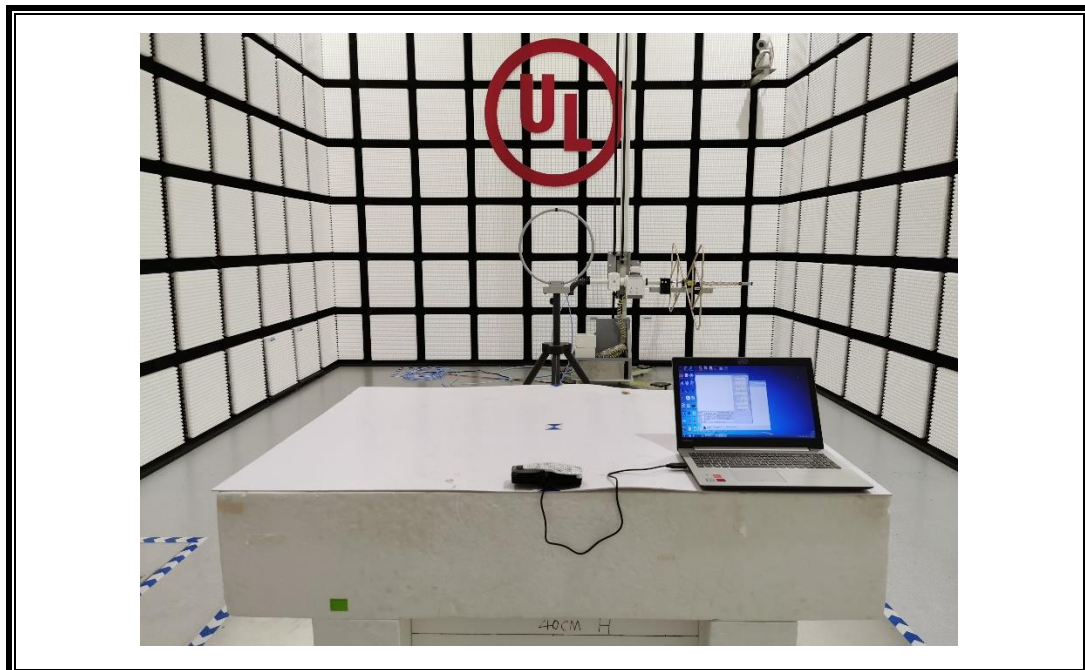
RADIATED RF MEASUREMENT SETUP for 2.4G WiFi function (Below 30MHz)
