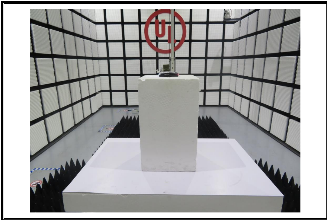
RADIATED RF MEASUREMENT SETUP for 2.4G function (Above 1G – X axis)
