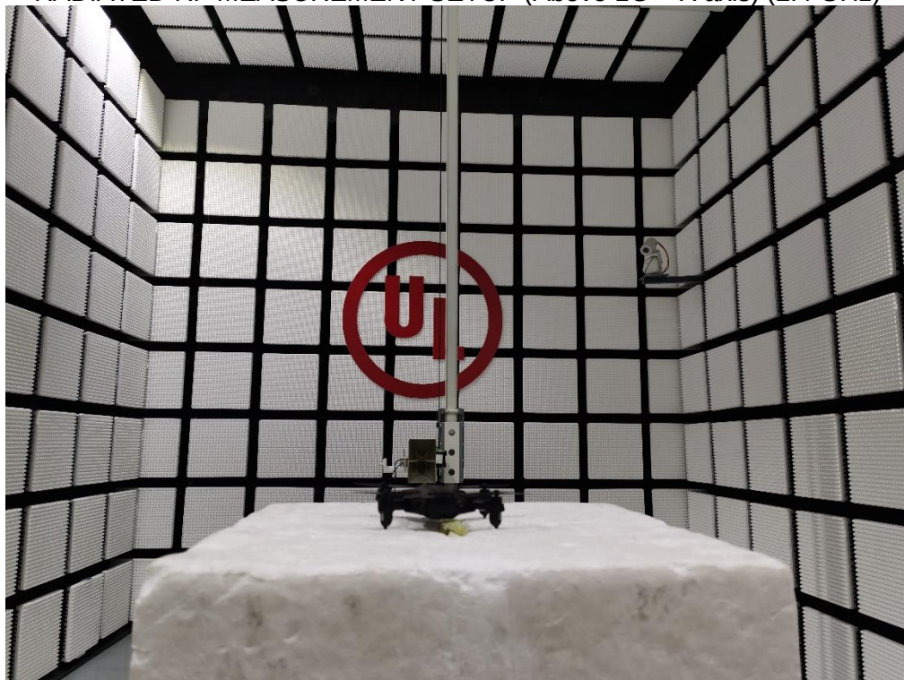
RADIATED RF MEASUREMENT SETUP (Above 1G – X axis) (2.4 GHz)
