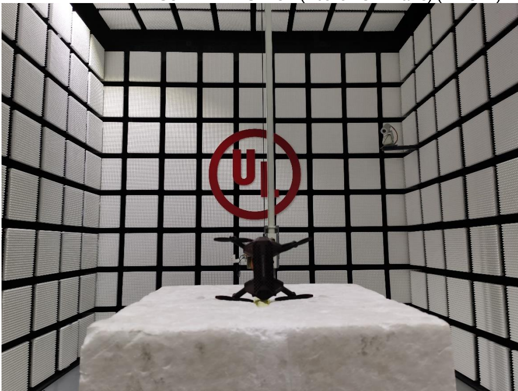
RADIATED RF MEASUREMENT SETUP (Above 1G – Z axis) (2.4 GHz)
