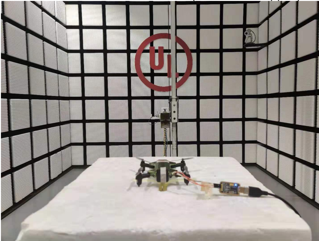
RADIATED RF MEASUREMENT SETUP (Above 1G – X axis) (WiFi)
