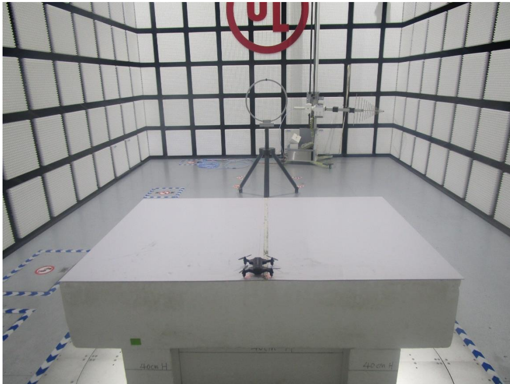
Radiated Disturbance below 30 MHz (2.4 GHz)
