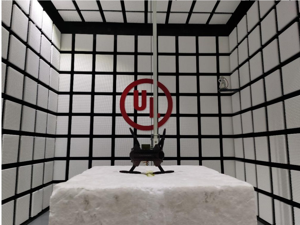
RADIATED RF MEASUREMENT SETUP (Above 1G – Y axis) (2.4 GHz)
