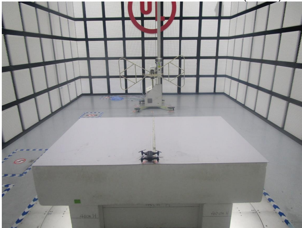
Radiated Disturbance below 1 GHz and above 30 MHz (2.4 GHz)
