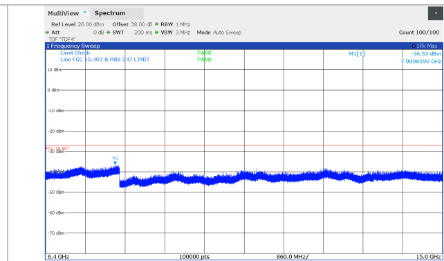
Figure 8.5-80: Conducted spurious emissions 6.4 – 15 GHz, 10 MHz Channel BW, Low channel (5794 MHz), SB1P Band
