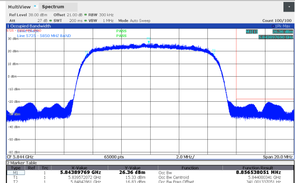
Figure 8.6-28: Frequency stability, 99% OBW, 10 MHz Channel BW, Highest channel (5844 MHz), SB2P Band (-10°C; -48 VDC)
