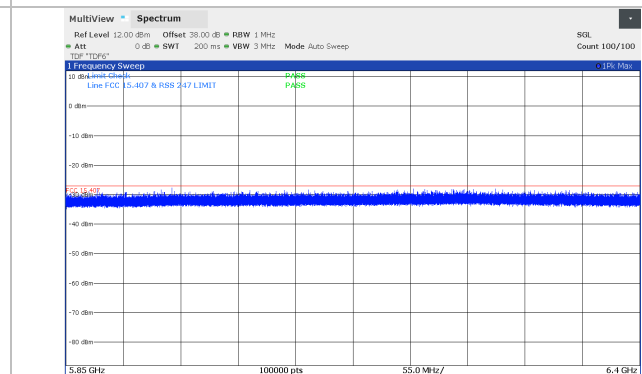
Figure 8.5-88: Conducted spurious emissions 5.850 – 6.4 GHz, 10 MHz Channel BW, Middle channel (5804 MHz), SB1P Band
