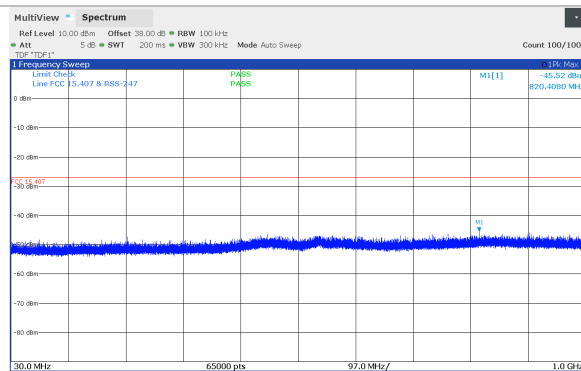
Figure 8.5-114: Conducted spurious emissions 0.03 - 1 GHz, 10 MHz Channel BW, Low channel (5824 MHz), SB2P Band
