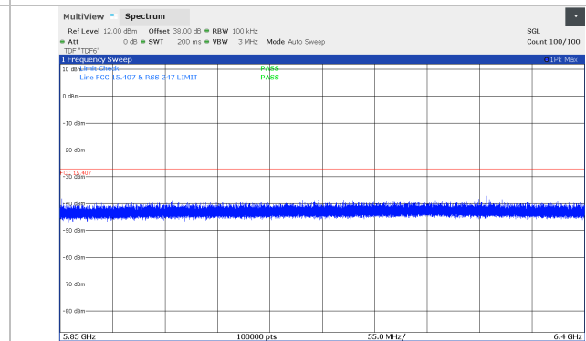
Figure 8.5-16: Conducted spurious emissions 5.850 – 6.4 GHz, 10 MHz Channel BW, Middle channel (5741 MHz), SB1 Band, *100 kHz RBW
