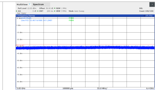
Figure 8.5-98: Conducted spurious emissions 5.850 – 6.4 GHz, 30 MHz Channel BW, Middle channel (5804 MHz), SB1P Band
