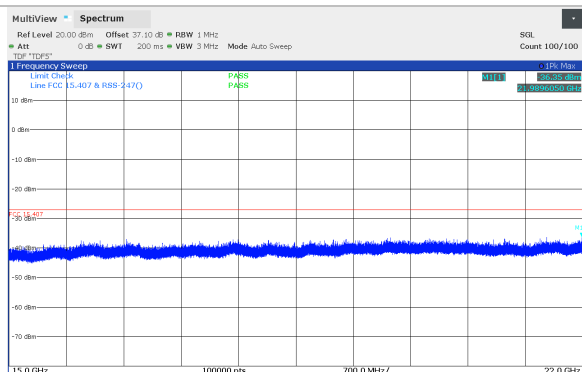
Figure 8.5-111: Conducted spurious emissions 15 - 22 GHz, 10 MHz Channel BW, High channel (5814 MHz), SB1P Band
