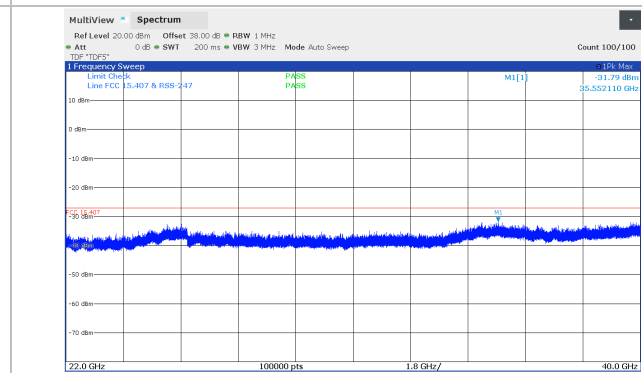
Figure 8.5-102: Conducted spurious emissions 22 - 40 GHz, 30 MHz Channel BW, Middle channel (5804 MHz), SB1P Band
