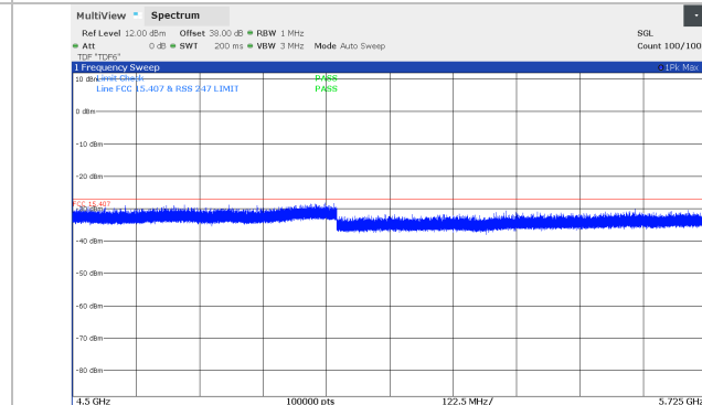
Figure 8.5-96: Conducted spurious emissions 4.5 - 5.725 GHz, 30 MHz Channel BW, Middle channel (5804 MHz), SB1P Band
