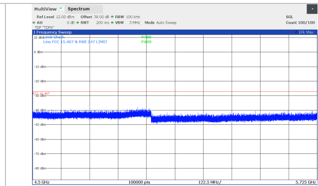
Figure 8.5-14: Conducted spurious emissions 4.5 – 5.725 GHz, 10 MHz Channel BW, Middle channel (5741 MHz), SB1 Band, *100 kHz RBW
