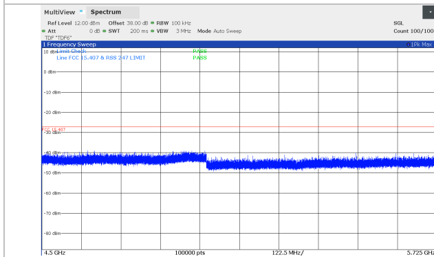
Figure 8.5-117: Conducted spurious emissions 4.5 – 5.725 GHz, 10 MHz Channel BW, Low channel (5824 MHz), SB2P Band, *100 kHz RBW
