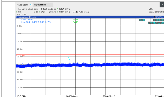
Figure 8.5-131: Conducted spurious emissions 15 - 22 GHz, 10 MHz Channel BW, Middle channel (5834 MHz), SB2P Band
