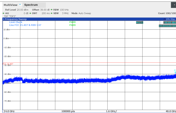
Figure 8.5-55: Conducted spurious emissions 24 - 40 GHz, 10 MHz Channel BW, Middle channel (5771 MHz), SB2 Band, *100 kHz RBW
