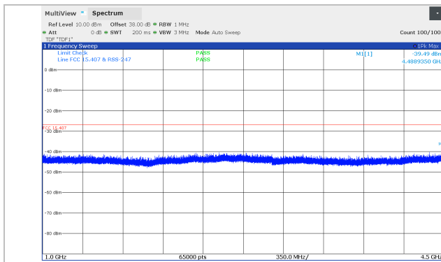
Figure 8.5-115: Conducted spurious emissions 1 – 4.5 GHz, 10 MHz Channel BW, Low channel (5824 MHz), SB2P Band
