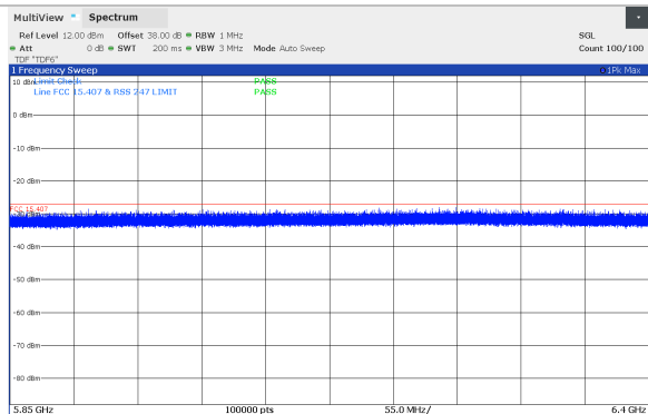
Figure 8.5-33: Conducted spurious emissions 5.850 – 6.4 GHz, 10 MHz Channel BW, High channel (5751 MHz), SB1 Band
