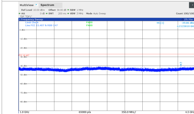
Figure 8.5-135: Conducted spurious emissions 1 – 4.5 GHz, 30 MHz Channel BW, Middle channel (5834 MHz), SB2P Band
