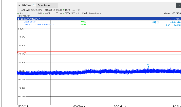
Figure 8.5-47: Conducted spurious emissions 0.03 - 1 GHz, 10 MHz Channel BW, Middle channel (5771 MHz), SB2 Band
