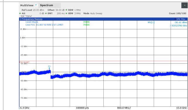
Figure 8.5-120: Conducted spurious emissions 6.4 – 15 GHz, 10 MHz Channel BW, Low channel (5824 MHz), SB2P Band
