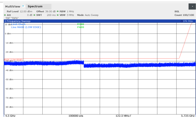
Figure 8.5-146: Conducted spurious emissions 4.5 – 5.725 GHz, 10 MHz Channel BW, High channel (5844 MHz), SB2P Band
