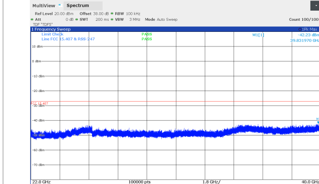
Figure 8.5-93: Conducted spurious emissions 22 - 40 GHz, 10 MHz Channel BW, Middle channel (5804 MHz), SB1P Band, *100 kHz RBW
