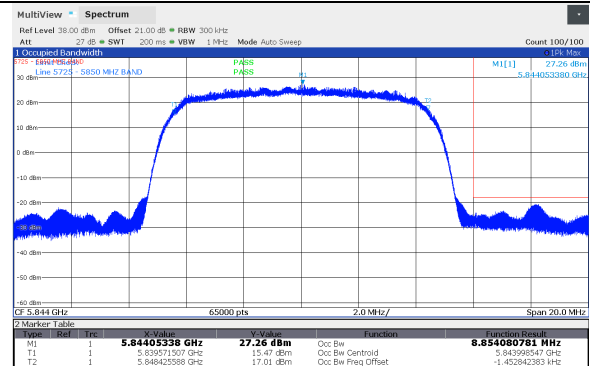
Figure 8.6-34: Frequency stability, 99% OBW, 10 MHz Channel BW, Highest channel (5844 MHz), SB2P Band (+50°C; -48 VDC)
