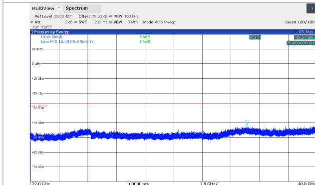
Figure 8.5-83: Conducted spurious emissions 22 - 40 GHz, 10 MHz Channel BW, Low channel (5794 MHz), SB1P Band, *100 kHz RBW
