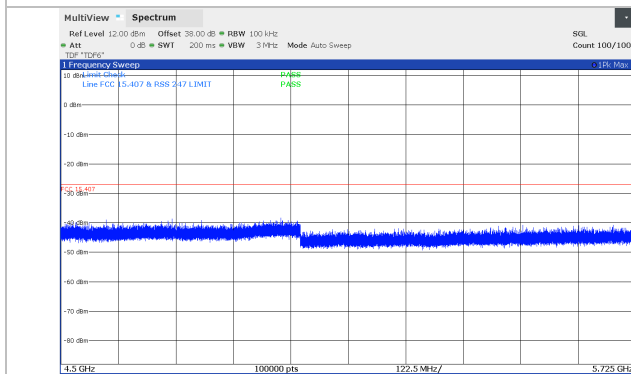
Figure 8.5-87: Conducted spurious emissions 4.5 – 5.725 GHz, 10 MHz Channel BW, Middle channel (5804 MHz), SB1P Band, *100 kHz RBW
