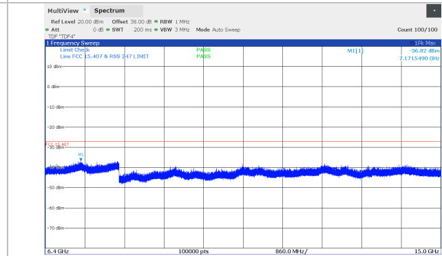
Figure 8.5-100: Conducted spurious emissions 6.4 – 15 GHz, 30 MHz Channel BW, Middle channel (5804 MHz), SB1P Band
