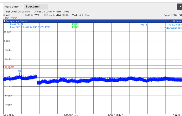
Figure 8.5-110: Conducted spurious emissions 6.4 - 15 GHz, 10 MHz Channel BW, High channel (5814 MHz), SB1P Band
