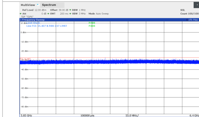
Figure 8.5-51: Conducted spurious emissions 5.850 – 6.4 GHz, 10 MHz Channel BW, Middle channel (5771 MHz), SB2 Band
