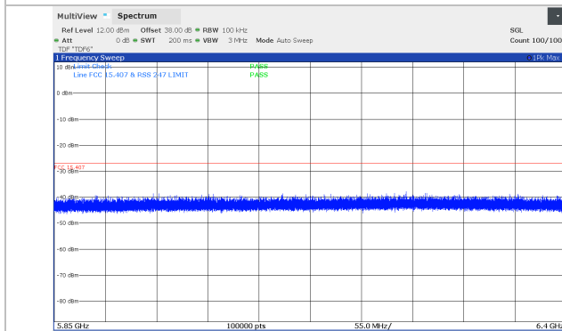
Figure 8.5-129: Conducted spurious emissions 5.850 – 6.4 GHz, 10 MHz Channel BW, Middle channel (5834 MHz), SB2P Band, *100 kHz RBW
