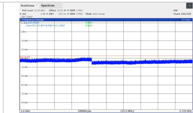
Figure 8.5-86: Conducted spurious emissions 4.5 – 5.725 GHz, 10 MHz Channel BW, Middle channel (5804 MHz), SB1P Band
