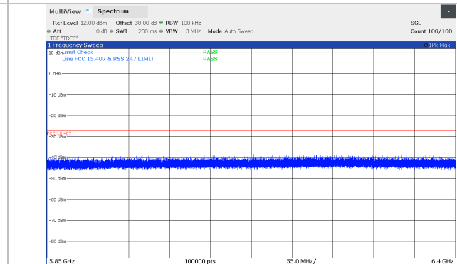
Figure 8.5-52: Conducted spurious emissions 5.850 – 6.4 GHz, 10 MHz Channel BW, Middle channel (5771 MHz), SB2 Band, *100 kHz RBW
