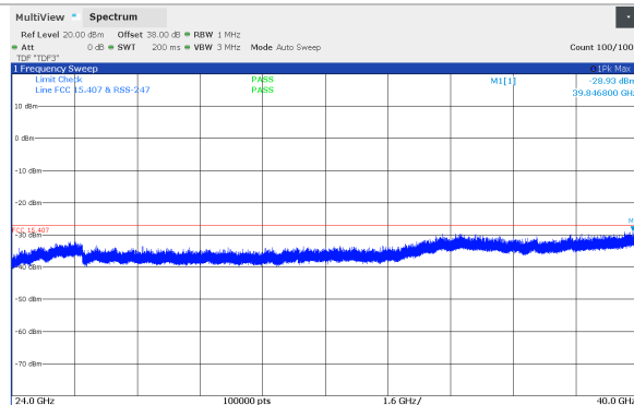
Figure 8.5-36: Conducted spurious emissions 24 - 40 GHz, 10 MHz Channel BW, High channel (5751 MHz), SB1 Band
