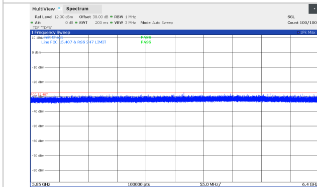
Figure 8.5-15: Conducted spurious emissions 5.850 – 6.4 GHz, 10 MHz Channel BW, Middle channel (5741 MHz), SB1 Band
