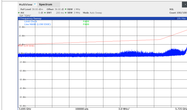
Figure 8.5-5: Conducted spurious emissions 5.695 – 5.725 GHz, 10 MHz Channel BW, Low channel (5731 MHz), SB1 Band
