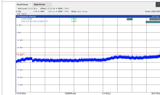
Figure 8.5-63: Conducted spurious emissions 24 - 40 GHz, 30 MHz Channel BW, Middle channel (5771 MHz), SB2 Band
