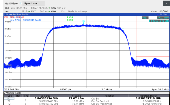
Figure 8.6-26: Frequency stability, 99% OBW, 10 MHz Channel BW, Highest channel (5844 MHz), SB2P Band (-30°C; -48 VDC)
