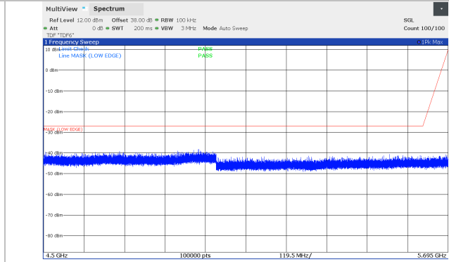
Figure 8.5-4: Conducted spurious emissions 4.5 – 5.695 GHz, 10 MHz Channel BW, Low channel (5731 MHz), SB1 Band, *100 kHz RBW
