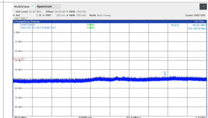
Figure 8.5-144: Conducted spurious emissions 0.03 - 1 GHz, 10 MHz Channel BW, High channel (5844 MHz), SB2P Band
