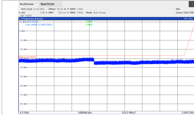
Figure 8.5-3: Conducted spurious emissions 4.5 – 5.695 GHz, 10 MHz Channel BW, Low channel (5731 MHz), SB1 Band
