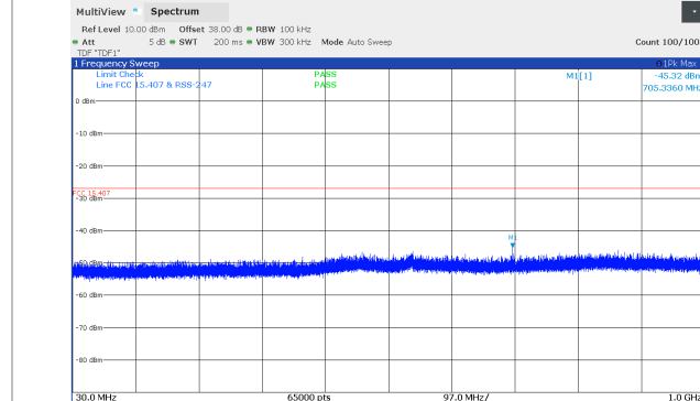
Figure 8.5-94: Conducted spurious emissions 0.03 - 1 GHz, 30 MHz Channel BW, Middle channel (5804 MHz), SB1P Band
