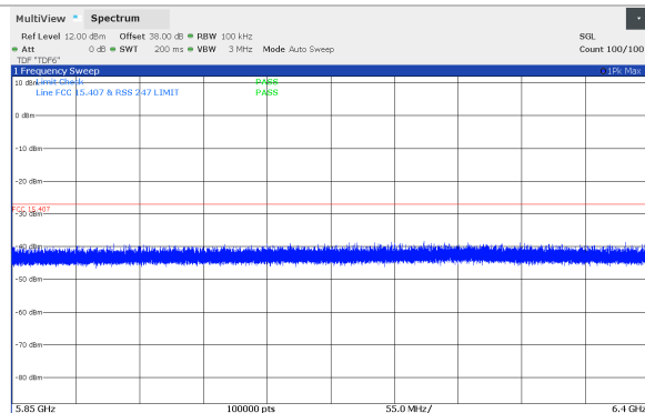
Figure 8.5-34: Conducted spurious emissions 5.850 – 6.4 GHz, 10 MHz Channel BW, High channel (5751 MHz), SB1 Band, *100 kHz RBW
