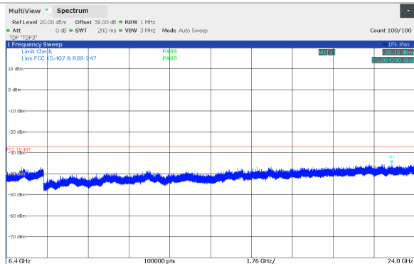
Figure 8.5-35: Conducted spurious emissions 6.4 - 24 GHz, 10 MHz Channel BW, High channel (5751 MHz), SB1 Band
