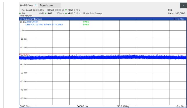
Figure 8.5-128: Conducted spurious emissions 5.850 – 6.4 GHz, 10 MHz Channel BW, Middle channel (5834 MHz), SB2P Band
