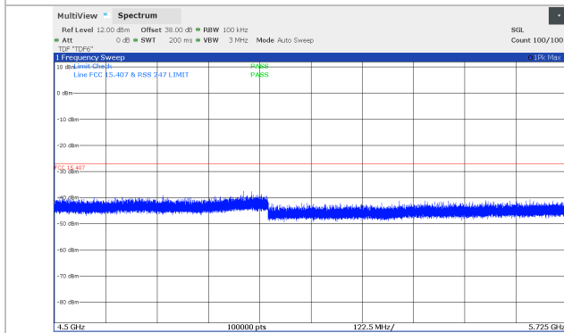
Figure 8.5-137: Conducted spurious emissions 4.5 – 5.725 GHz, 30 MHz Channel BW, Middle channel (5834 MHz), SB2P Band, *100 kHz RBW
