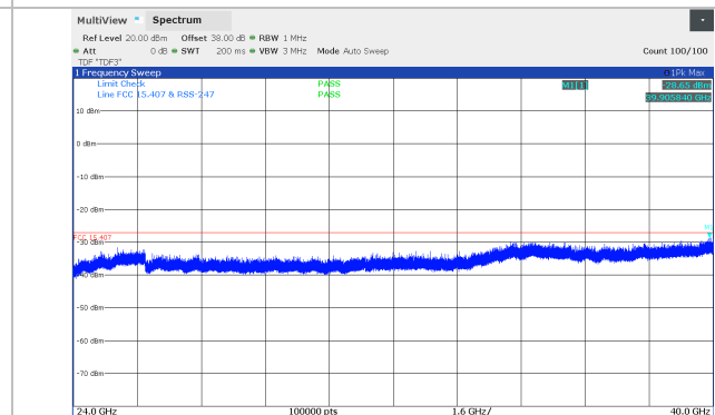
Figure 8.5-18: Conducted spurious emissions 24 - 40 GHz, 10 MHz Channel BW, Middle channel (5741 MHz), SB1 Band
