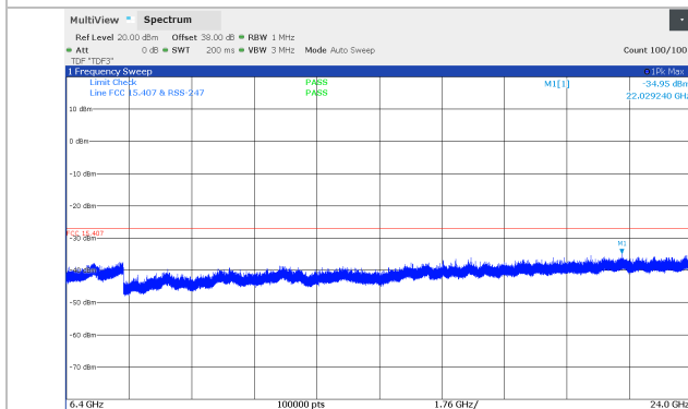
Figure 8.5-71: Conducted spurious emissions 6.4 - 24 GHz, 10 MHz Channel BW, High channel (5781 MHz), SB2 Band
