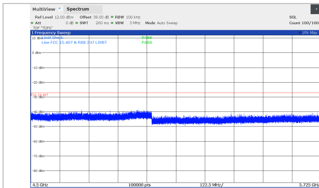
Figure 8.5-127: Conducted spurious emissions 4.5 – 5.725 GHz, 10 MHz Channel BW, Middle channel (5834 MHz), SB2P Band, *100 kHz RBW
