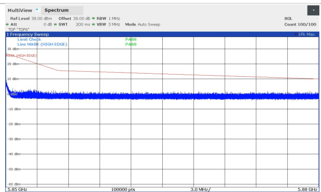
Figure 8.5-148: Conducted spurious emissions 5.850 – 5.880 GHz, 10 MHz Channel BW, High channel (5844 MHz), SB2P Band
