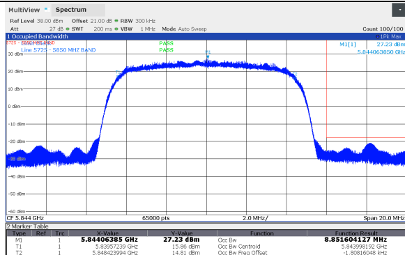
Figure 8.6-33: Frequency stability, 99% OBW, 10 MHz Channel BW, Highest channel (5844 MHz), SB2P Band (+40°C; -48 VDC)
