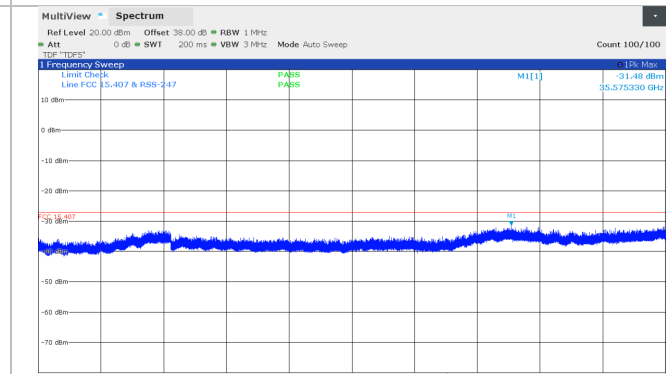
Figure 8.5-142: Conducted spurious emissions 22 - 40 GHz, 30 MHz Channel BW, Middle channel (5834 MHz), SB2P Band
