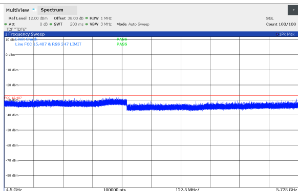
Figure 8.5-31: Conducted spurious emissions 4.5 – 5.725 GHz, 10 MHz Channel BW, High channel (5751 MHz), SB1 Band
