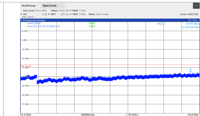
Figure 8.5-8: Conducted spurious emissions 6.4 - 24 GHz, 10 MHz Channel BW, Low channel (5731 MHz), SB1 Band
