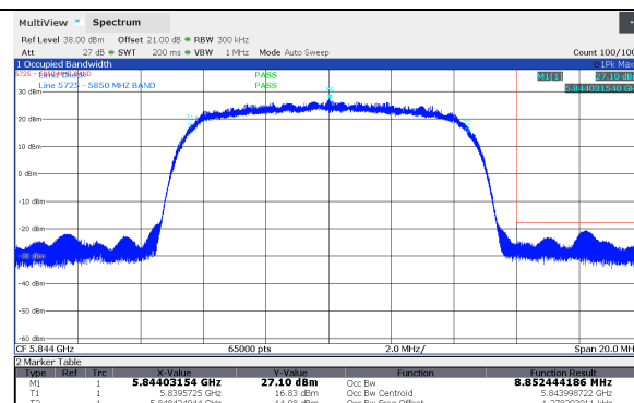
Figure 8.6-38: Frequency stability, 99% OBW, 10 MHz Channel BW, Highest channel (5844 MHz), SB2P Band (+50°C; -55.2 VDC)
