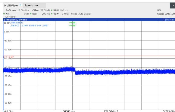
Figure 8.5-32: Conducted spurious emissions 4.5 – 5.725 GHz, 10 MHz Channel BW, High channel (5751 MHz), SB1 Band, *100 kHz RBW
