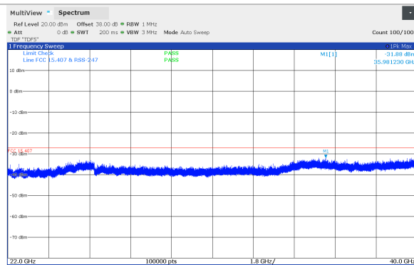
Figure 8.5-112: Conducted spurious emissions 22 - 40GHz, 10 MHz Channel BW, High channel (5814 MHz), SB1P Band
