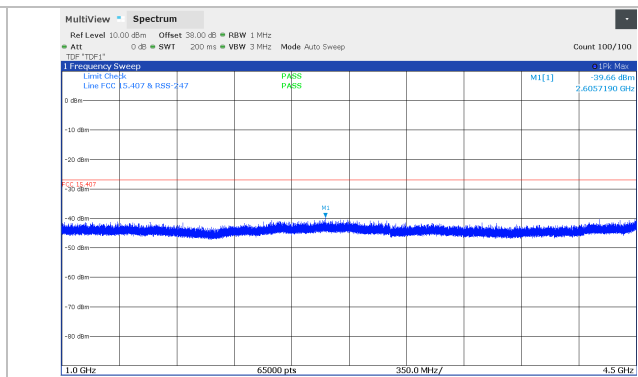
Figure 8.5-2: Conducted spurious emissions 1 – 4.5 GHz, 10 MHz Channel BW, Low channel (5731 MHz), SB1 Band
