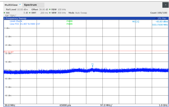
Figure 8.5-74: Conducted spurious emissions 0.03 - 1 GHz, 10 MHz Channel BW, Low channel (5794 MHz), SB1P Band
