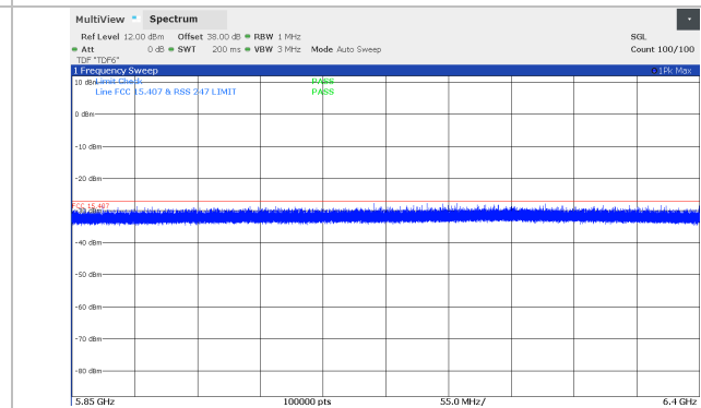
Figure 8.5-118: Conducted spurious emissions 5.850 – 6.4 GHz, 10 MHz Channel BW, Low channel (5824 MHz), SB2P Band
