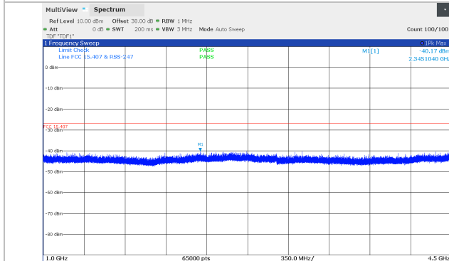
Figure 8.5-95: Conducted spurious emissions 1 - 4.5 GHz, 30 MHz Channel BW, Middle channel (5804 MHz), SB1P Band
