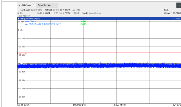
Figure 8.5-119: Conducted spurious emissions 5.850 – 6.4 GHz, 10 MHz Channel BW, Low channel (5824 MHz), SB2P Band, *100 kHz RBW
