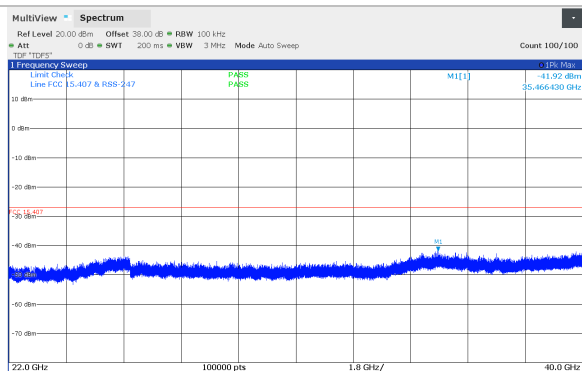
Figure 8.5-113: Conducted spurious emissions 22 - 40GHz, 10 MHz Channel BW, High channel (5814 MHz), SB1P Band, *100 kHz RBW
