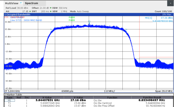
Figure 8.6-32: Frequency stability, 99% OBW, 10 MHz Channel BW, Highest channel (5844 MHz), SB2P Band (+30°C; -48 VDC)
