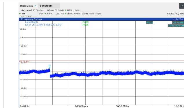
Figure 8.5-140: Conducted spurious emissions 6.4 - 15 GHz, 30 MHz Channel BW, Middle channel (5834 MHz), SB2P Band
