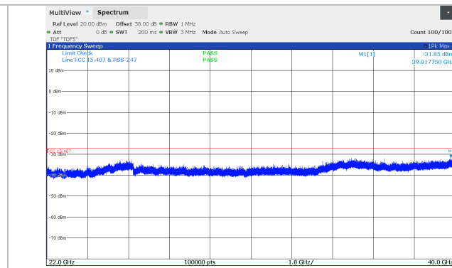
Figure 8.5-92: Conducted spurious emissions 22 - 40 GHz, 10 MHz Channel BW, Middle channel (5804 MHz), SB1P Band
