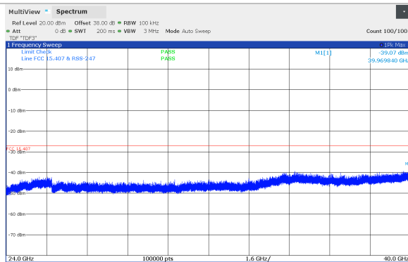
Figure 8.5-19: Conducted spurious emissions 24 - 40 GHz, 10 MHz Channel BW, Middle channel (5741 MHz), SB1 Band, *100 kHz RBW
