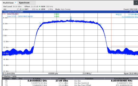
Figure 8.6-31: Frequency stability, 99% OBW, 10 MHz Channel BW, Highest channel (5844 MHz), SB1 Band (+20°C; -48 VDC)
