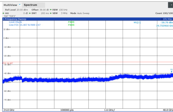
Figure 8.5-73: Conducted spurious emissions 24 - 40 GHz, 10 MHz Channel BW, High channel (5781 MHz), SB2 Band, *100 kHz RBW
