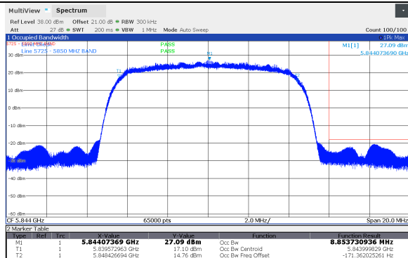
Figure 8.6-29: Frequency stability, 99% OBW, 10 MHz Channel BW, Highest channel (5844 MHz), SB1 Band (0°C; -48 VDC)
