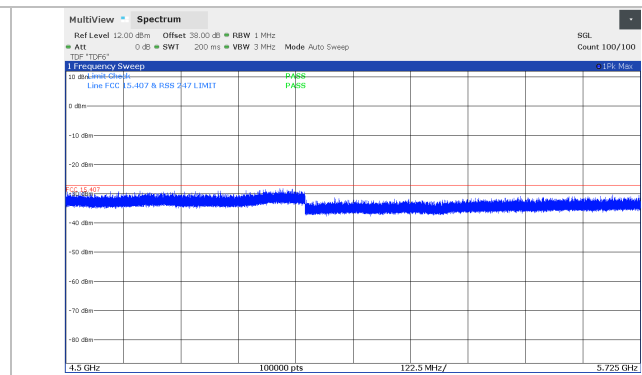
Figure 8.5-116: Conducted spurious emissions 4.5 – 5.725 GHz, 10 MHz Channel BW, Low channel (5824 MHz), SB2P Band
