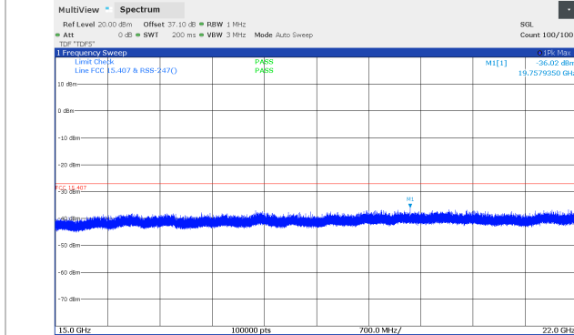
Figure 8.5-81: Conducted spurious emissions 15 - 22 GHz, 10 MHz Channel BW, Low channel (5794 MHz), SB1P Band
