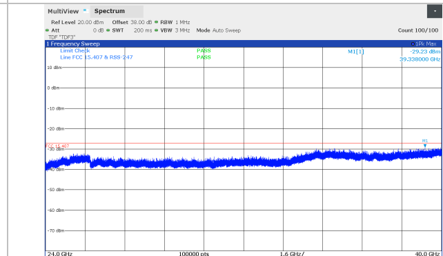
Figure 8.5-54: Conducted spurious emissions 24 - 40 GHz, 10 MHz Channel BW, Middle channel (5771 MHz), SB2 Band
