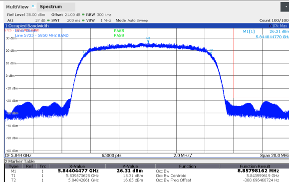
Figure 8.6-27: Frequency stability, 99% OBW, 10 MHz Channel BW, Highest channel (5844 MHz), SB2P Band (-20°C; -48 VDC)
