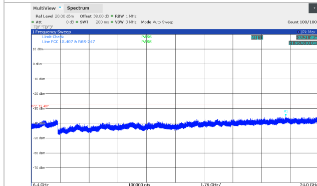
Figure 8.5-53: Conducted spurious emissions 6.4 - 24 GHz, 10 MHz Channel BW, Middle channel (5771 MHz), SB2 Band
