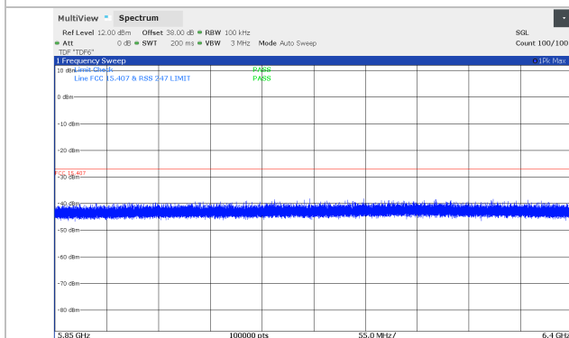
Figure 8.5-89: Conducted spurious emissions 5.850 – 6.4 GHz, 10 MHz Channel BW, Middle channel (5804 MHz), SB1P Band, *100 kHz RBW
