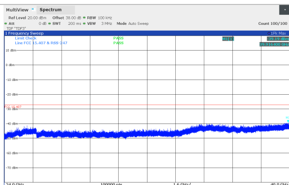
Figure 8.5-37: Conducted spurious emissions 24 - 40 GHz, 10 MHz Channel BW, High channel (5751 MHz), SB1 Band, *100 kHz RBW
