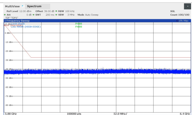
Figure 8.5-150: Conducted spurious emissions 5.880 – 6.4 GHz, 10 MHz Channel BW, High channel (5844 MHz), SB2P Band, *100 kHz RBW
