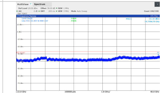
Figure 8.5-132: Conducted spurious emissions 22 - 40 GHz, 10 MHz Channel BW, Middle channel (5834 MHz), SB2P Band
