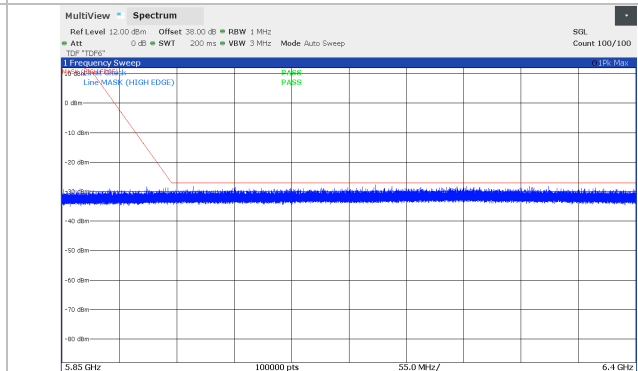
Figure 8.5-6: Conducted spurious emissions 5.850 – 6.4 GHz, 10 MHz Channel BW, Low channel (5731 MHz), SB1 Band
