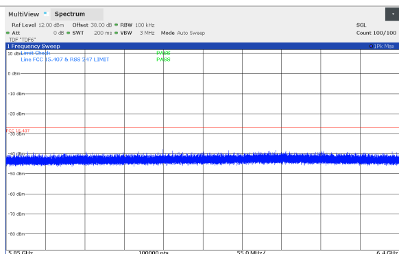
Figure 8.5-109: Conducted spurious emissions 5.850 – 6.4 GHz, 10 MHz Channel BW, High channel (5814 MHz), SB1P Band, *100 kHz RBW
