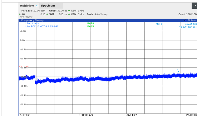
Figure 8.5-17: Conducted spurious emissions 6.4 - 24 GHz, 10 MHz Channel BW, Middle channel (5741 MHz), SB1 Band
