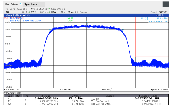
Figure 8.6-30: Frequency stability, 99% OBW, 10 MHz Channel BW, Highest channel (5844 MHz), SB1 Band (+10°C; -48 VDC)
