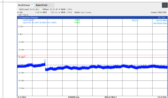
Figure 8.5-90: Conducted spurious emissions 6.4 – 15 GHz, 10 MHz Channel BW, Middle channel (5804 MHz), SB1P Band
