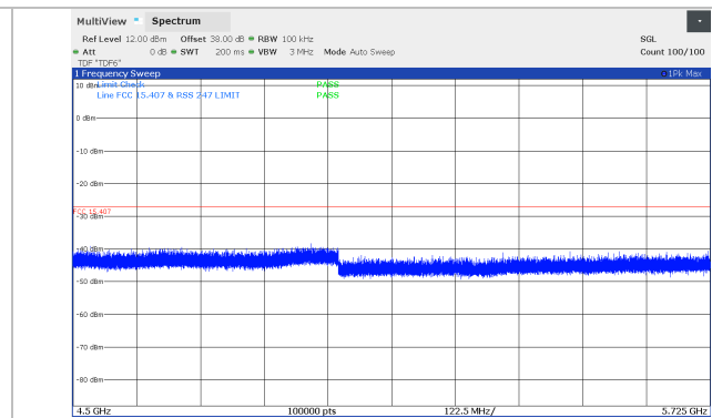
Figure 8.5-50: Conducted spurious emissions 4.5 – 5.725 GHz, 10 MHz Channel BW, Middle channel (5771 MHz), SB2 Band, *100 kHz RBW
