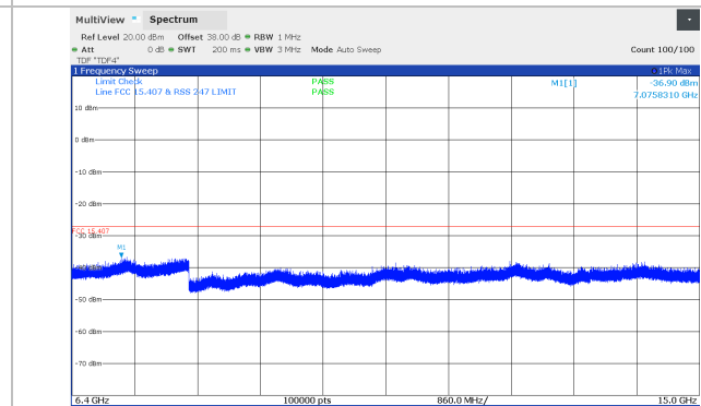
Figure 8.5-130: Conducted spurious emissions 6.4 – 15 GHz, 10 MHz Channel BW, Middle channel (5834 MHz), SB2P Band
