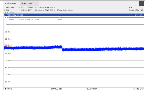
Figure 8.5-106: Conducted spurious emissions 4.5 – 5.725 GHz, 10 MHz Channel BW, High channel (5814 MHz), SB1P Band
