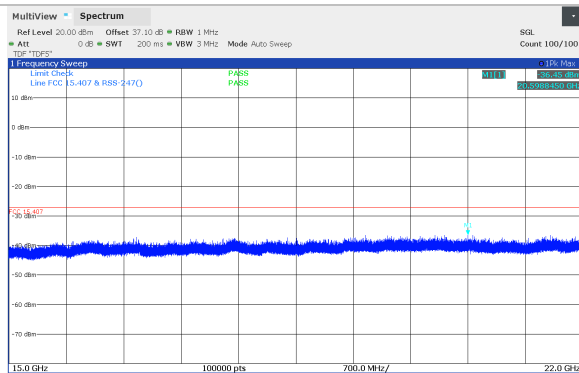
Figure 8.5-121: Conducted spurious emissions 15 - 22 GHz, 10 MHz Channel BW, Low channel (5824 MHz), SB2P Band
