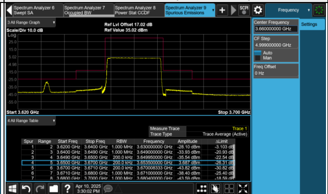
Channel 642502 (3637.53MHz)
