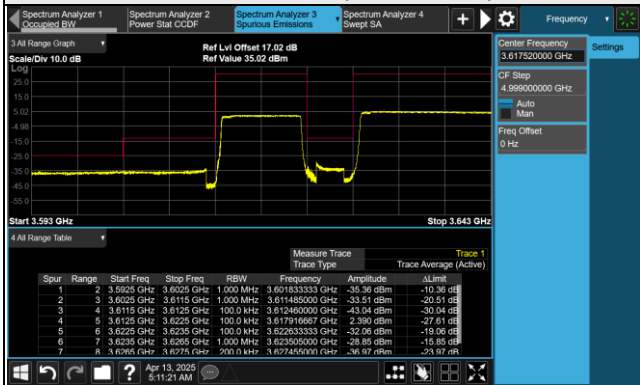
Channel 641168 (3617.52MHz)
