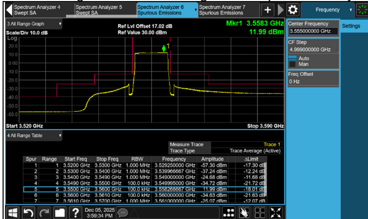
CH 637000 (3555 MHz)
