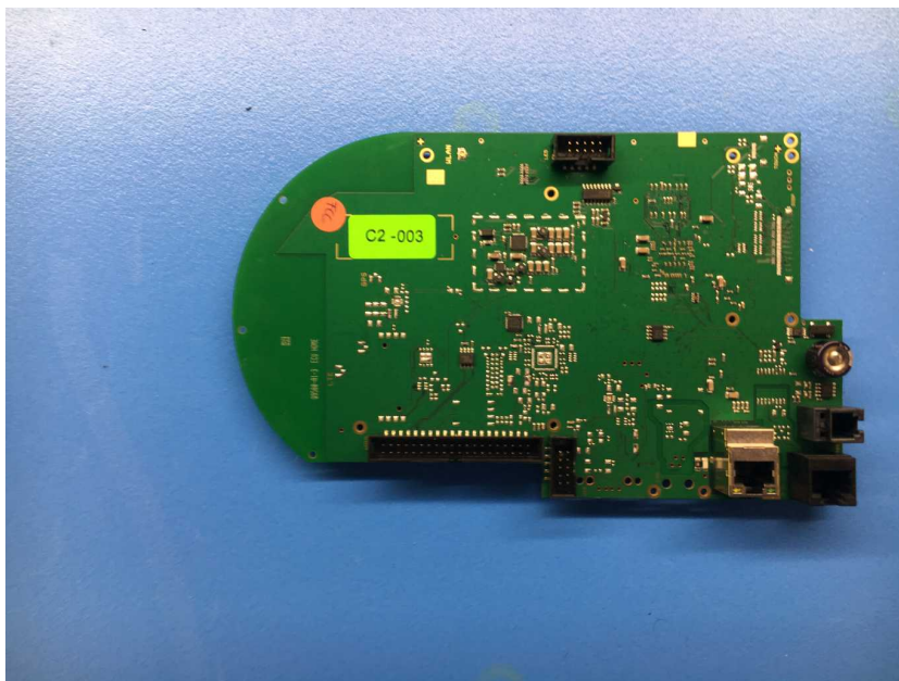
Photo 10: ECU board front side view with shieldings removed
