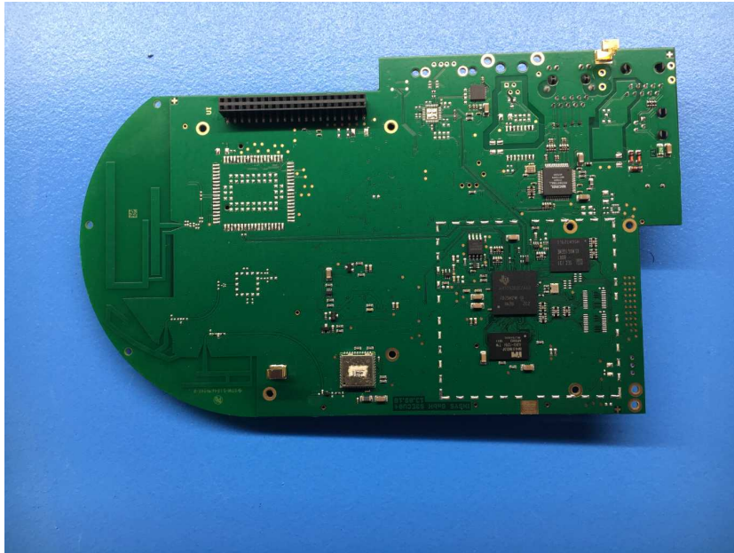
Photo 11: ECU board back side view with shieldings removed
