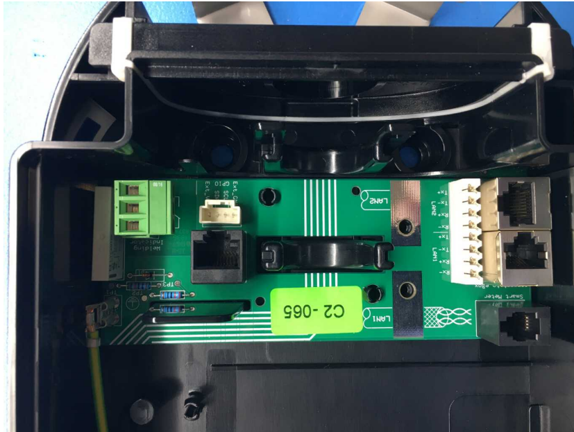
Photo 7: IF board
