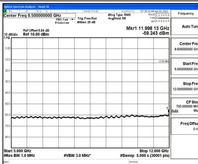
Band26-3MHz-16QAM-26705-1-0-Low-5000-12000--59.24-PASS
