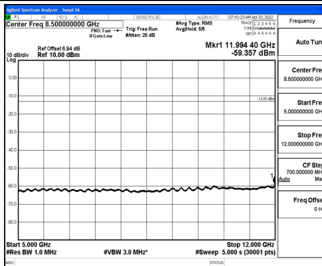
Band26-3MHz-QPSK-26775-1-0-High-5000-12000--59.36-PASS
