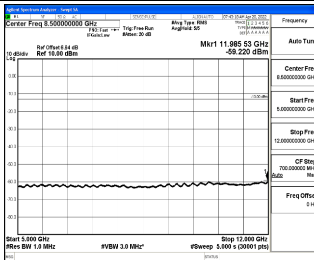
Band26-3MHz-16QAM-26775-1-0-High-5000-12000--59.22-PASS
