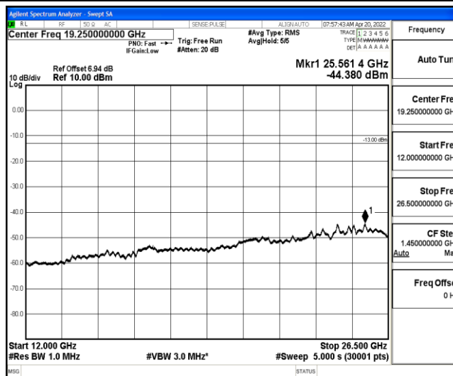
Band26-5MHz-QPSK-26740-1-0-Low-12000-26500--44.38-PASS
