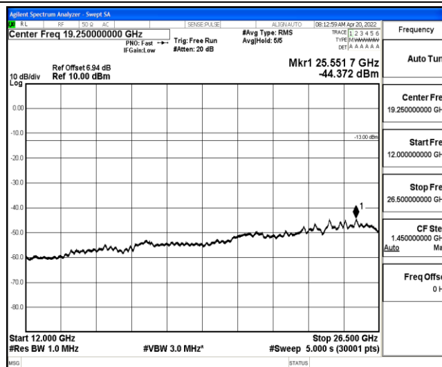
Band26-10MHz-QPSK-26740-1-0-Low-12000-26500--44.37-PASS
