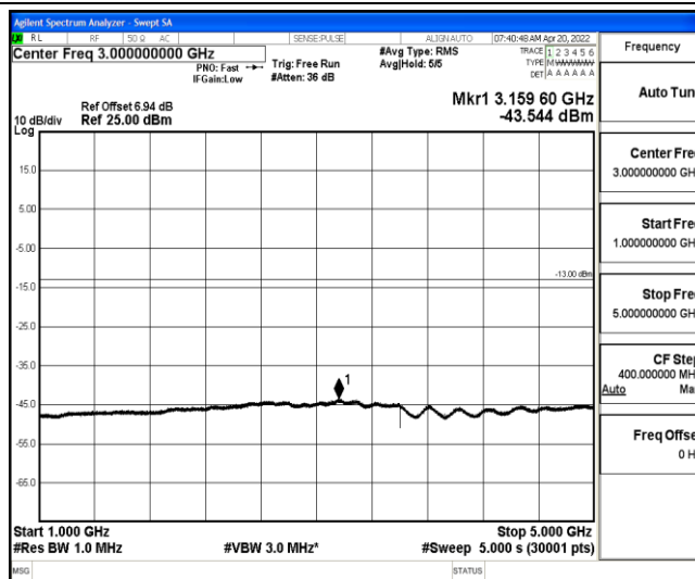
Band26-3MHz-QPSK-26775-1-0-High-1000-5000--43.54-PASS
