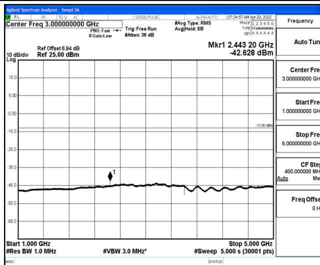
Band26-3MHz-16QAM-26705-1-0-Low-1000-5000--42.63-PASS
