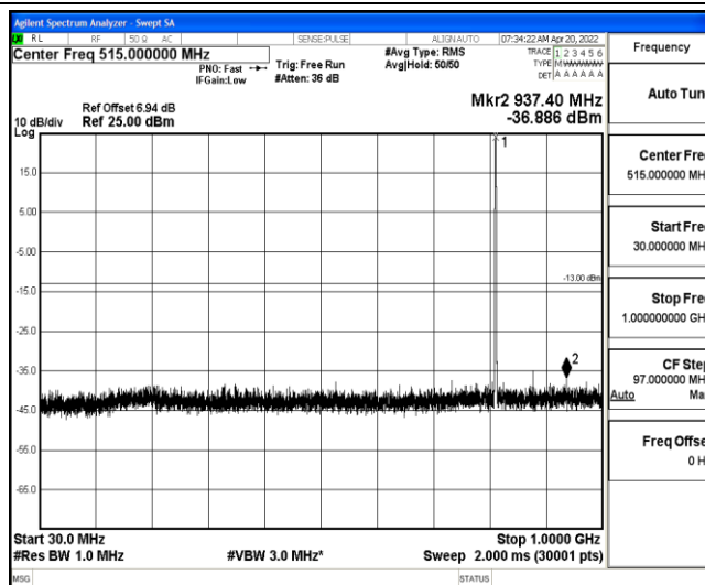
Band26-3MHz-16QAM-26705-1-0-Low-30-1000--36.89-PASS
