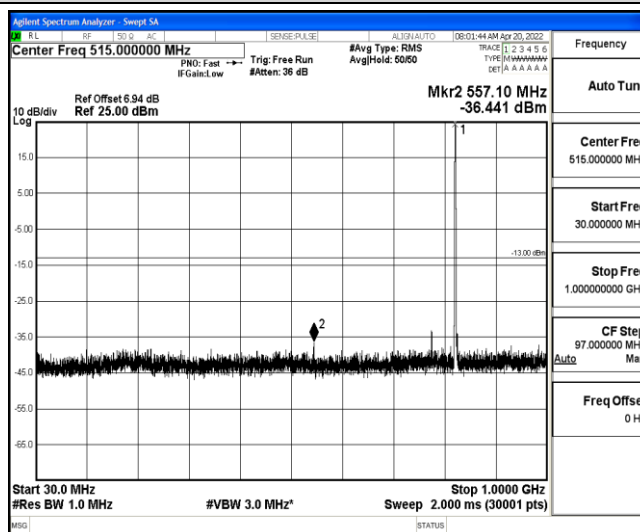
Band26-5MHz-16QAM-26785-1-0-High-30-1000--36.44-PASS
