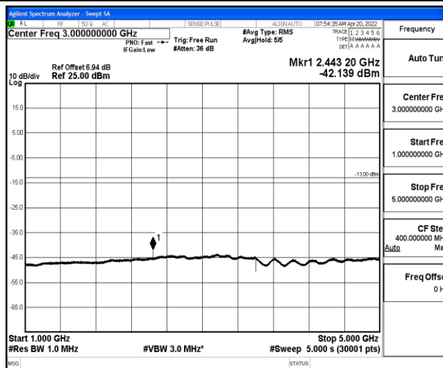
Band26-5MHz-16QAM-26715-1-0-Low-1000-5000--42.14-PASS
