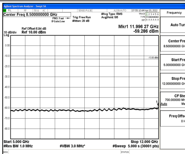
Band26-5MHz-16QAM-26715-1-0-Low-5000-12000--59.29-PASS
