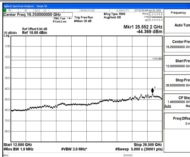
Band26-5MHz-QPSK-26715-1-0-Low-12000-26500--44.37-PASS
