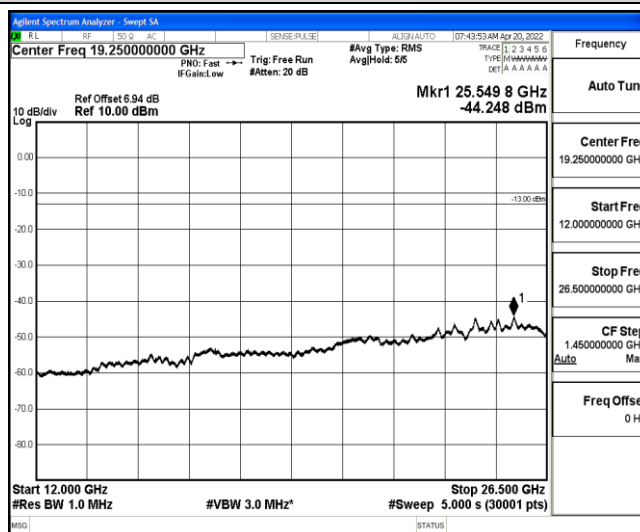
Band26-3MHz-16QAM-26775-1-0-High-12000-26500--44.25-PASS
