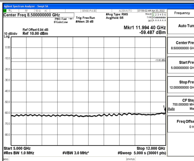
Band26-5MHz-16QAM-26740-1-0-Low-5000-12000--59.49-PASS
