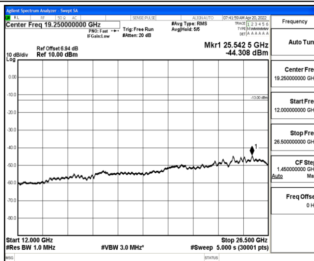
Band26-3MHz-QPSK-26775-1-0-High-12000-26500--44.31-PASS
