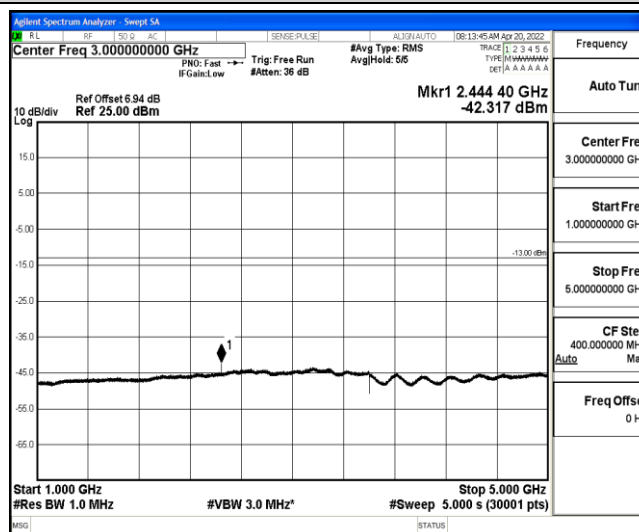
Band26-10MHz-16QAM-26740-1-0-Low-1000-5000--42.32-PASS
