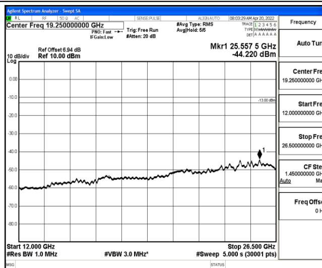
Band26-5MHz-16QAM-26785-1-0-High-12000-26500--44.22-PASS
