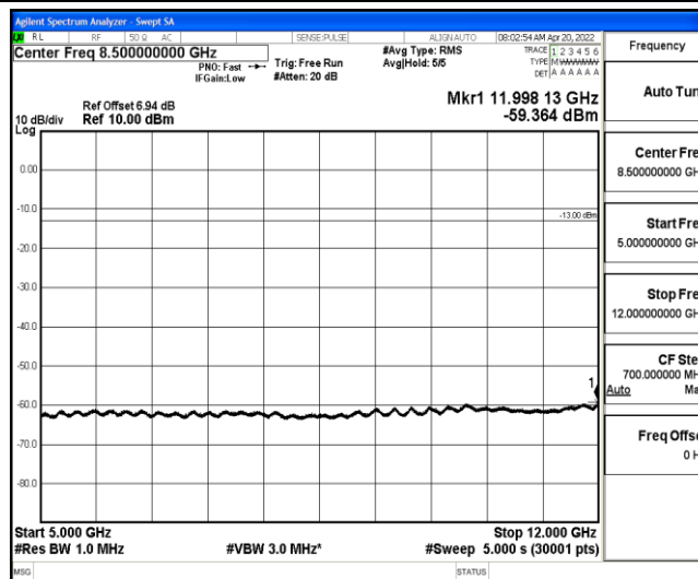
Band26-5MHz-16QAM-26785-1-0-High-5000-12000--59.36-PASS
