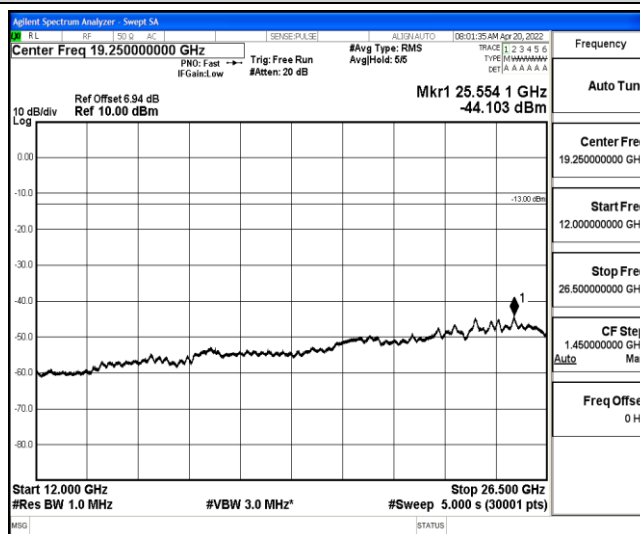
Band26-5MHz-QPSK-26785-1-0-High-12000-26500--44.1-PASS
