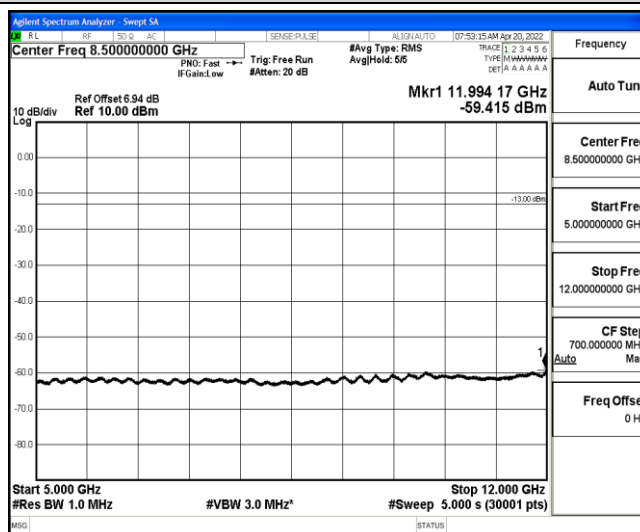
Band26-5MHz-QPSK-26715-1-0-Low-5000-12000--59.42-PASS
