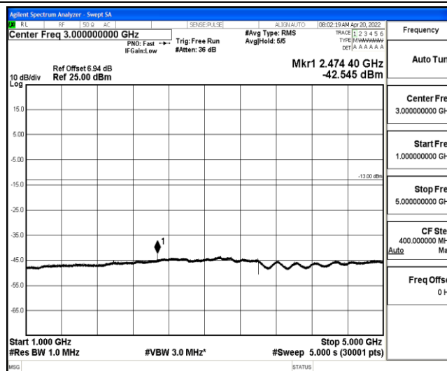
Band26-5MHz-16QAM-26785-1-0-High-1000-5000--42.55-PASS
