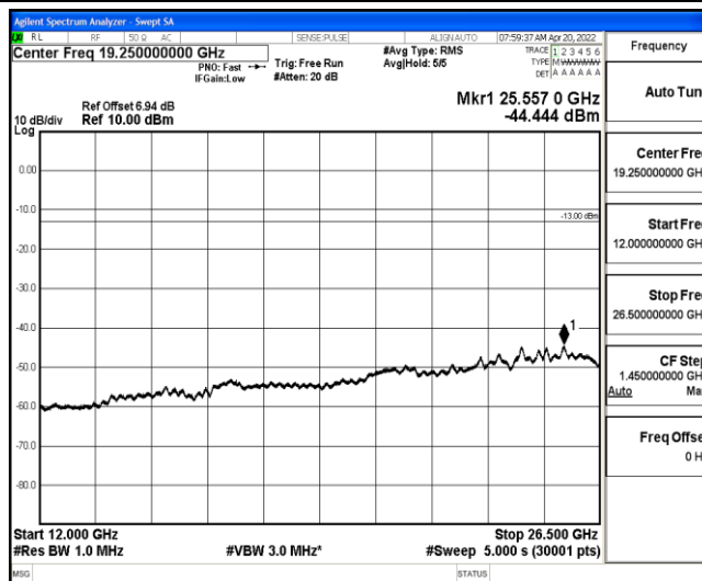
Band26-5MHz-16QAM-26740-1-0-Low-12000-26500--44.44-PASS
