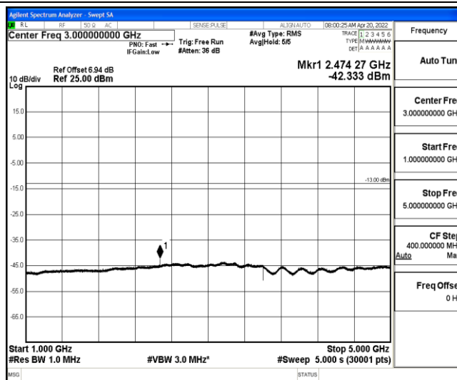
Band26-5MHz-QPSK-26785-1-0-High-1000-5000--42.33-PASS
