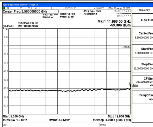
Band26-5MHz-QPSK-26785-1-0-High-5000-12000--59.39-PASS
