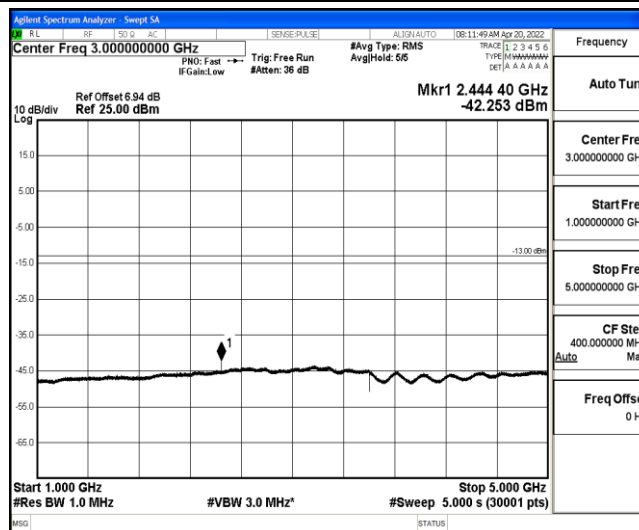
Band26-10MHz-QPSK-26740-1-0-Low-1000-5000--42.25-PASS
