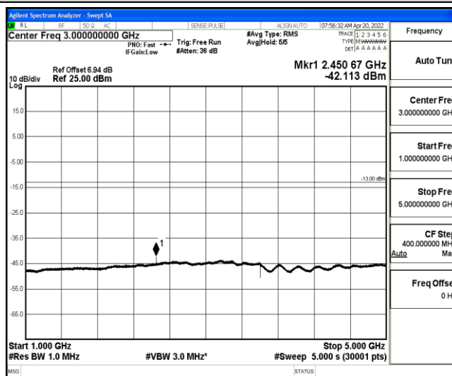
Band26-5MHz-QPSK-26740-1-0-Low-1000-5000--42.11-PASS
