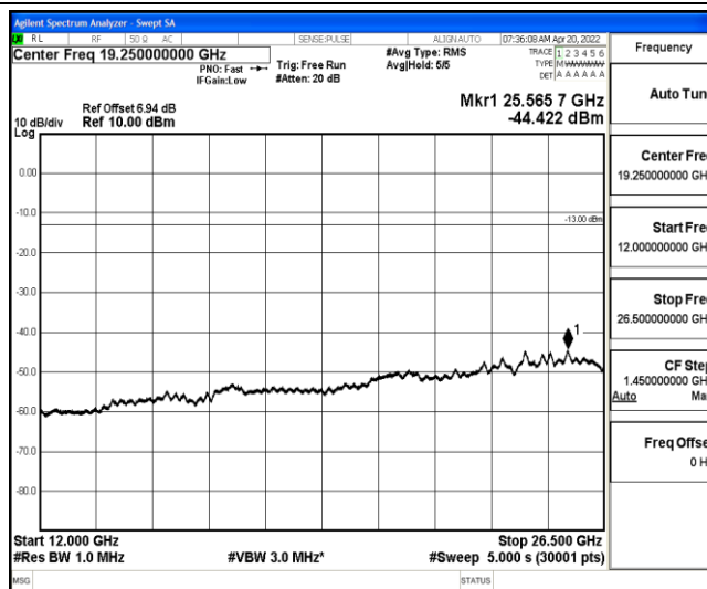
Band26-3MHz-16QAM-26705-1-0-Low-12000-26500--44.42-PASS
