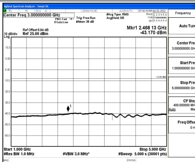
Band26-3MHz-16QAM-26775-1-0-High-1000-5000--43.17-PASS
