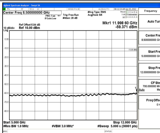
Band26-10MHz-QPSK-26740-1-0-Low-5000-12000--59.37-PASS
