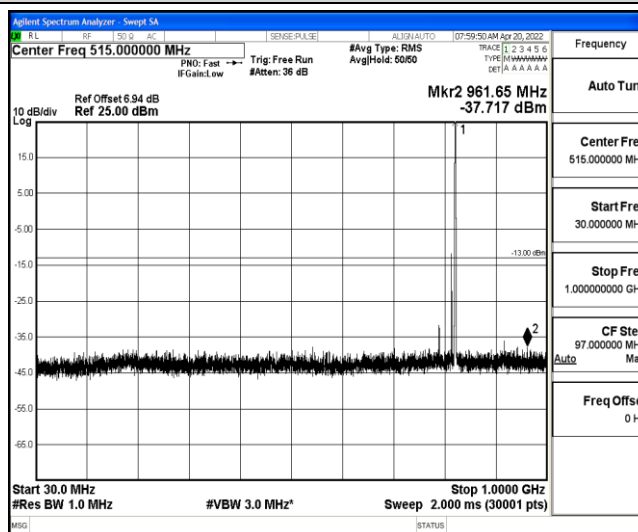
Band26-5MHz-QPSK-26785-1-0-High-30-1000--37.72-PASS
