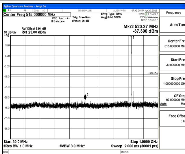
Band26-3MHz-16QAM-26775-1-0-High-30-1000--37.4-PASS
