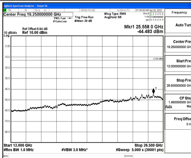
Band26-3MHz-16QAM-26740-1-0-Low-12000-26500--44.48-PASS
