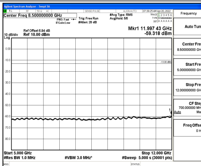
Band26-3MHz-16QAM-26740-1-0-Low-5000-12000--59.32-PASS
