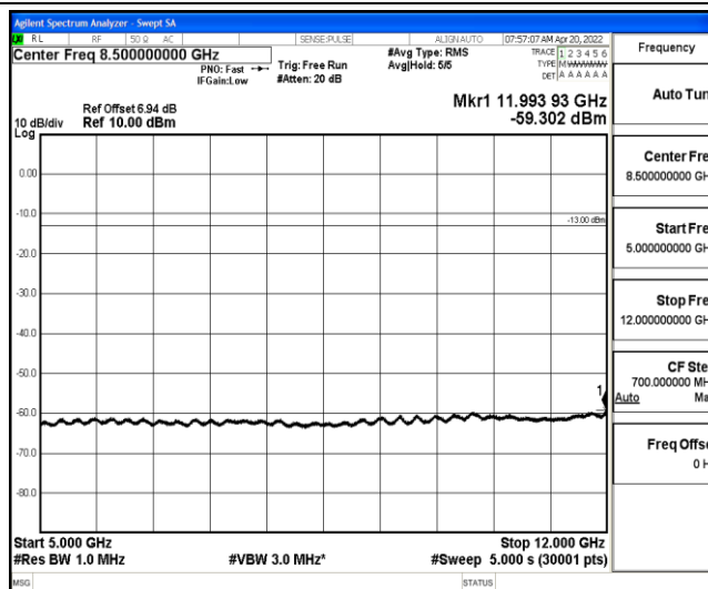
Band26-5MHz-QPSK-26740-1-0-Low-5000-12000--59.3-PASS
