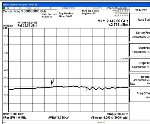
Band26-5MHz-QPSK-26715-1-0-Low-1000-5000--42.74-PASS
