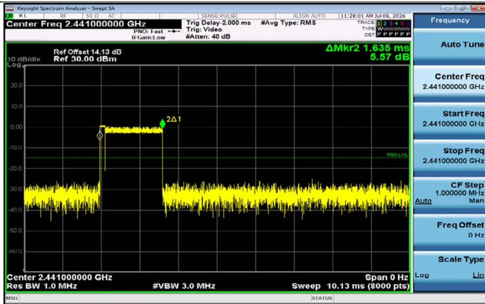
3DH3-Ant1-Hop-PASS
