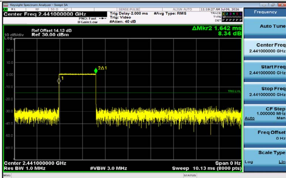
DH3-Ant1-Hop-PASS
