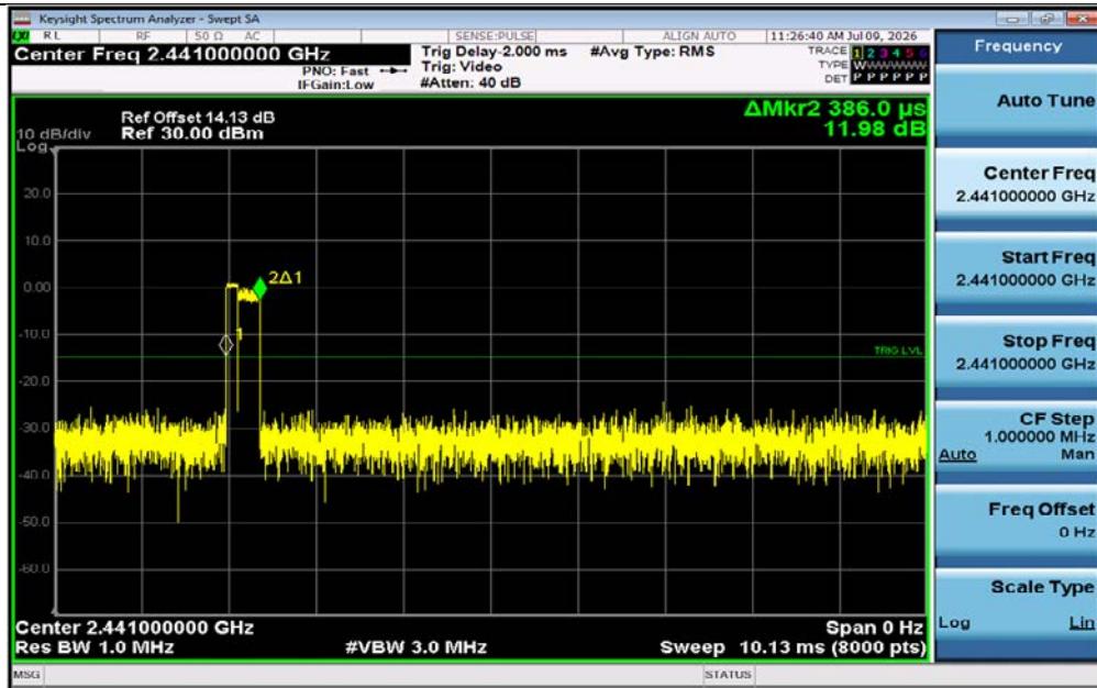
3DH1-Ant1-Hop-PASS
