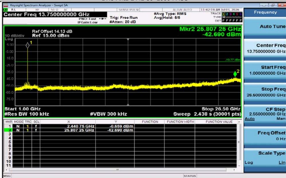
DH5-Ant1-2441-1000~26500-PASS
