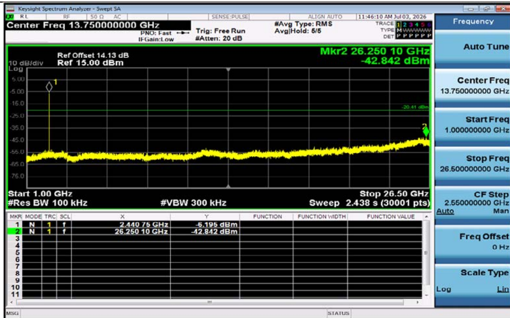
2DH5-Ant1-2441-1000-26500-PASS
