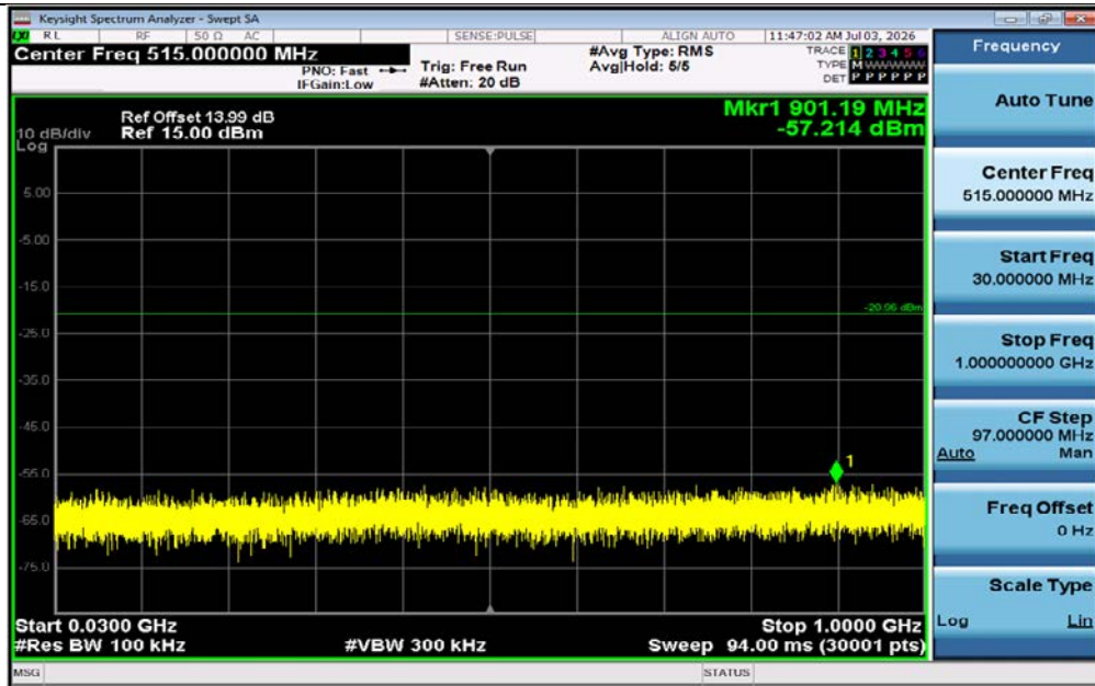
2DH5-Ant1-2480-30~1000-PASS
