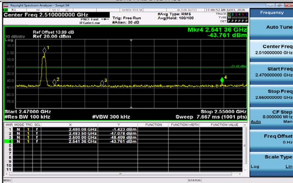
2DH5-Ant1-2480-PASS
