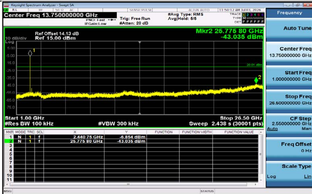
3DH5-Ant1-2441-1000~26500-PASS
