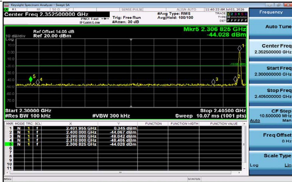
DH5-Ant1-2402-PASS
