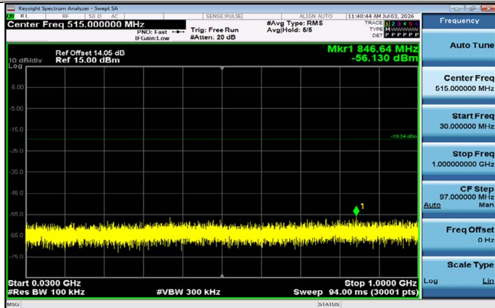
DH5-Ant1-2402-30~1000-PASS
