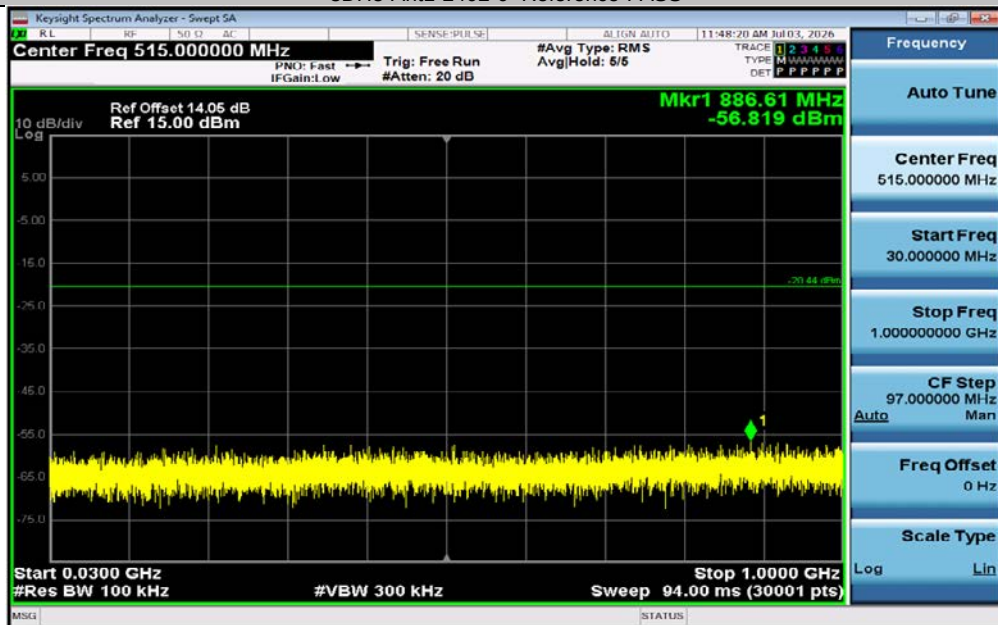
3DH5-Ant1-2402-30~1000-PASS
