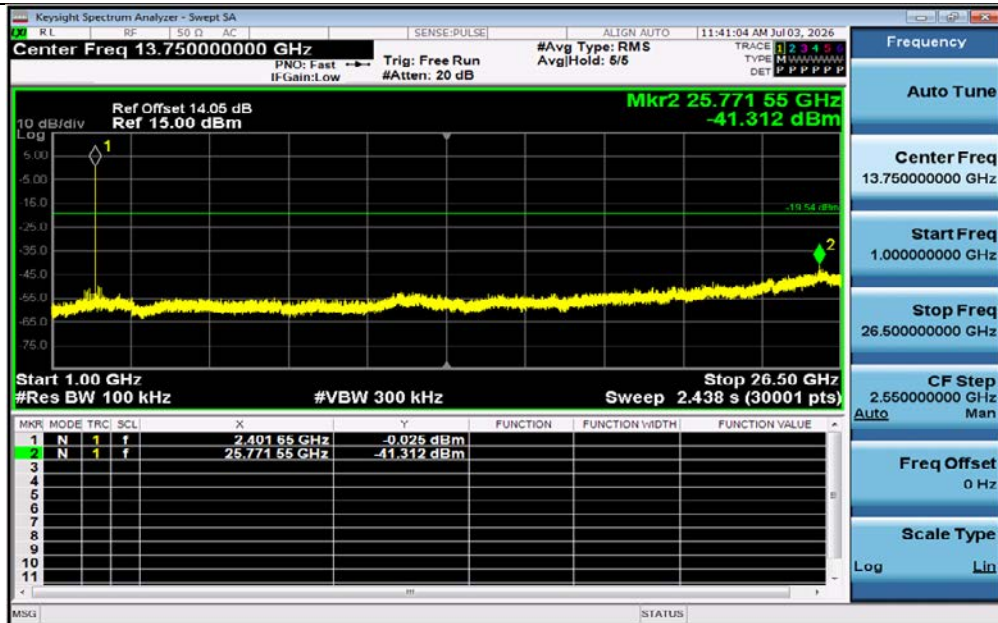
DH5-Ant1-2402-1000~26500-PASS
