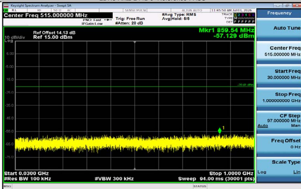
2DH5-Ant1-2441-30~1000-PASS
