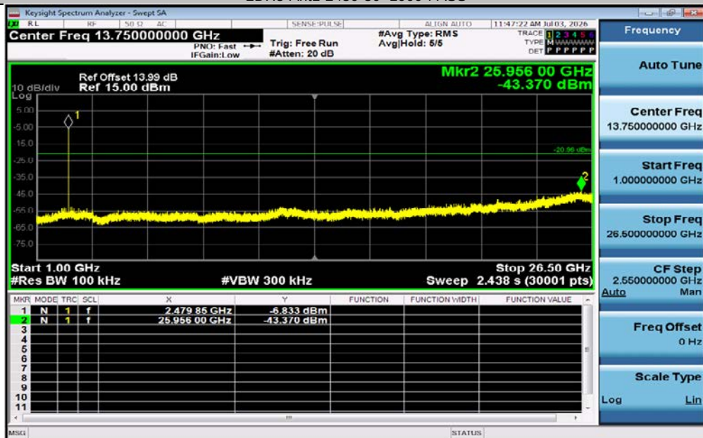
2DH5-Ant1-2480-1000~26500-PASS
