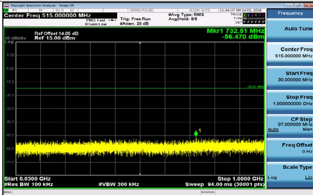
2DH5-Ant1-2402-30~1000-PASS
