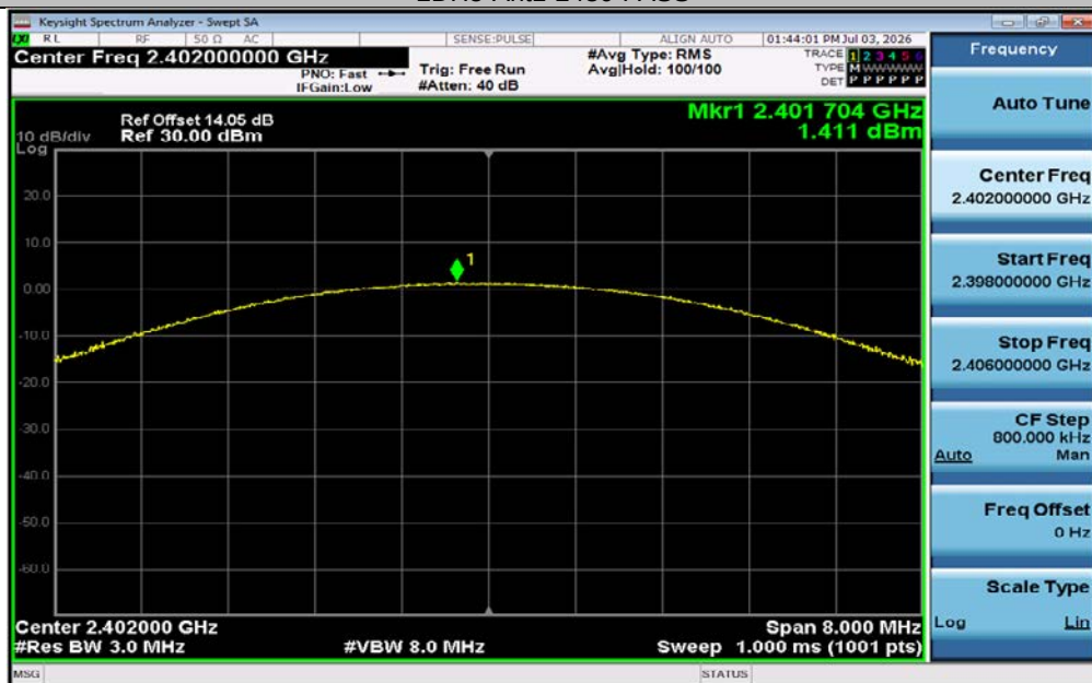
3DH5-Ant1-2402-PASS
