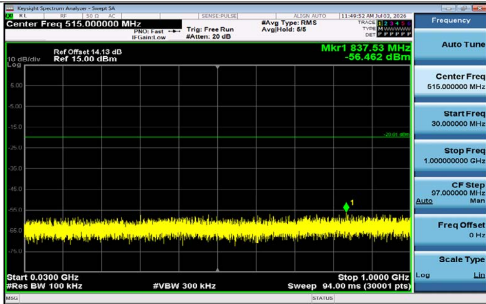
3DH5-Ant1-2441-30~1000-PASS
