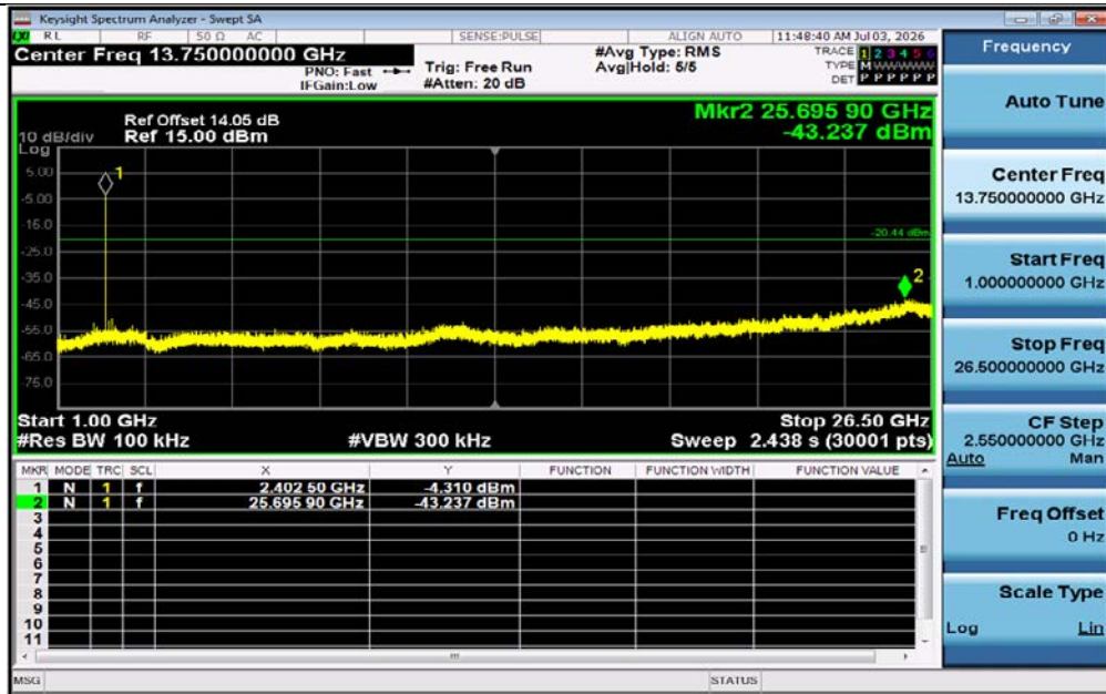
3DH5-Ant1-2402-1000-26500-PASS
