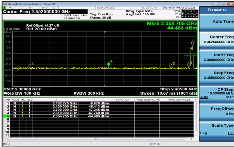
3DH5-Ant1-Hop_2402-PASS
