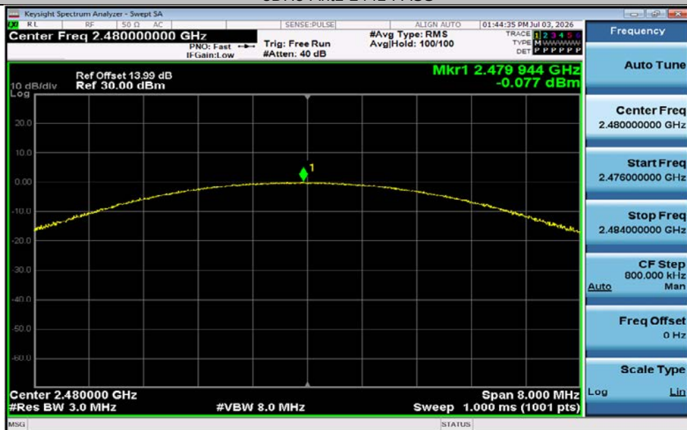
3DH5-Ant1-2480-PASS
