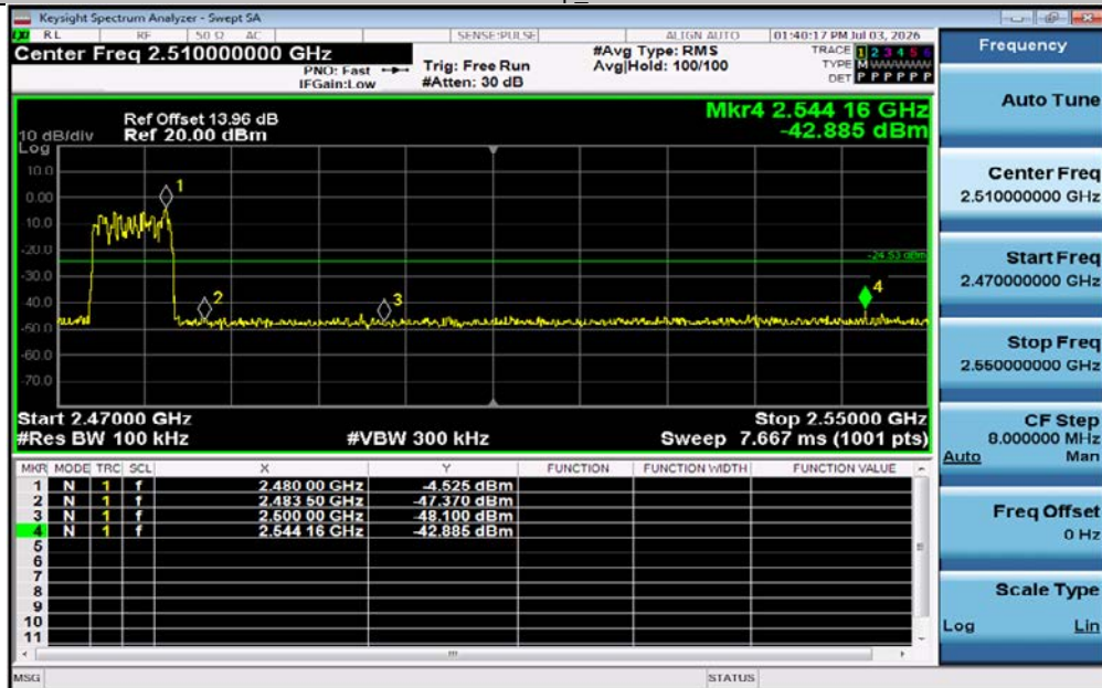
2DH5-Ant1-Hop_2480-PASS
