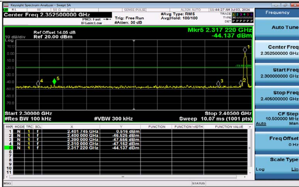
2DH5-Ant1-2402-PASS
