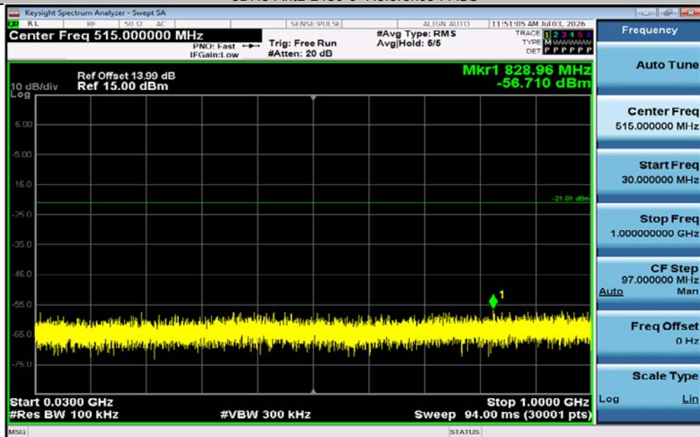
3DH5-Ant1-2480-30~1000-PASS
