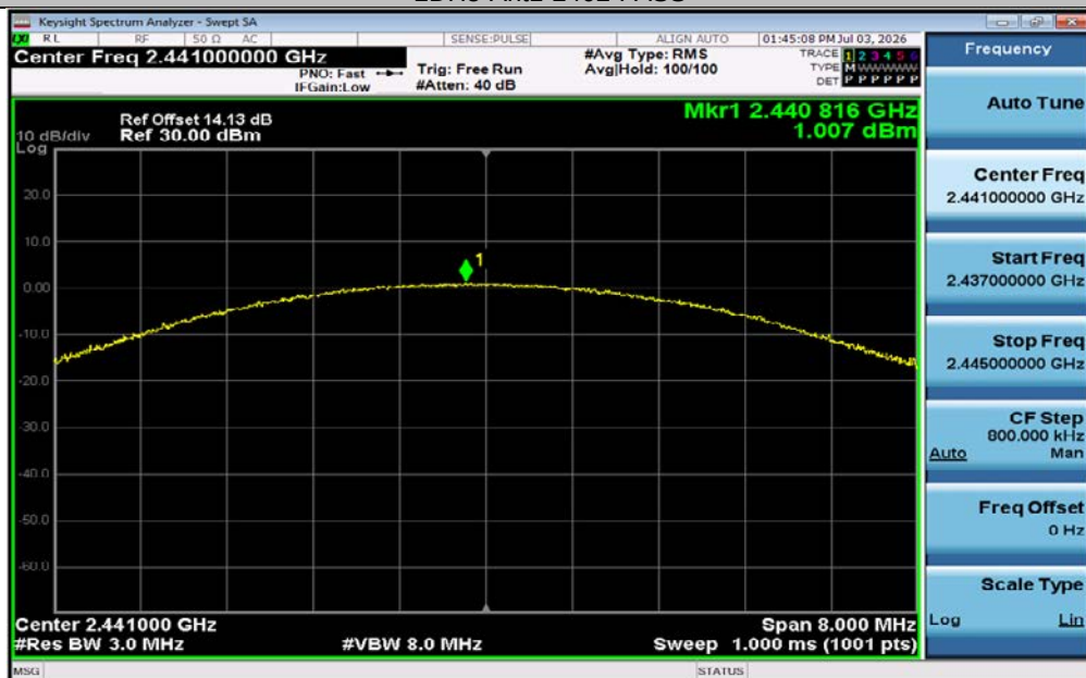
2DH5-Ant1-2441-PASS
