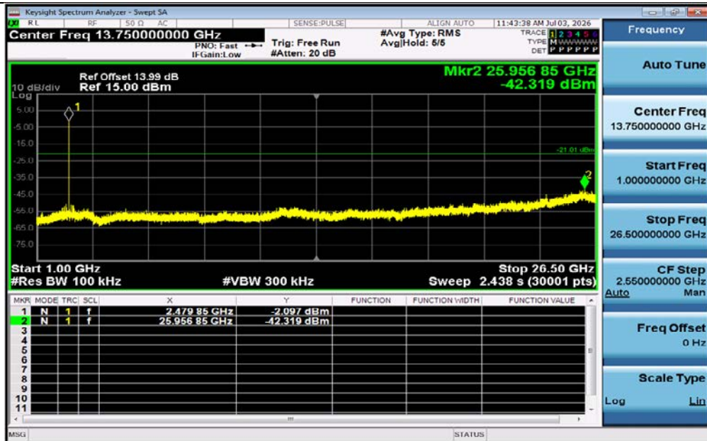
DH5-Ant1-2480-1000-26500-PASS
