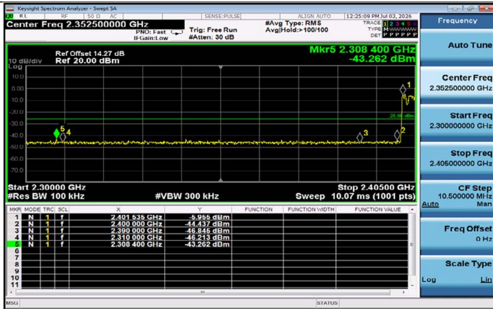
2DH5-Ant1-Hop_2402-PASS
