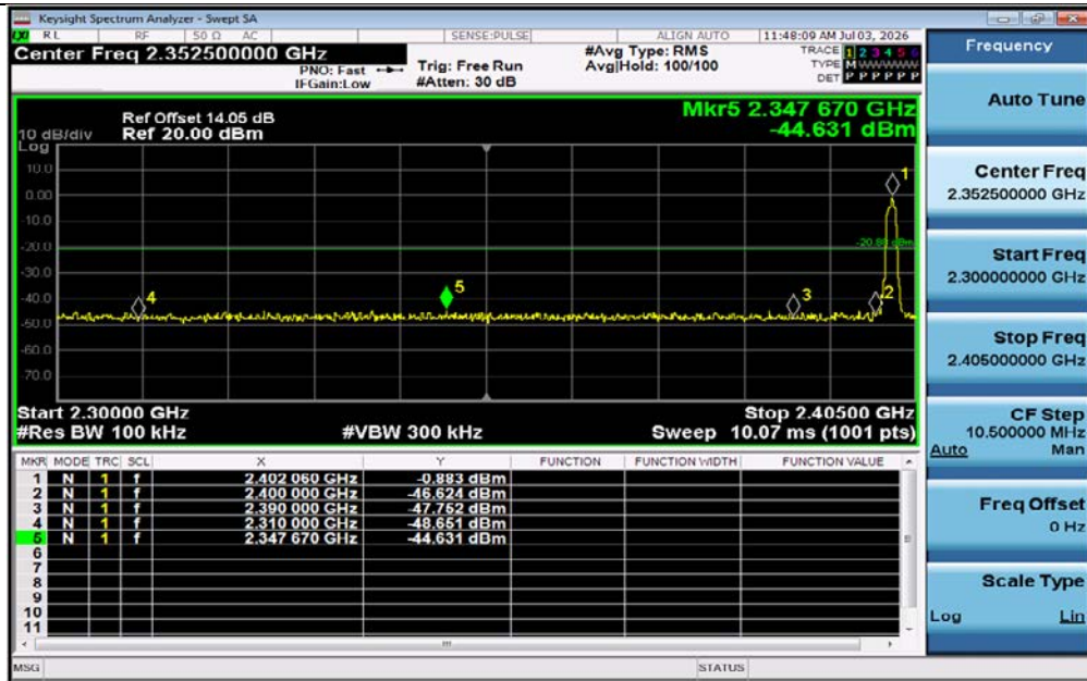
3DH5-Ant1-2402-PASS
