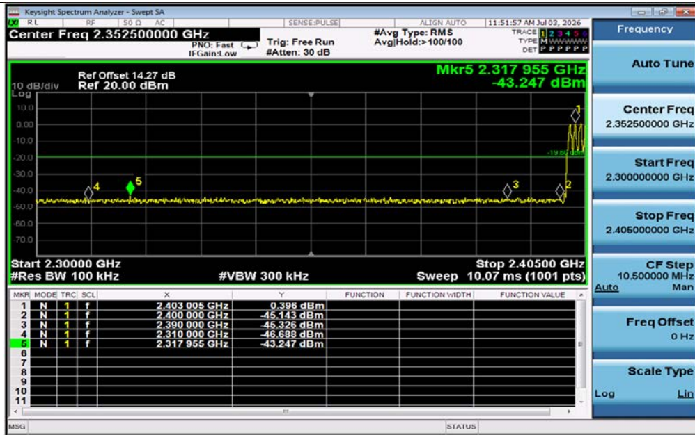
DH5-Ant1-Hop_2402-PASS
