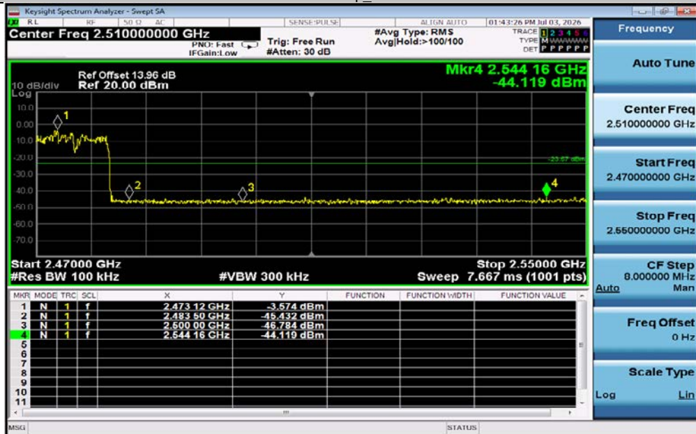
3DH5-Ant1-Hop_2480-PASS
