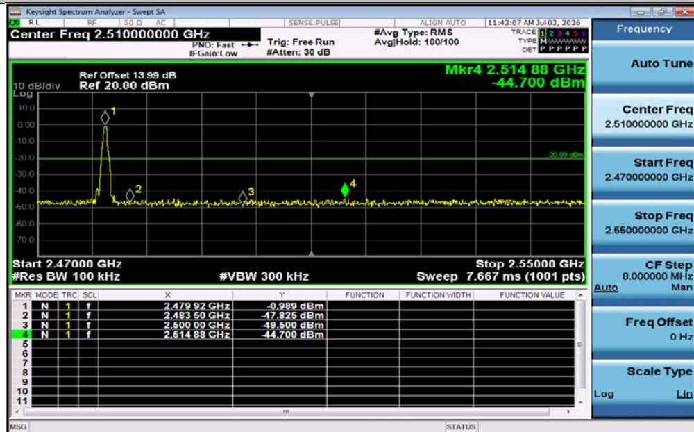
DH5-Ant1-2480-PASS
