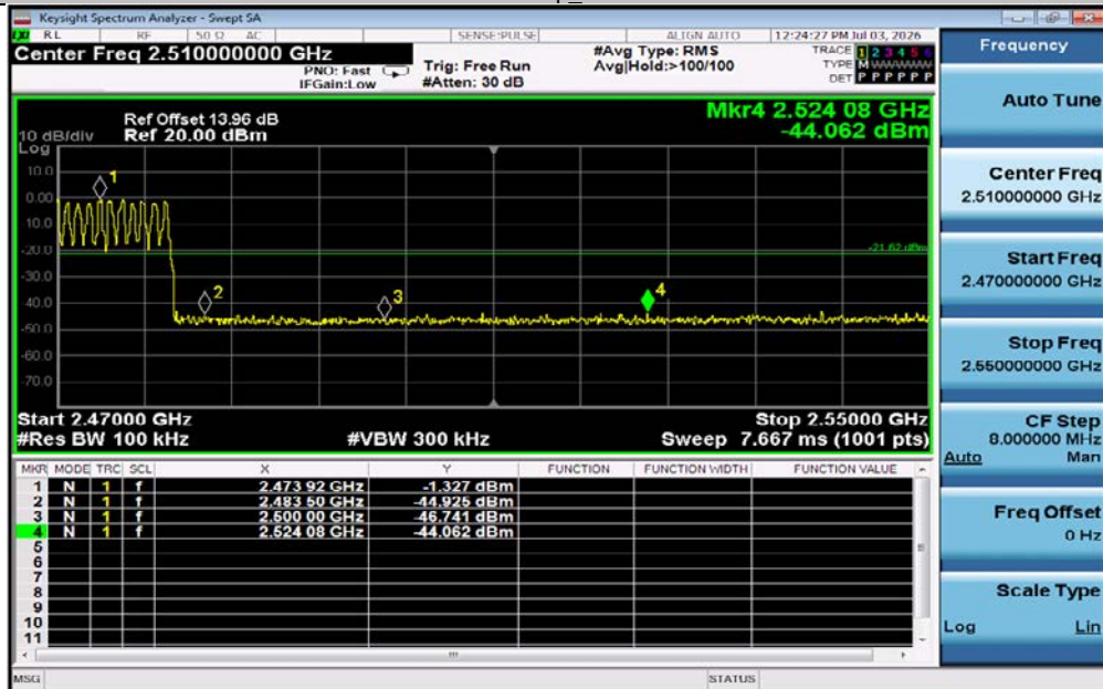
DH5-Ant1-Hop_2480-PASS
