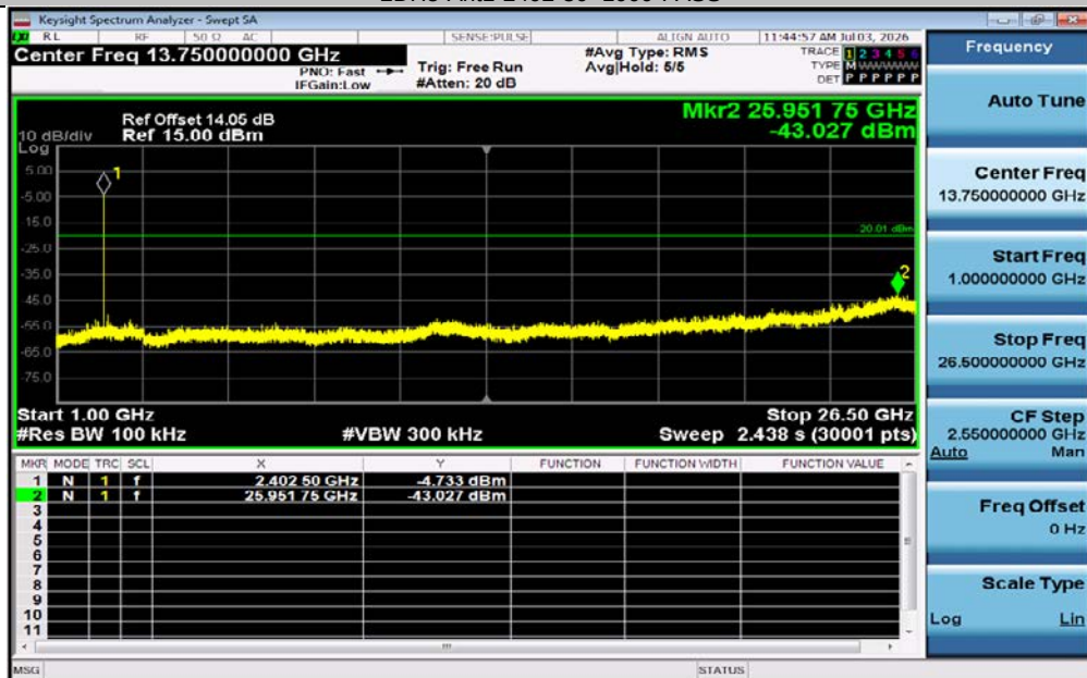
2DH5-Ant1-2402-1000~26500-PASS
