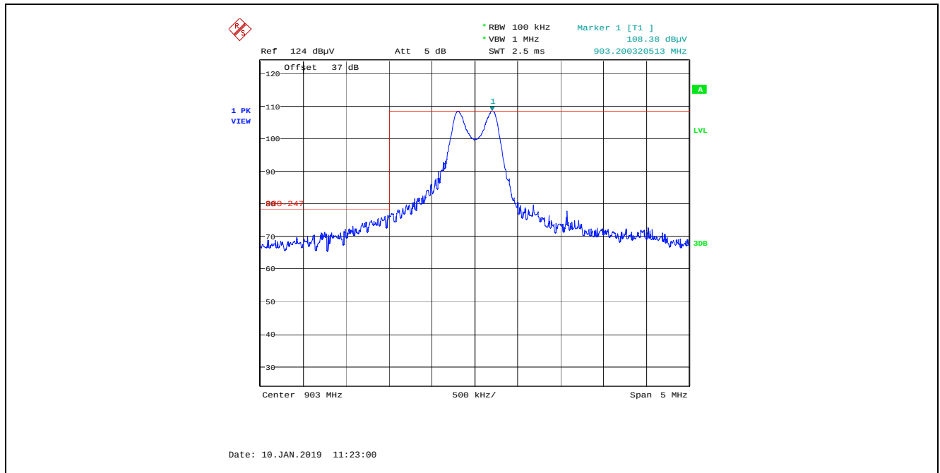
Plot 5.3.4.2.1. Band-Edge Radiated Emissions Rx Antenna in Vertical Polarization, FSK Modulation, 903 MHz
