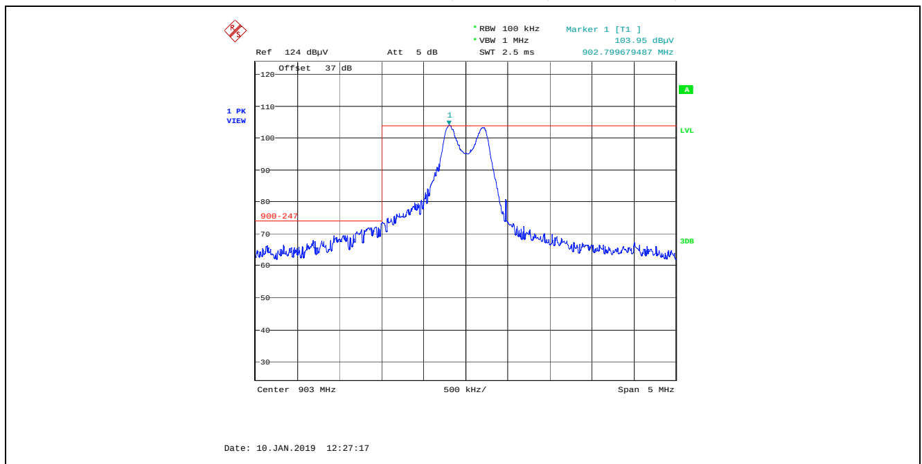
Plot 5.3.4.2.2. Band-Edge Radiated Emissions Rx Antenna in Horizontal Polarization, Polarization, FSK Modulation, 903 MHz
