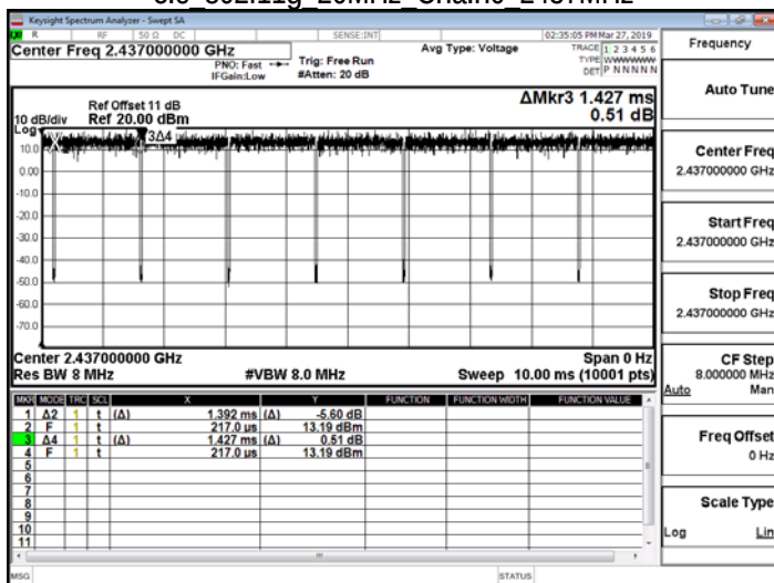
FCC_15_247_WLAN\Duty Cycle 802.11g 20MHz Chain0 2437MHz
