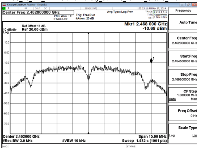
FCC_15_247_WLAN\Power Density_802.11b_20MHz_Chain0_2462MHz
