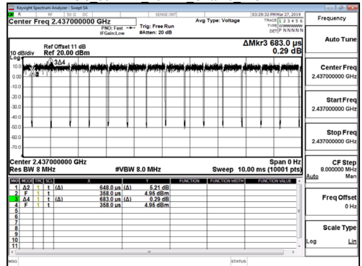
FCC_15_247_WLAN\Duty Cycle 802.11n 40MHz Chain0 2437MHz
