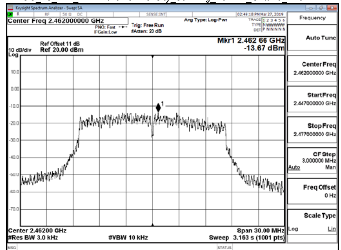
FCC_15_247_WLAN\Power Density_802.11g_20MHz_Chain0_2462MHz
