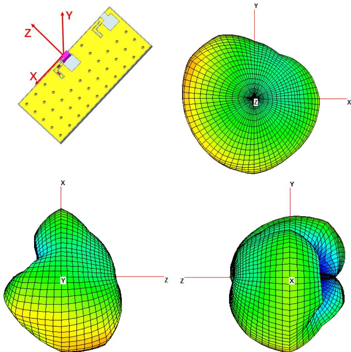
FIGURE 4.6.3 3D RADIATION PATTERN OF ANTENNA AT 5500MHZ IN FREE SPACE Test Personnel: FOR CONFIGURE 2
