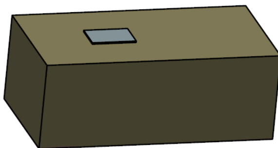
Molex 2119640001 2.4GHz/5GHz Ceramic SMT antenna 3D VIEW
