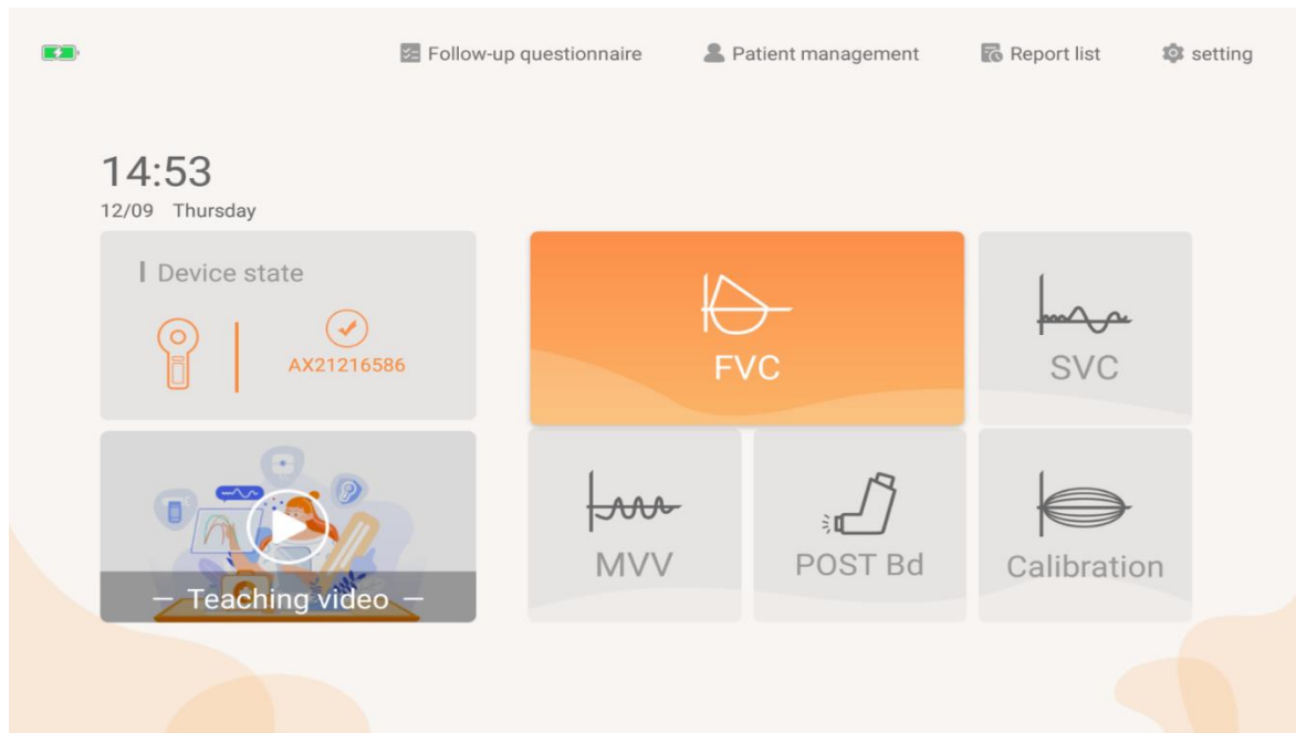
Figure 5 main interface
