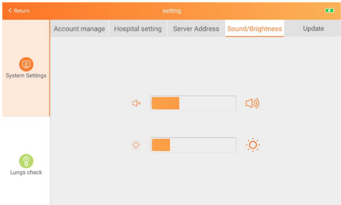
Figure 33 Sound/Brightness interface
