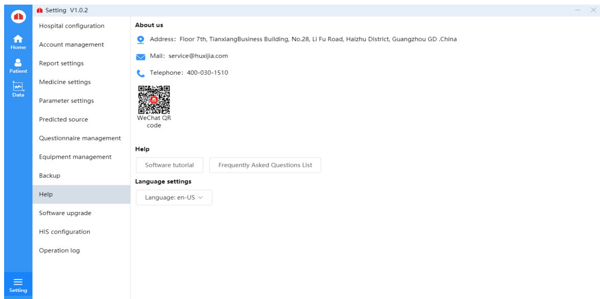
Figure50 Help interface
