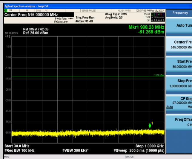
Band2-10MHz-16QAM-18900-1-0-Low-30-1000--61.27-PASS
