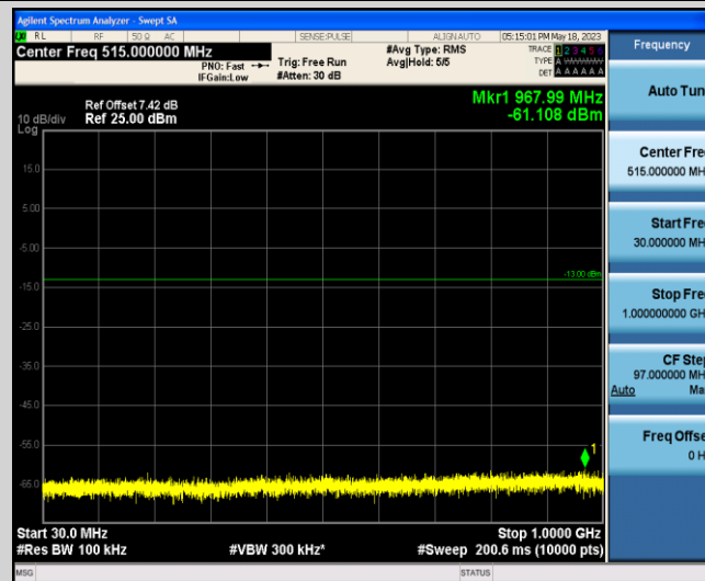
Band2-15MHz-QPSK-19125-1-0-High-30-1000--61.11-PASS
