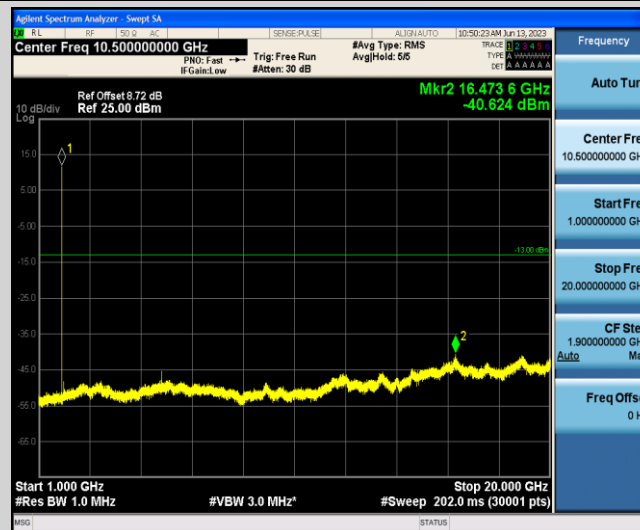
Band2-20MHz-16QAM-18700-1-0-Low-1000-20000--40.62-PASS
