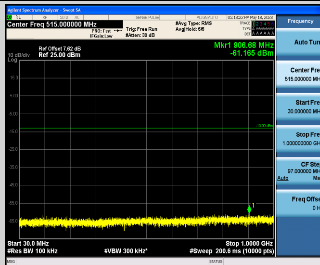
Band2-15MHz-QPSK-18900-1-0-Low-30-1000--61.17-PASS
