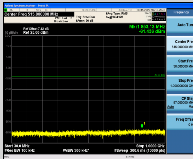
Band2-15MHz-16QAM-19125-1-0-High-30-1000--61.44-PASS
