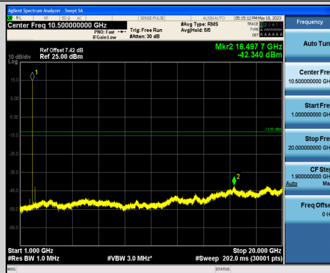
Band2-15MHz-QPSK-19125-1-0-High-1000-20000--42.34-PASS
