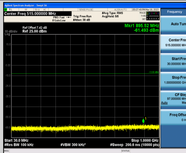
Band2-10MHz-16QAM-19150-1-0-High-30-1000--61.49-PASS
