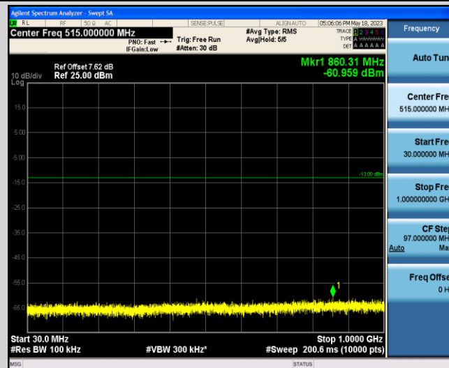
Band2-10MHz-QPSK-18650-1-0-Low-30-1000--60.96-PASS
