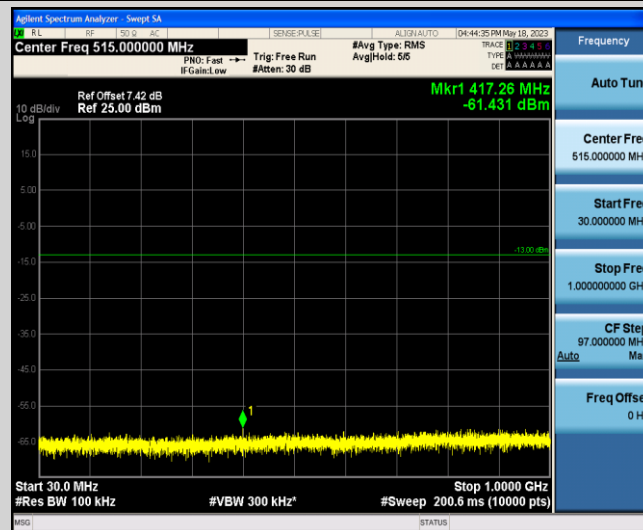
Band2-5MHz-16QAM-19175-1-0-Low-30-1000--61.43-PASS
