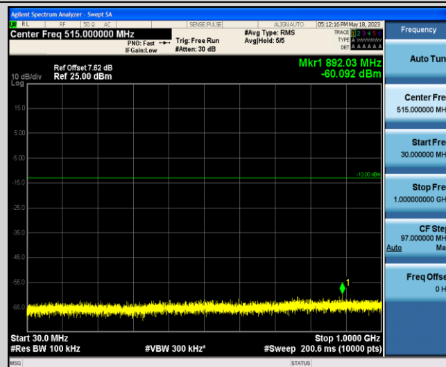
Band2-15MHz-QPSK-18675-1-0-Low-30-1000--60.09-PASS
