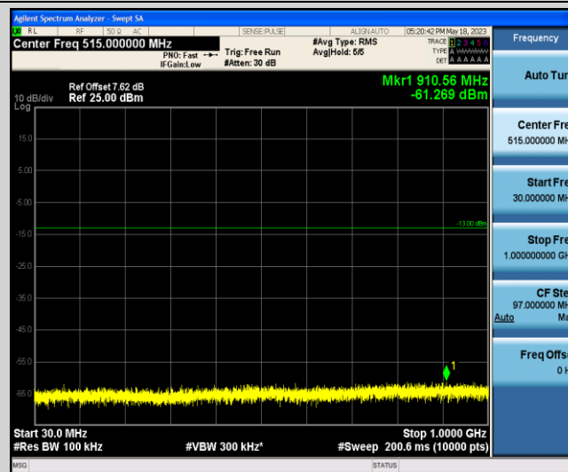
Band2-20MHz-16QAM-18900-1-0-Low-30-1000--61.27-PASS
