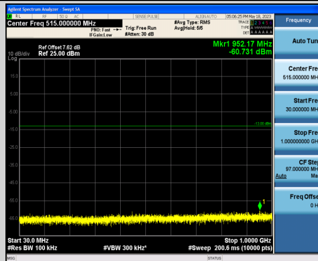
Band2-10MHz-16QAM-18650-1-0-Low-30-1000--60.73-PASS
