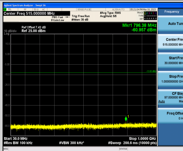
Band2-20MHz-QPSK-19100-1-0-High-30-1000--60.96-PASS
