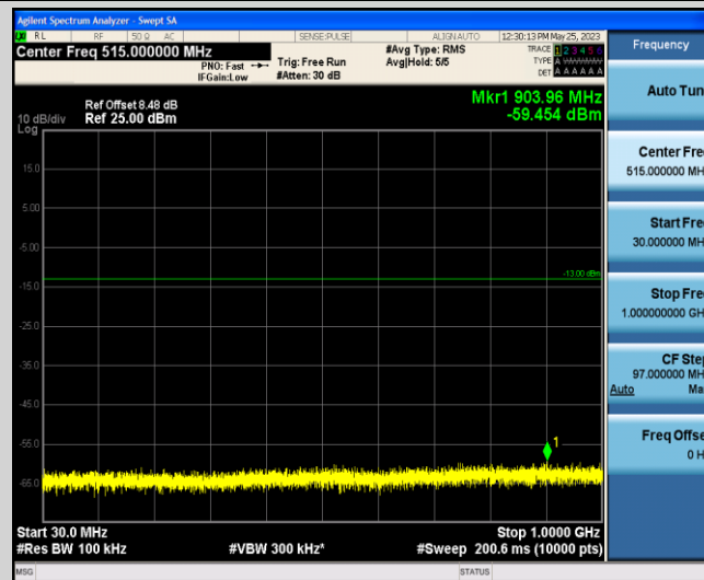
Band4-1.4MHz-16QAM-20393-1-0-Low-30-1000--59.45-PASS
