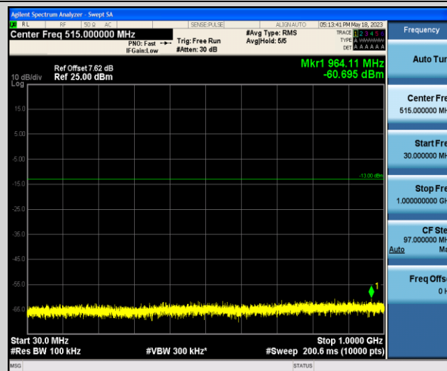
Band2-15MHz-16QAM-18900-1-0-Low-30-1000--60.7-PASS
