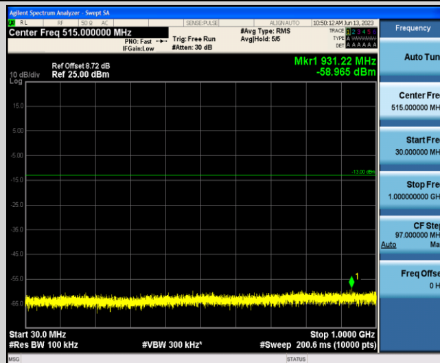
Band2-20MHz-16QAM-18700-1-0-Low-30-1000--58.97-PASS
