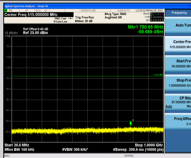
Band4-1.4MHz-16QAM-20175-1-0-Low-30-1000--59.69-PASS
