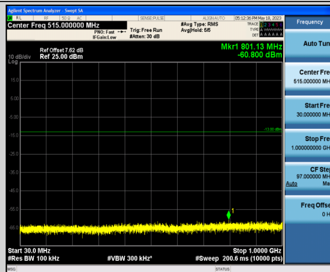
Band2-15MHz-16QAM-18675-1-0-Low-30-1000--60.8-PASS
