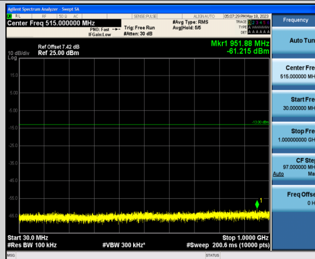
Band2-10MHz-QPSK-19150-1-0-High-30-1000--61.22-PASS
