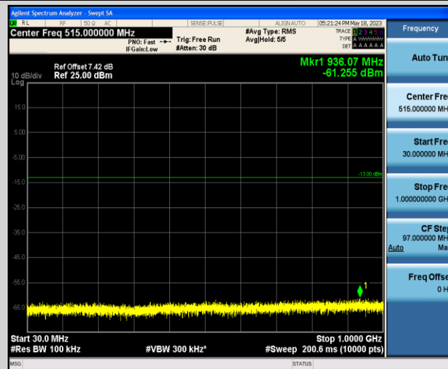
Band2-20MHz-16QAM-19100-1-0-High-30-1000--61.26-PASS
