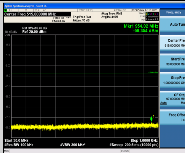
Band4-5MHz-16QAM-20175-1-0-Low-30-1000--59.35-PASS
