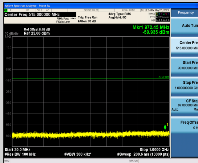
Band4-15MHz-16QAM-20325-1-0-Low-30-1000--59.94-PASS
