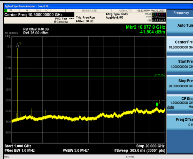
Band4-15MHz-QPSK-20325-1-0-Low-1000-20000--41.5-PASS
