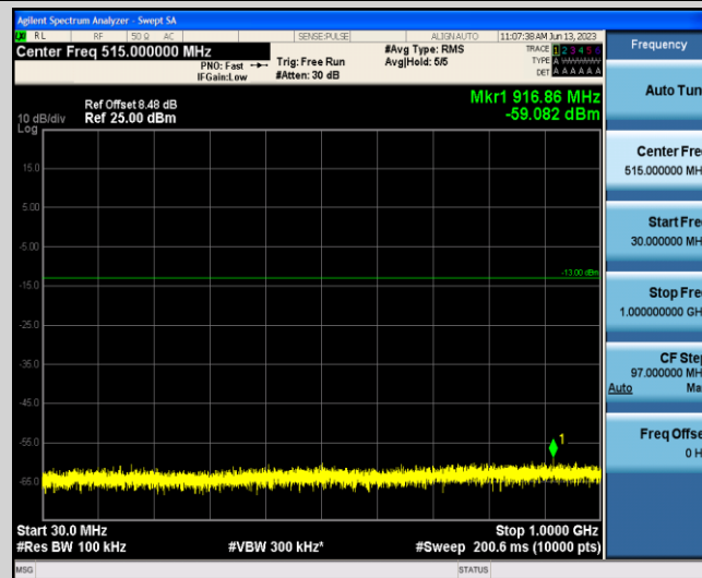
Band4-20MHz-QPSK-20300-1-0-High-30-1000--59.08-PASS
