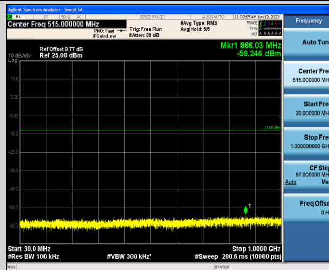
Band4-15MHz-QPSK-20025-1-0-Low-30-1000--59.25-PASS
