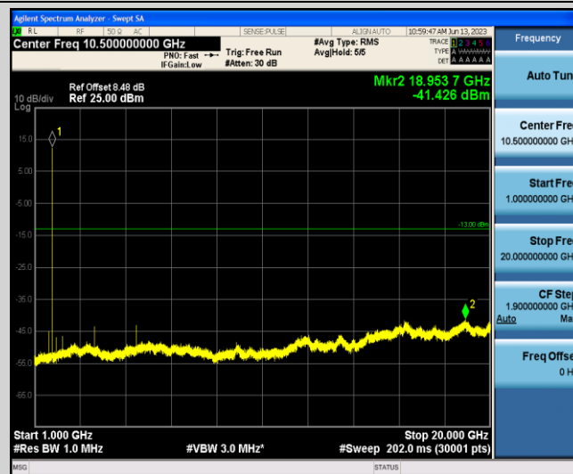
Band4-5MHz-16QAM-20375-1-0-Low-1000-20000--41.43-PASS
