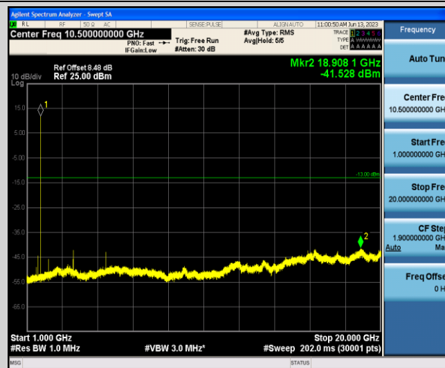
Band4-10MHz-QPSK-20350-1-0-Low-1000-20000--41.53-PASS
