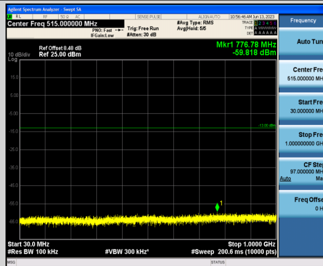
Band4-3MHz-16QAM-20385-1-0-Low-30-1000--59.82-PASS
