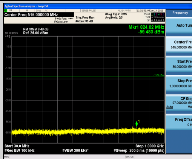
Band4-15MHz-QPSK-20175-1-0-Low-30-1000--59.48-PASS
