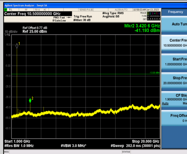
Band4-5MHz-QPSK-19975-1-0-Low-1000-20000--41.19-PASS
