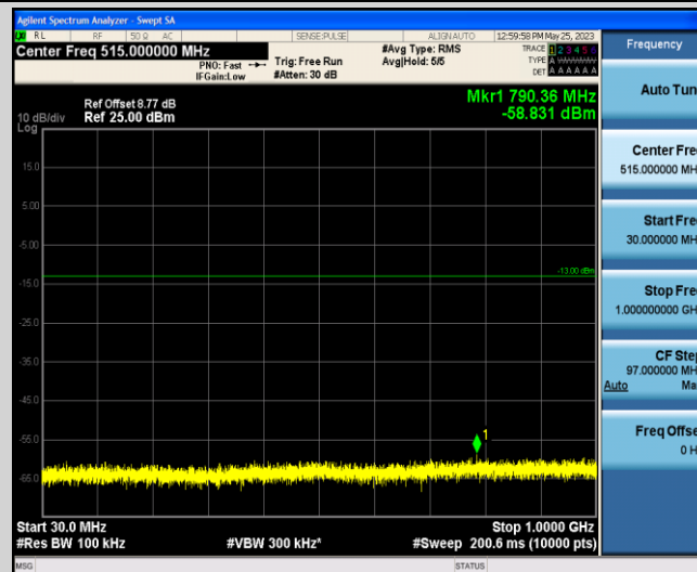
Band4-10MHz-16QAM-20000-1-0-Low-30-1000--58.83-PASS
