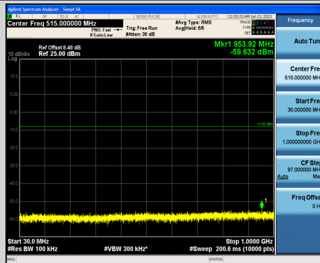
Band4-15MHz-16QAM-20175-1-0-Low-30-1000--59.63-PASS
