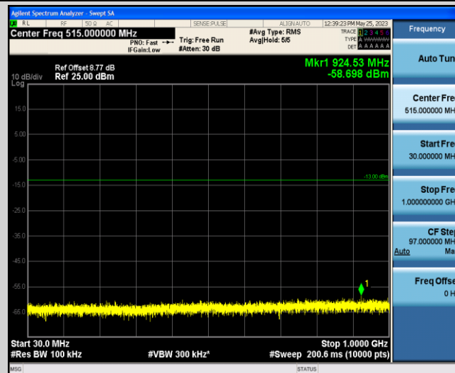
Band4-3MHz-16QAM-19965-1-0-Low-30-1000--58.7-PASS
