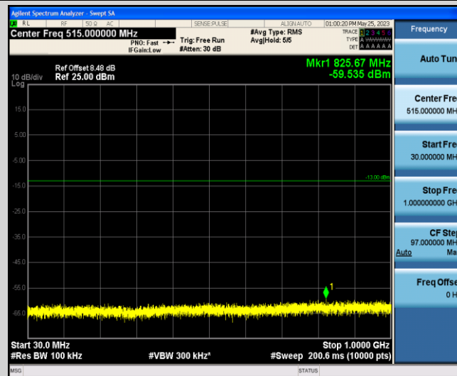
Band4-10MHz-QPSK-20175-1-0-Low-30-1000--59.54-PASS
