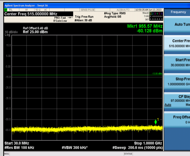
Band4-5MHz-16QAM-20375-1-0-Low-30-1000--60.13-PASS
