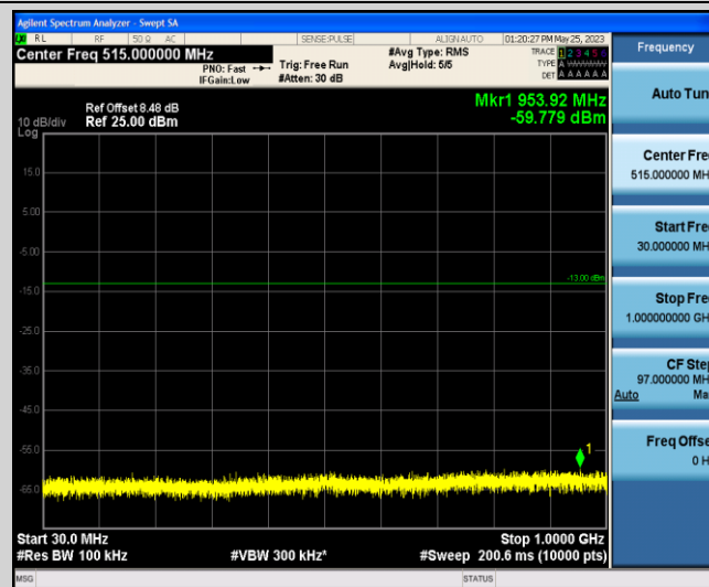
Band4-20MHz-QPSK-20175-1-0-Low-30-1000--59.78-PASS
