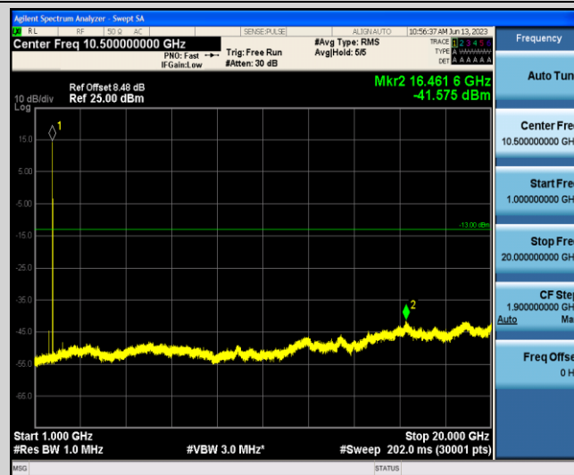
Band4-3MHz-QPSK-20385-1-0-Low-1000-20000--41.58-PASS
