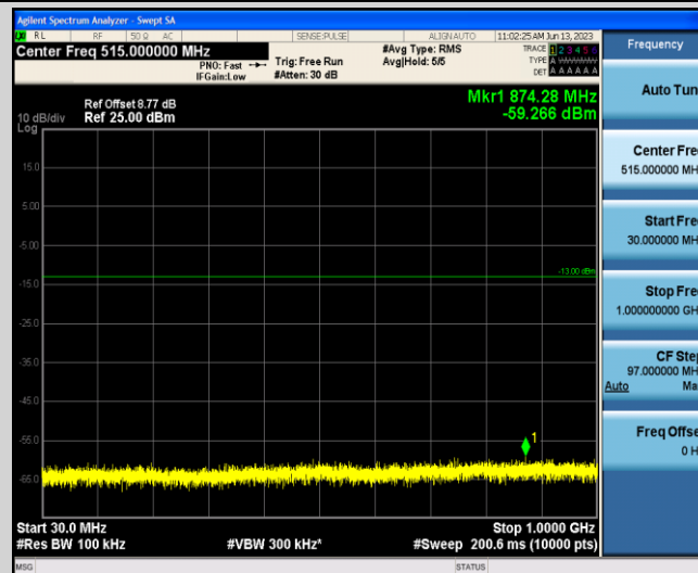
Band4-15MHz-16QAM-20025-1-0-Low-30-1000--59.27-PASS
