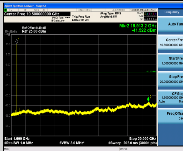
Band4-10MHz-16QAM-20350-1-0-Low-1000-20000--41.52-PASS
