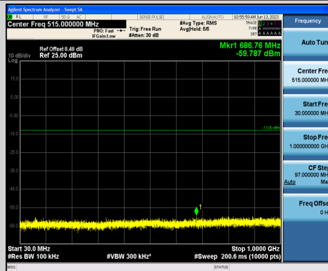
Band4-3MHz-16QAM-20175-1-0-Low-30-1000--59.79-PASS
