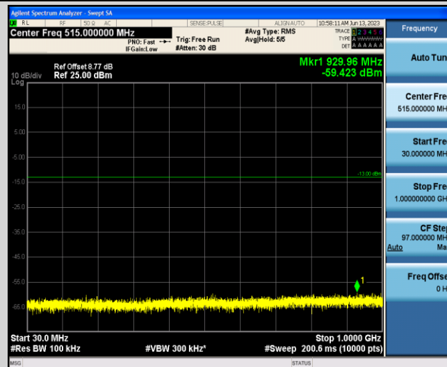
Band4-5MHz-16QAM-19975-1-0-Low-30-1000--59.42-PASS
