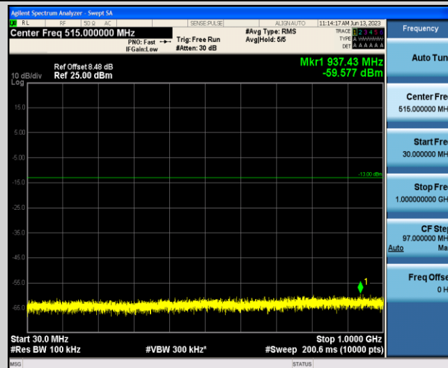
Band66-3MHz-16QAM-132657-1-0-Low-30-1000--59.58-PASS
