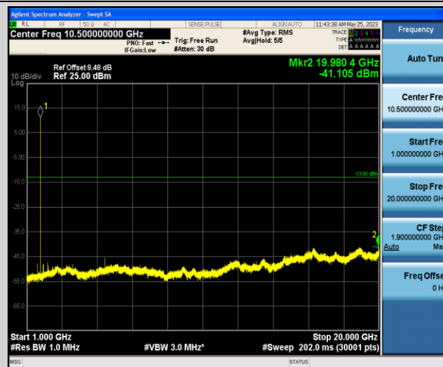
Band66-10MHz-16QAM-132322-1-0-Low-1000-20000--41.11-PASS
