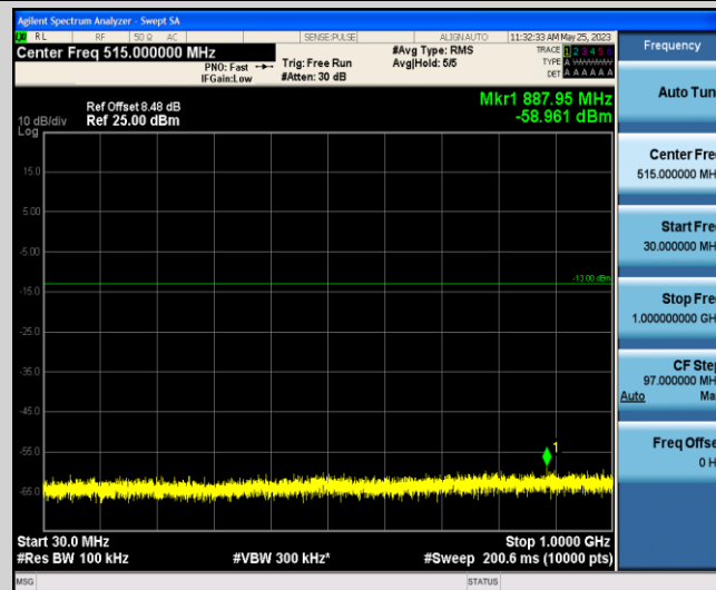
Band66-5MHz-QPSK-132322-1-0-Low-30-1000--58.96-PASS
