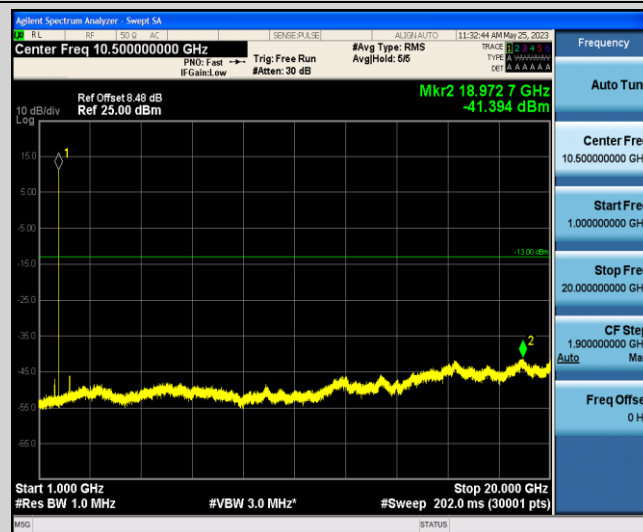
Band66-5MHz-QPSK-132322-1-0-Low-1000-20000--41.39-PASS
