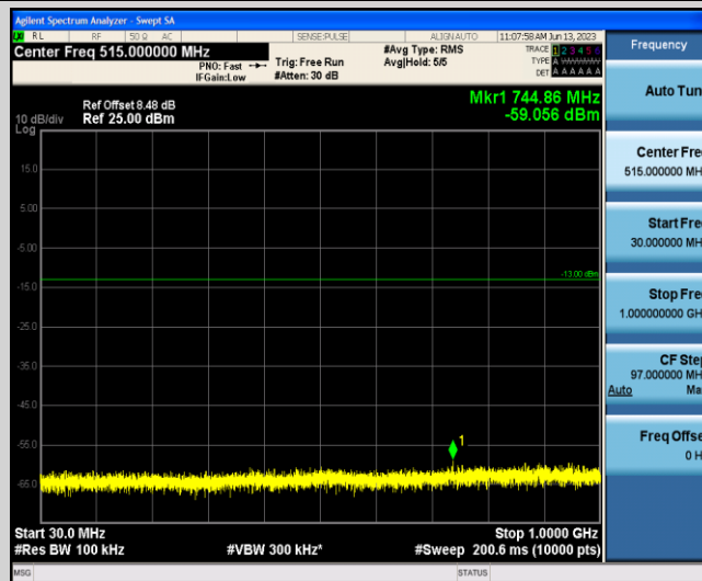
Band4-20MHz-16QAM-20300-1-0-High-30-1000--59.06-PASS
