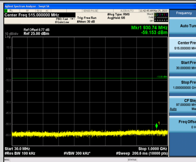
Band66-10MHz-16QAM-132022-1-0-Low-30-1000--59.15-PASS
