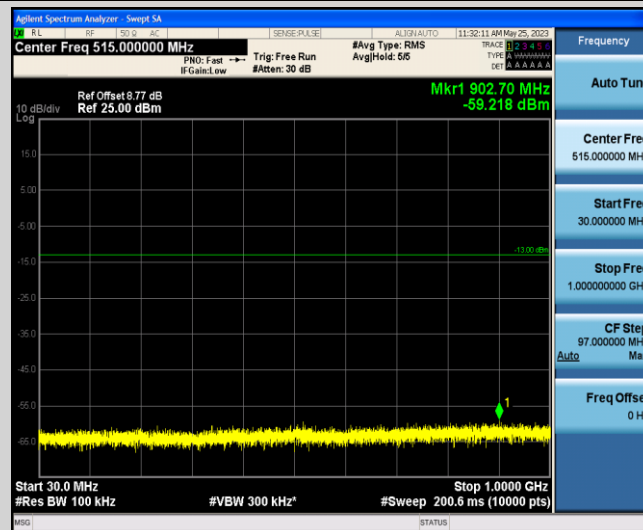
Band66-5MHz-16QAM-131997-1-0-Low-30-1000--59.22-PASS
