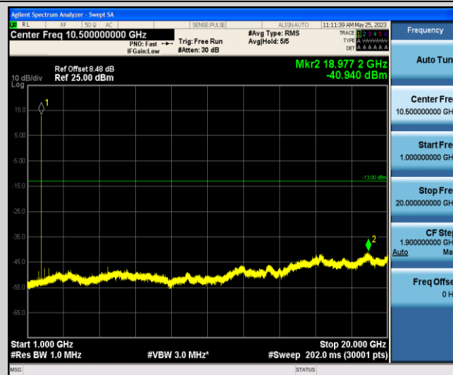
Band66-1.4MHz-QPSK-132322-1-0-Low-1000-20000--40.94-PASS
