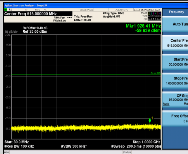
Band66-1.4MHz-16QAM-132665-1-0-Low-30-1000--59.64-PASS
