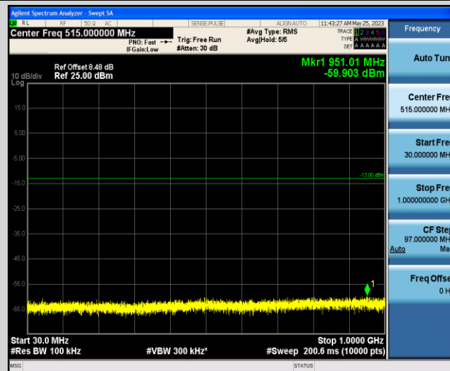
Band66-10MHz-16QAM-132322-1-0-Low-30-1000--59.9-PASS
