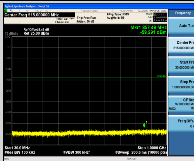
Band4-20MHz-16QAM-20175-1-0-Low-30-1000--59.29-PASS
