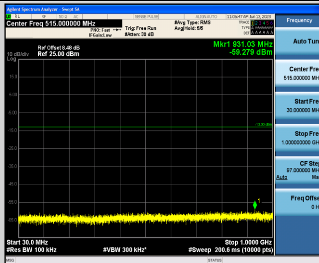
Band4-20MHz-1RB#0@Low-20300-1-0-High-30-1000--59.28-PASS
