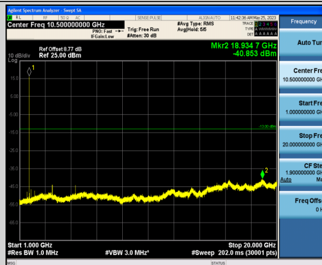
Band66-10MHz-QPSK-132022-1-0-Low-1000-20000--40.85-PASS
