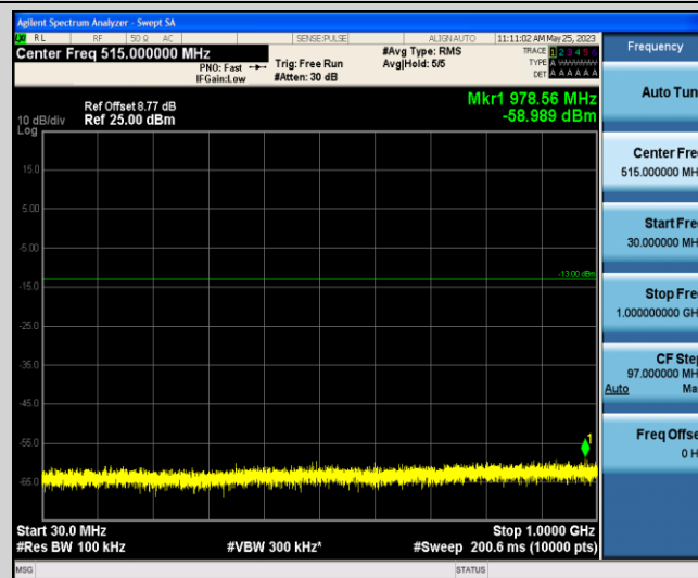
Band66-1.4MHz-16QAM-131979-1-0-Low-30-1000--58.99-PASS
