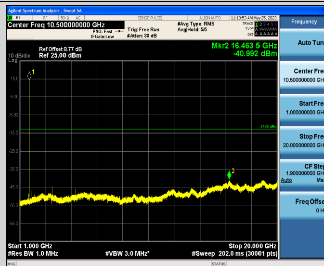
Band66-1.4MHz-QPSK-131979-1-0-Low-1000-20000--40.99-PASS
