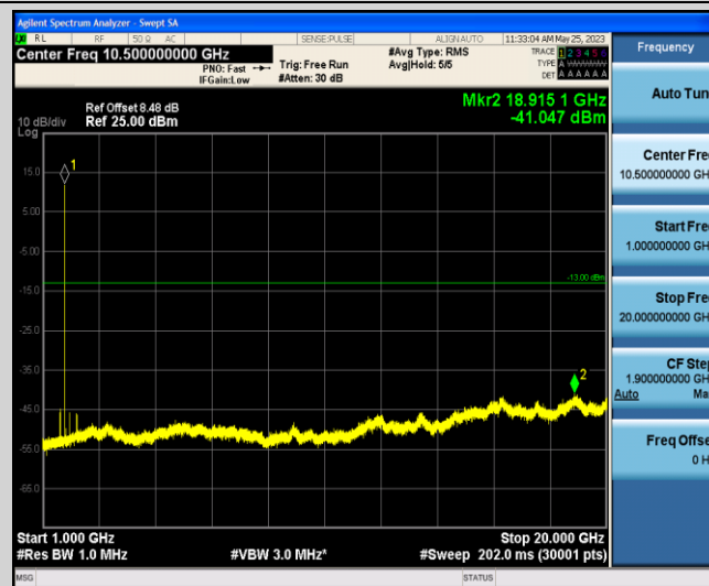
Band66-5MHz-16QAM-132322-1-0-Low-1000-20000--41.05-PASS
