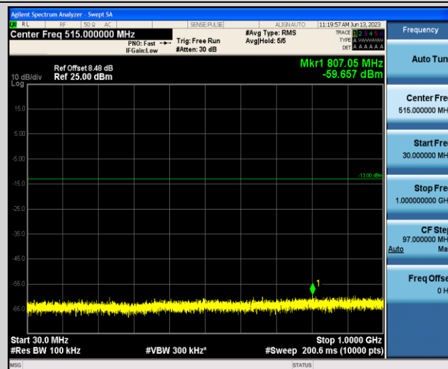
Band66-10MHz-16QAM-132622-1-0-Low-30-1000--59.66-PASS
