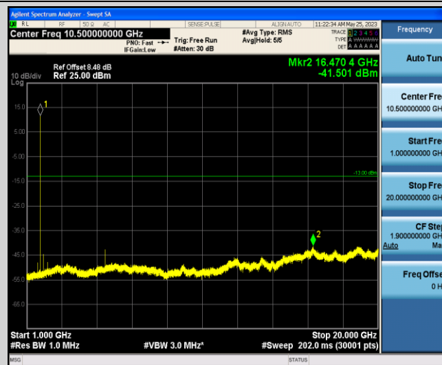
Band66-3MHz-16QAM-132322-1-0-Low-1000-20000--41.5-PASS
