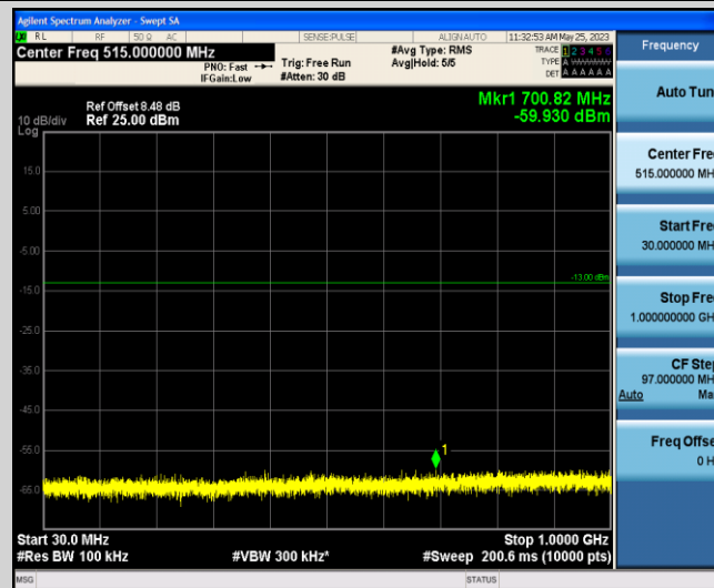
Band66-5MHz-16QAM-132322-1-0-Low-30-1000--59.93-PASS
