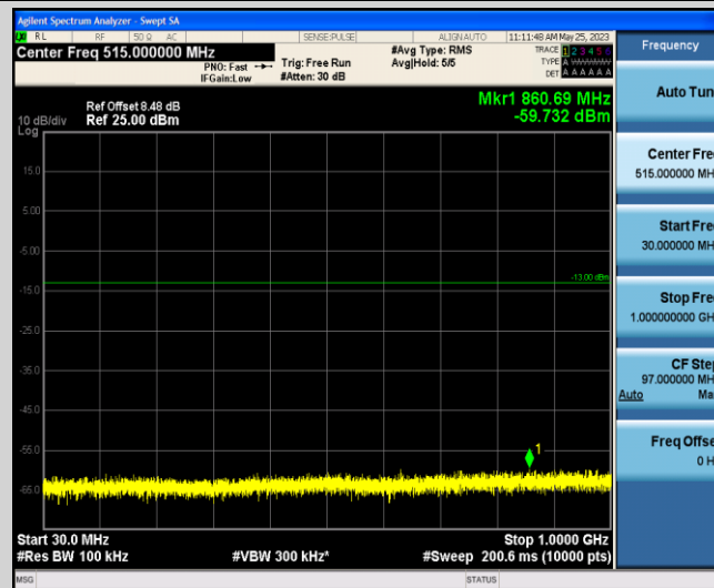
Band66-1.4MHz-16QAM-132322-1-0-Low-30-1000--59.73-PASS
