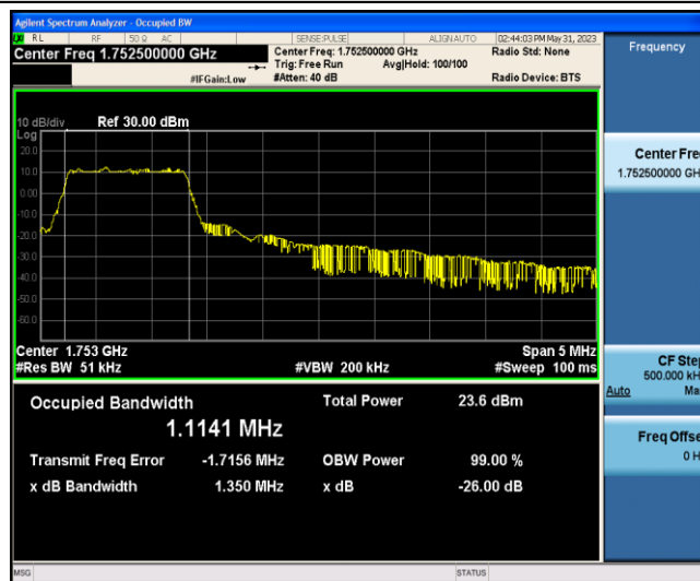
Band4-5MHz-QPSK-20375-6-0-Low-1.1141-1.350-PASS
