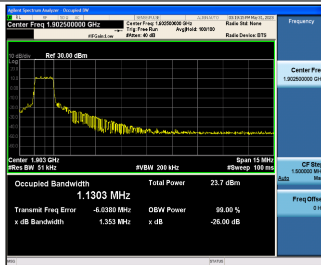
Band2-15MHz-16QAM-19125-6-0-Low-1.1303-1.353-PASS
