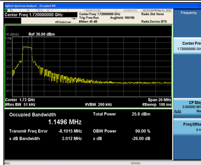
Band4-20MHz-16QAM-20050-6-0-Low-1.1496-2.012-PASS
