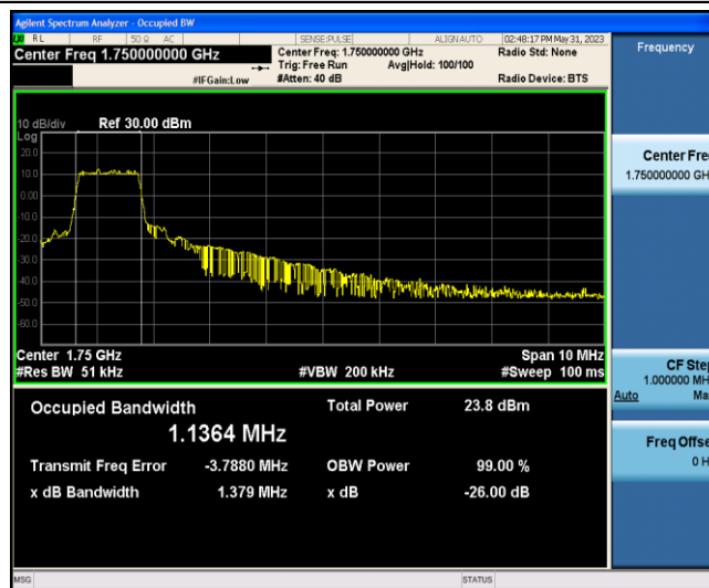
Band4-10MHz-16QAM-20350-6-0-Low-1.1364-1.379-PASS
