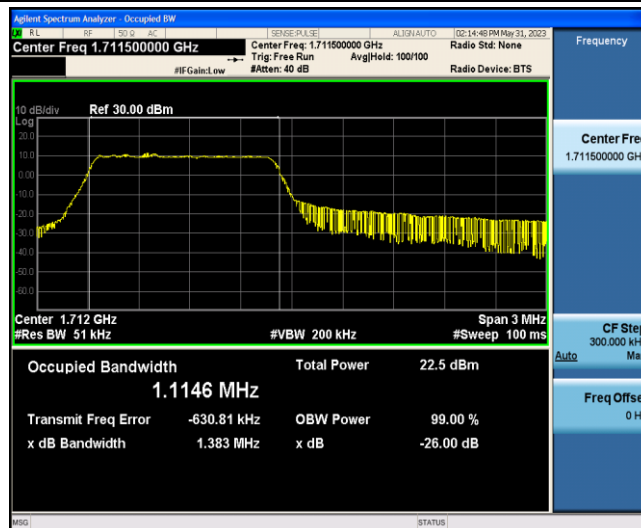
Band66-3MHz-QPSK-131987-6-0-Low-1.1146-1.383-PASS
