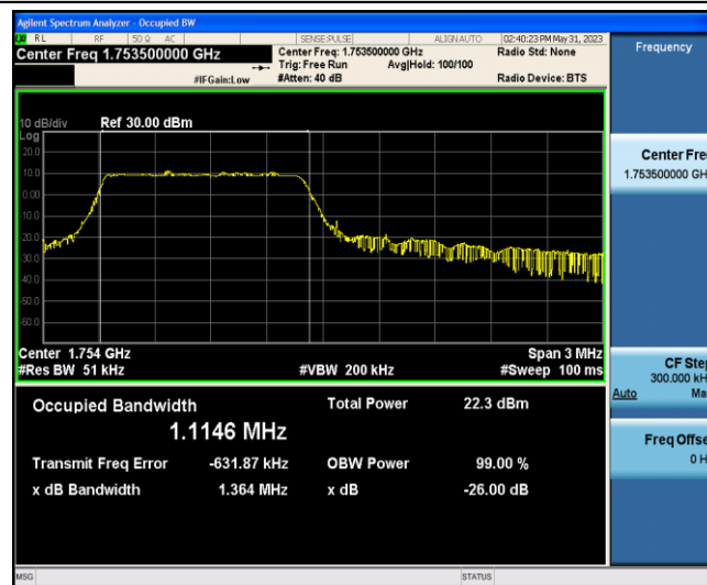
Band4-3MHz-16QAM-20385-6-0-Low-1.1146-1.364-PASS
