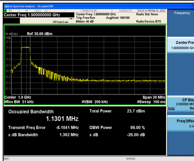
Band2-20MHz-16QAM-19100-6-0-Low-1.1301-1.362-PASS
