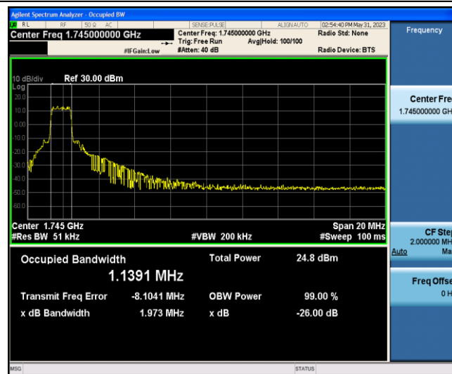
Band4-20MHz-16QAM-20300-6-0-Low-1.1391-1.973-PASS
