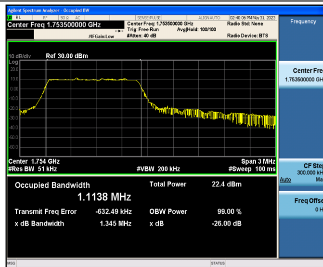
Band4-3MHz-QPSK-20385-6-0-Low-1.1138-1.345-PASS
