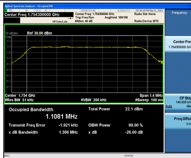
Band4-1.4MHz-QPSK-20393-6-0-Low-1.1081-1.366-PASS
