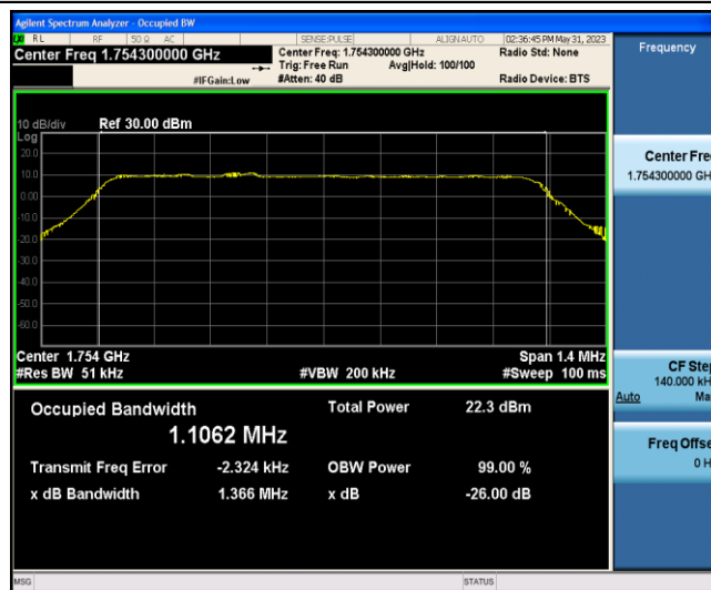
Band4-1.4MHz-16QAM-20393-6-0-Low-1.1062-1.366-PASS
