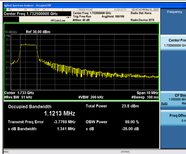
Band4-10MHz-16QAM-20175-6-0-Low-1.1213-1.341-PASS
