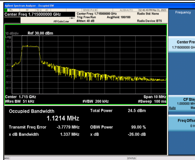
Band4-10MHz-QPSK-20000-6-0-Low-1.1214-1.337-PASS
