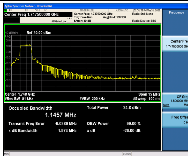
Band4-15MHz-QPSK-20325-6-0-Low-1.1457-1.973-PASS
