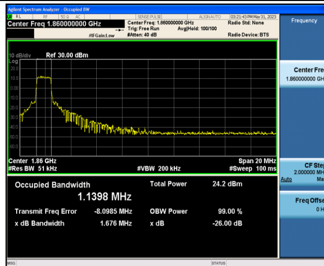
Band2-20MHz-QPSK-18700-6-0-Low-1.1398-1.676-PASS
