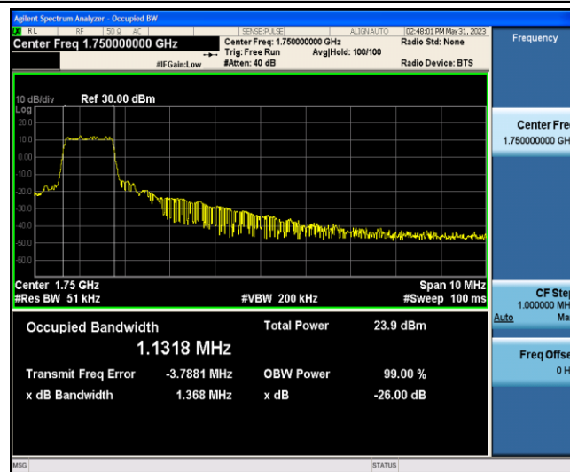
Band4-10MHz-QPSK-20350-6-0-Low-1.1318-1.368-PASS
