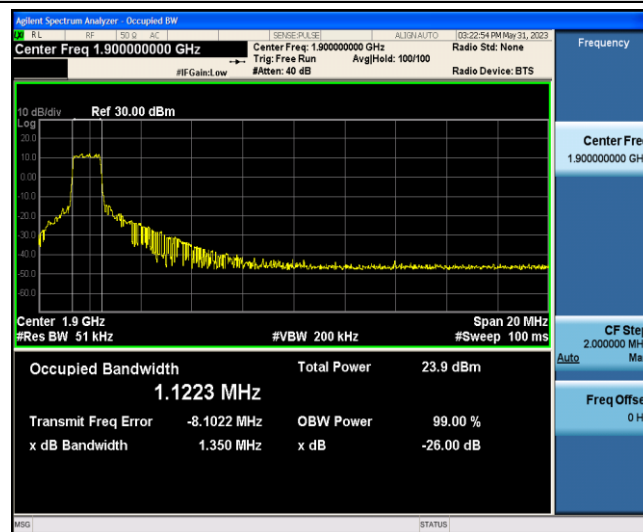
Band2-20MHz-QPSK-19100-6-0-Low-1.1223-1.350-PASS
