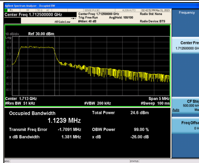
Band4-5MHz-QPSK-19975-6-0-Low-1.1239-1.381-PASS
