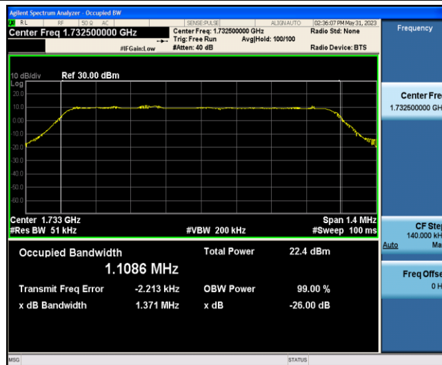
Band4-1.4MHz-16QAM-20175-6-0-Low-1.1086-1.371-PASS
