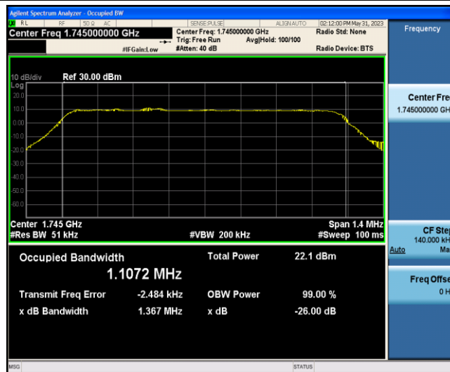
Band66-1.4MHz-16QAM-132322-6-0-Low-1.1072-1.367-PASS
