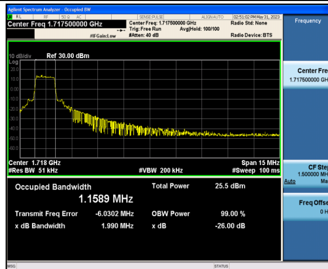
Band4-15MHz-16QAM-20025-6-0-Low-1.1589-1.990-PASS
