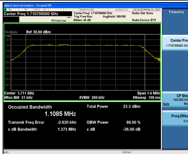
Band4-1.4MHz-QPSK-19957-6-0-Low-1.1085-1.373-PASS
