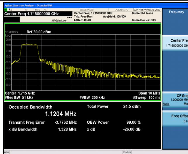
Band4-10MHz-16QAM-20000-6-0-Low-1.1204-1.328-PASS
