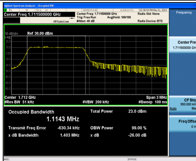
Band4-3MHz-QPSK-19965-6-0-Low-1.1143-1.403-PASS
