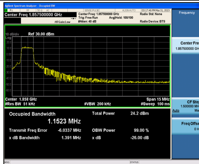
Band2-15MHz-QPSK-18675-6-0-Low-1.1523-1.391-PASS
