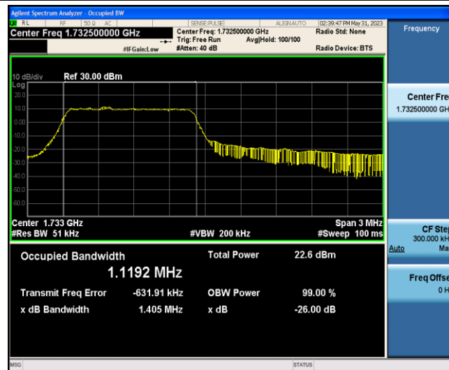
Band4-3MHz-16QAM-20175-6-0-Low-1.1192-1.405-PASS
