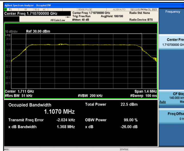
Band66-1.4MHz-QPSK-131979-6-0-Low-1.1070-1.368-PASS
