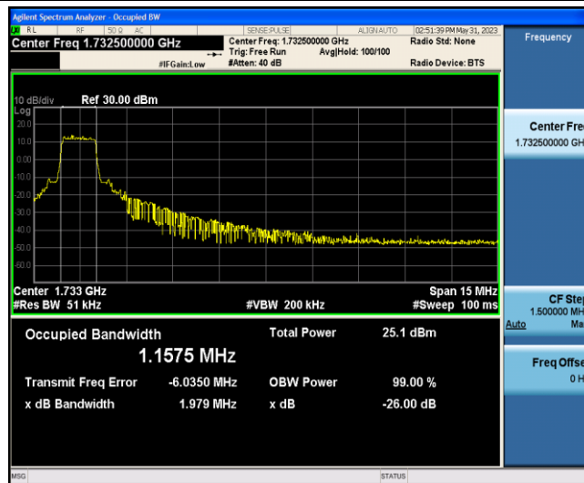
Band4-15MHz-16QAM-20175-6-0-Low-1.1575-1.979-PASS
