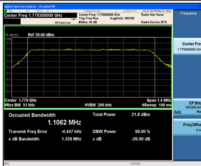
Band66-1.4MHz-16QAM-132665-6-0-Low-1.1062-1.339-PASS
