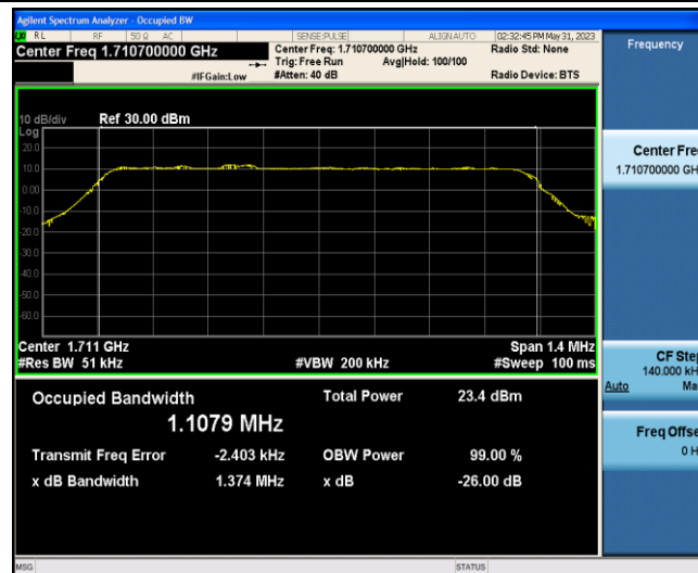
Band4-1.4MHz-16QAM-19957-6-0-Low-1.1079-1.374-PASS
