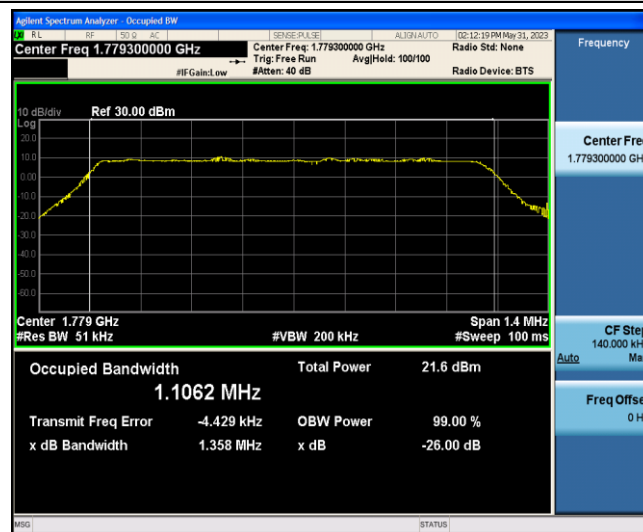
Band66-1.4MHz-QPSK-132665-6-0-Low-1.1062-1.358-PASS
