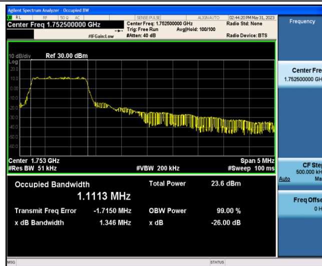
Band4-5MHz-16QAM-20375-6-0-Low-1.1113-1.346-PASS
