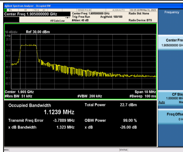
Band2-10MHz-16QAM-19150-6-0-Low-1.1239-1.323-PASS
