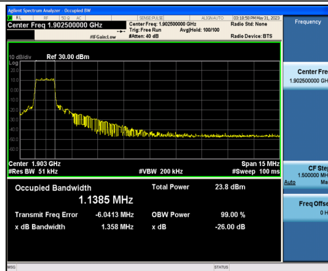
Band2-15MHz-QPSK-19125-6-0-Low-1.1385-1.358-PASS
