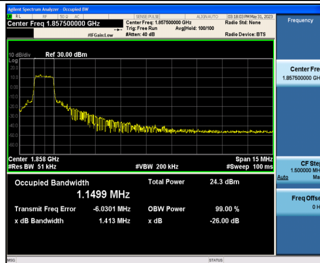
Band2-15MHz-16QAM-18675-6-0-Low-1.1499-1.413-PASS
