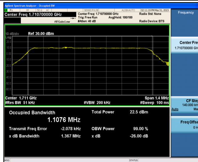
Band66-1.4MHz-16QAM-131979-6-0-Low-1.1076-1.367-PASS
