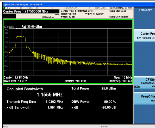
Band4-15MHz-QPSK-20025-6-0-Low-1.1555-1.994-PASS
