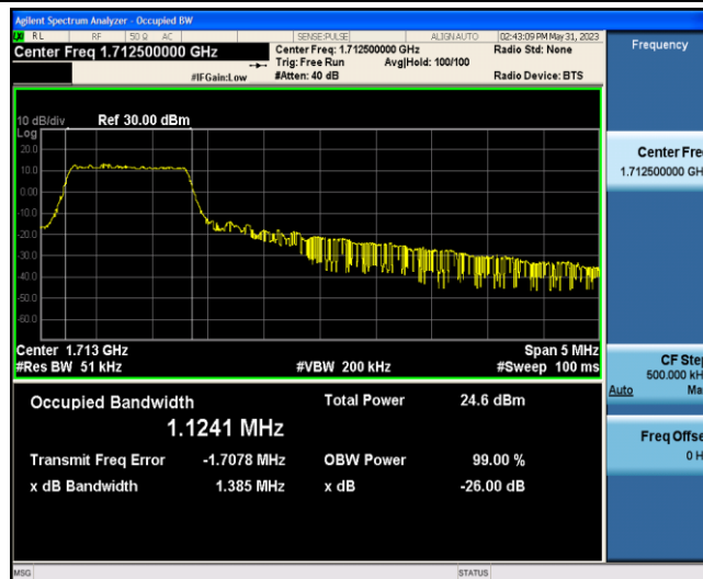
Band4-5MHz-16QAM-19975-6-0-Low-1.1241-1.385-PASS
