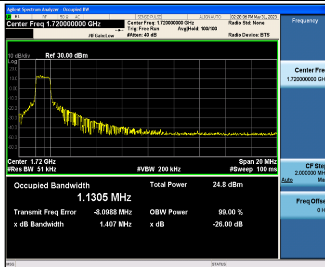
Band66-20MHz-16QAM-132072-6-0-Low-1.1305-1.407-PASS
