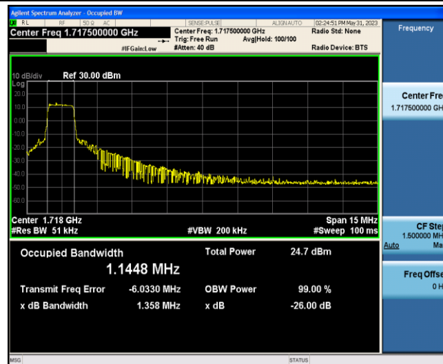
Band66-15MHz-16QAM-132047-6-0-Low-1.1448-1.358-PASS
