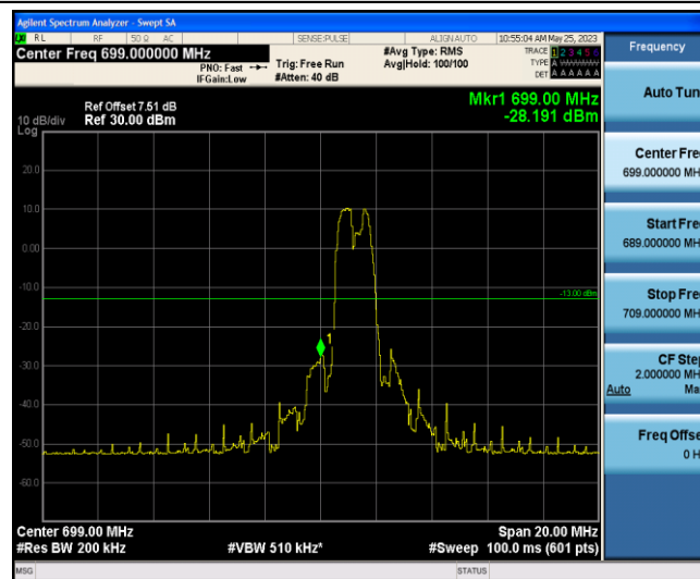
Band12-10MHz-QPSK-23060-6-0-Low--28.19-PASS
