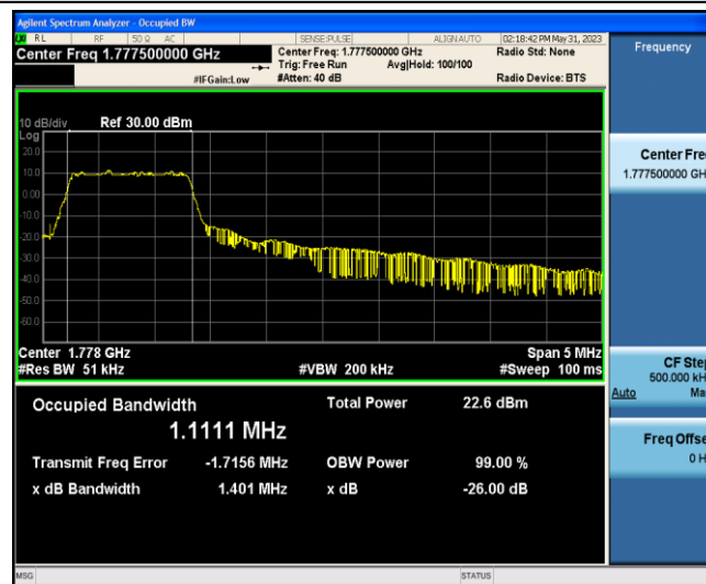
Band66-5MHz-16QAM-132647-6-0-Low-1.1111-1.401-PASS
