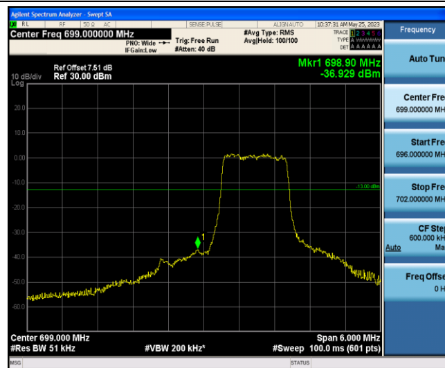
Band12-3MHz-16QAM-23025-6-0-Low--36.93-PASS
