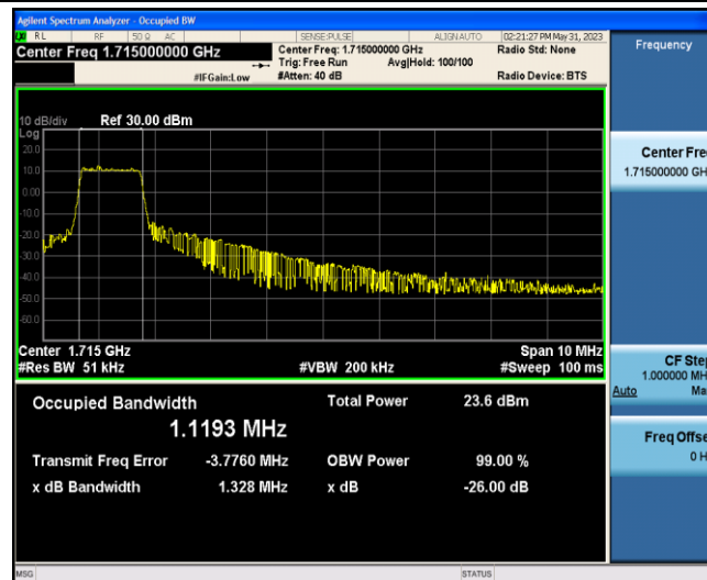
Band66-10MHz-16QAM-132022-6-0-Low-1.1193-1.328-PASS
