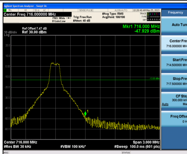
Band12-1.4MHz-QPSK-23173-1-5-High--47.93-PASS
