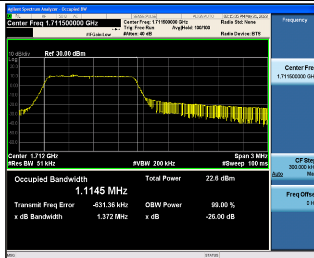
Band66-3MHz-16QAM-131987-6-0-Low-1.1145-1.372-PASS
