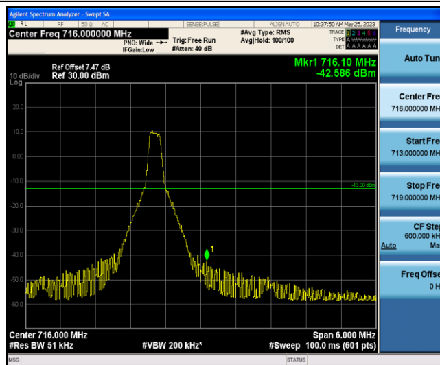
Band12-3MHz-QPSK-23165-1-5-High--42.59-PASS
