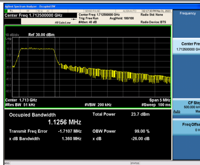
Band66-5MHz-16QAM-131997-6-0-Low-1.1256-1.360-PASS
