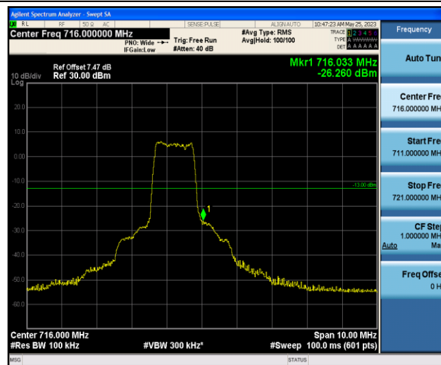
Band12-5MHz-QPSK-23155-6-0-High--26.26-PASS
