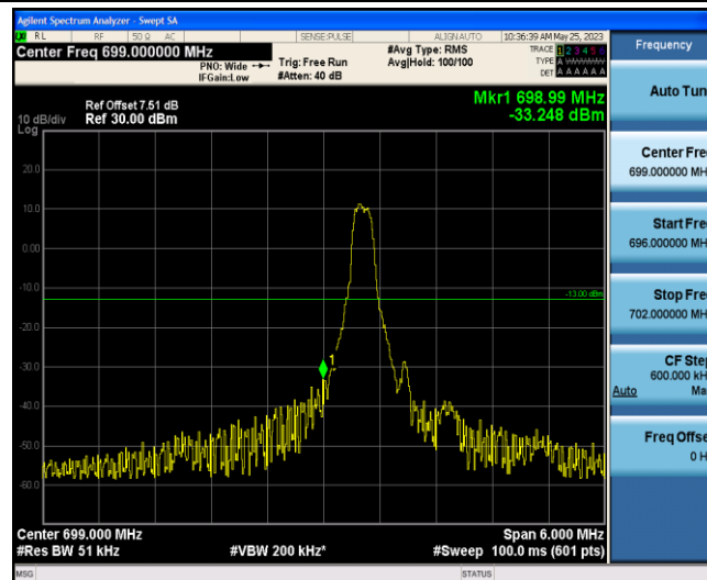
Band12-3MHz-QPSK-23025-1-0-Low--33.25-PASS
