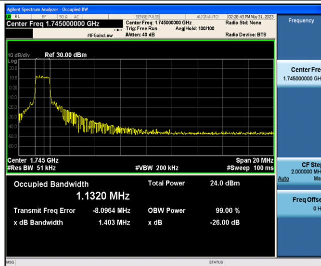
Band66-20MHz-16QAM-132322-6-0-Low-1.1320-1.403-PASS
