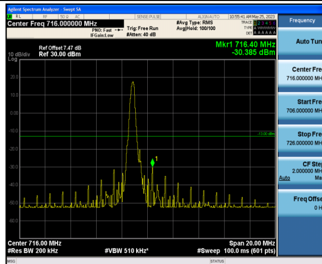
Band12-10MHz-QPSK-23130-1-5-High--30.38-PASS
