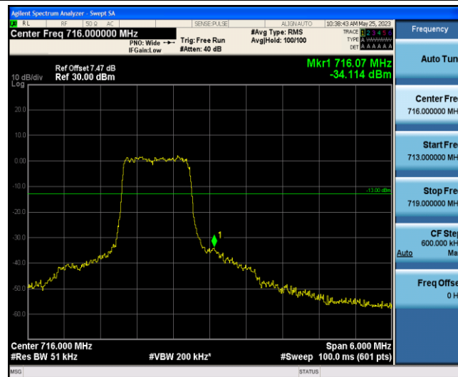
Band12-3MHz-16QAM-23165-6-0-High--34.11-PASS
