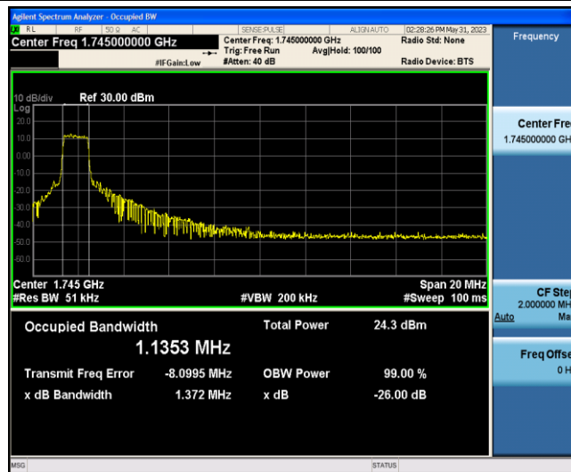
Band66-20MHz-QPSK-132322-6-0-Low-1.1353-1.372-PASS
