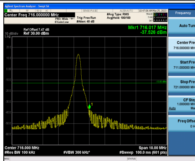
Band12-5MHz-16QAM-23155-1-5-High--37.53-PASS
