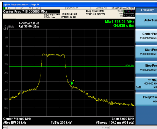
Band12-3MHz-QPSK-23165-6-0-High--34.64-PASS
