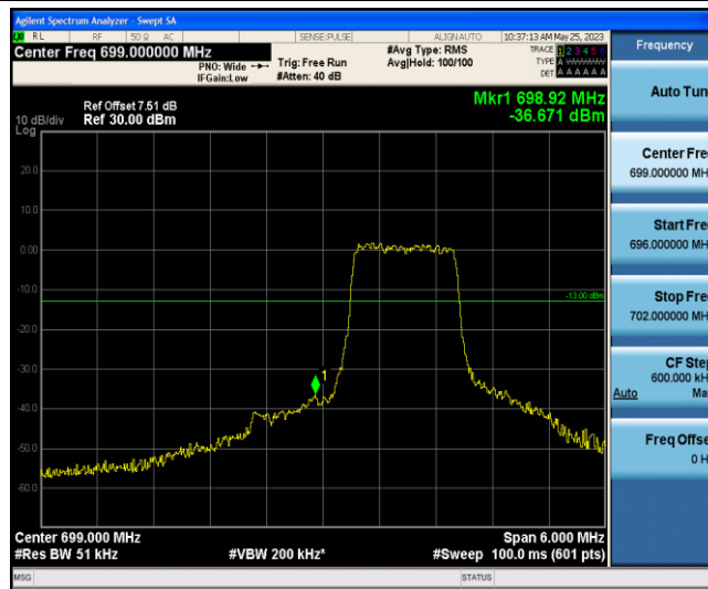
Band12-3MHz-QPSK-23025-6-0-Low--36.67-PASS
