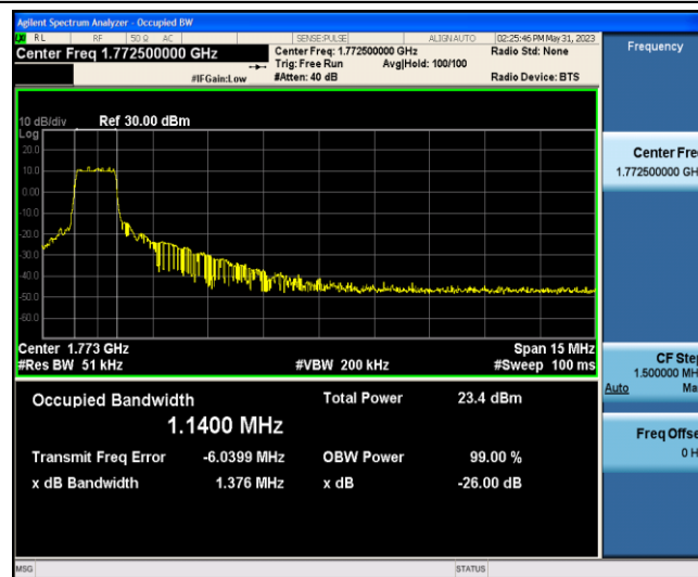
Band66-15MHz-QPSK-132597-6-0-Low-1.1400-1.376-PASS
