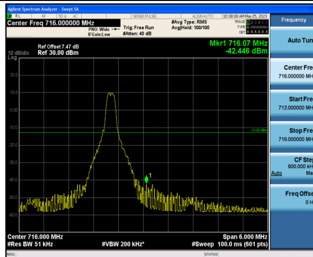
Band12-3MHz-16QAM-23165-1-5-High--42.45-PASS
