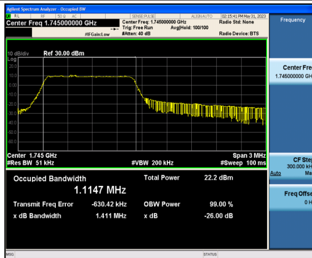
Band66-3MHz-16QAM-132322-6-0-Low-1.1147-1.411-PASS
