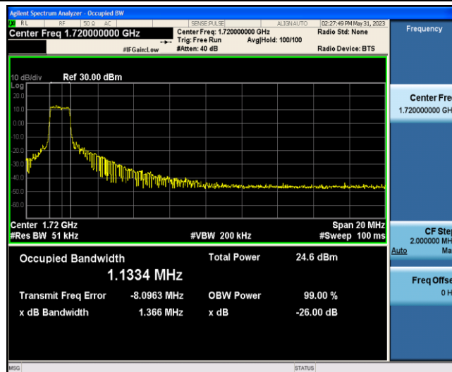
Band66-20MHz-QPSK-132072-6-0-Low-1.1334-1.366-PASS
