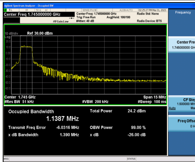
Band66-15MHz-16QAM-132322-6-0-Low-1.1387-1.390-PASS
