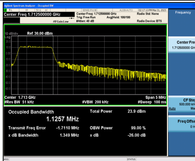
Band66-5MHz-QPSK-131997-6-0-Low-1.1257-1.349-PASS
