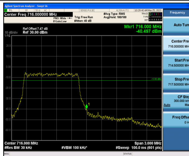
Band12-1.4MHz-16QAM-23173-6-0-High--40.50-PASS
