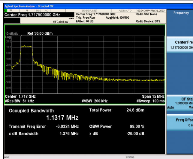
Band66-15MHz-QPSK-132047-6-0-Low-1.1317-1.376-PASS
