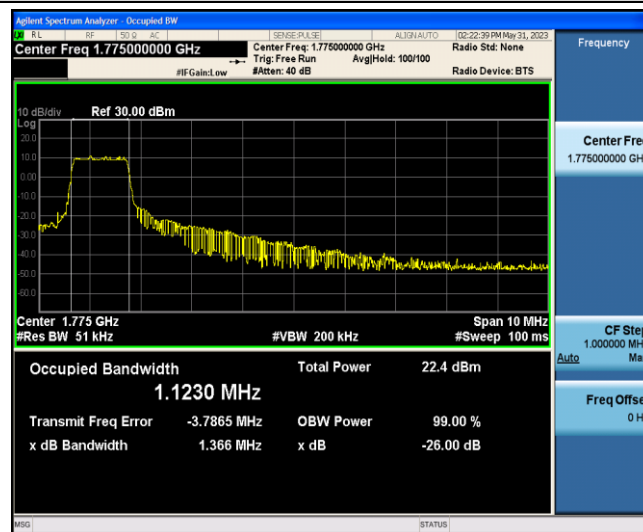
Band66-10MHz-16QAM-132622-6-0-Low-1.1230-1.366-PASS
