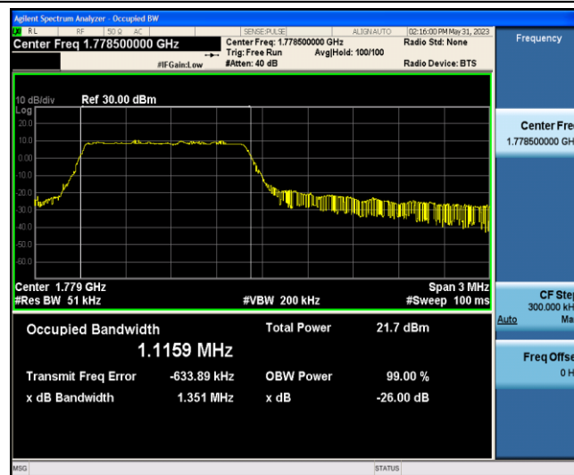
Band66-3MHz-QPSK-132657-6-0-Low-1.1159-1.351-PASS
