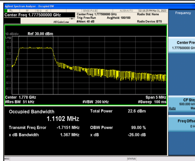
Band66-5MHz-QPSK-132647-6-0-Low-1.1102-1.367-PASS
