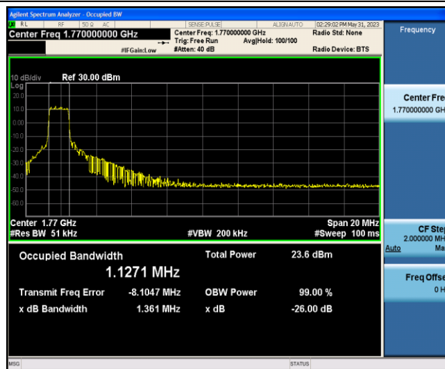
Band66-20MHz-QPSK-132572-6-0-Low-1.1271-1.361-PASS
