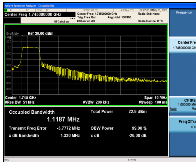
Band66-10MHz-16QAM-132322-6-0-Low-1.1187-1.330-PASS
