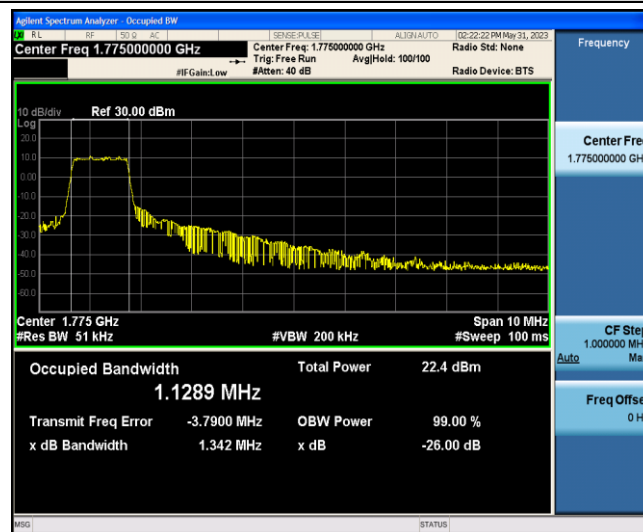
Band66-10MHz-QPSK-132622-6-0-Low-1.1289-1.342-PASS
