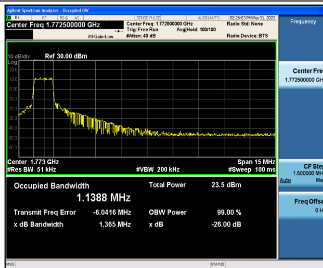
Band66-15MHz-16QAM-132597-6-0-Low-1.1388-1.365-PASS
