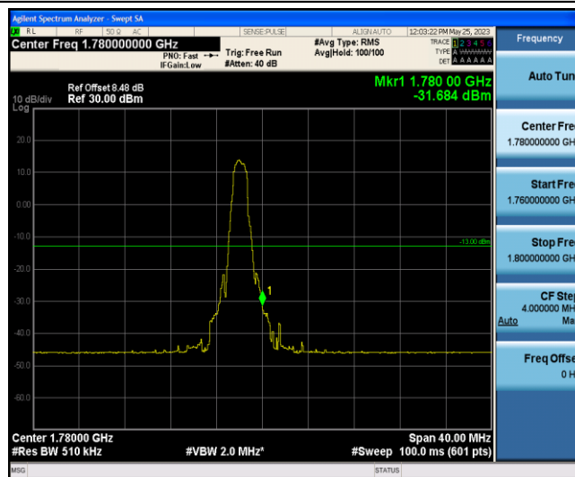
Band66-20MHz-QPSK-132572-6-0-High--31.68-PASS
