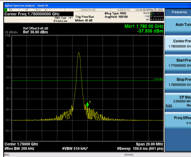
Band66-10MHz-16QAM-132622-1-5-High--37.94-PASS
