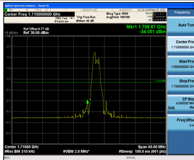
Band4-20MHz-16QAM-20050-6-0-Low--34.05-PASS
