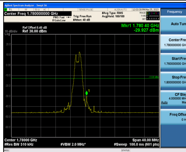
Band66-20MHz-16QAM-132572-6-0-High--29.93-PASS
