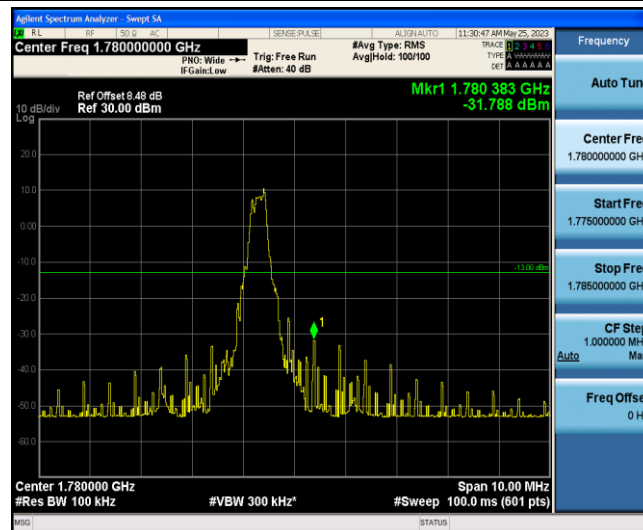
Band66-5MHz-QPSK-132647-1-5-High--31.79-PASS
