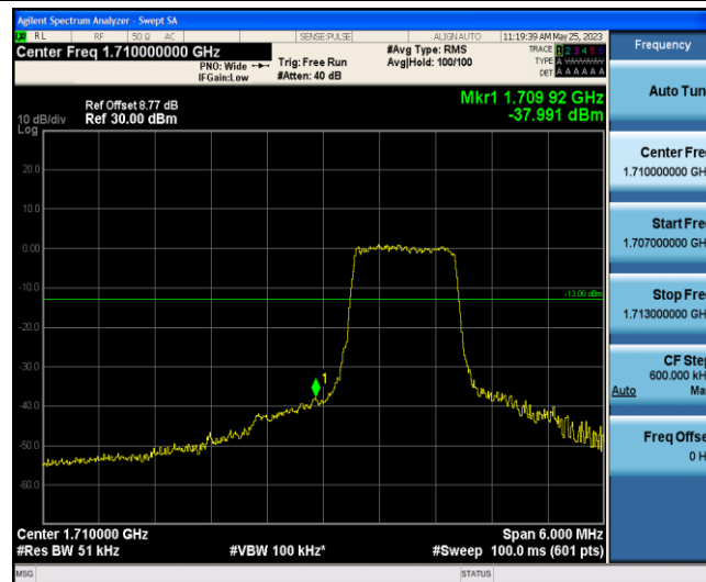
Band66-3MHz-QPSK-131987-6-0-Low--37.99-PASS
