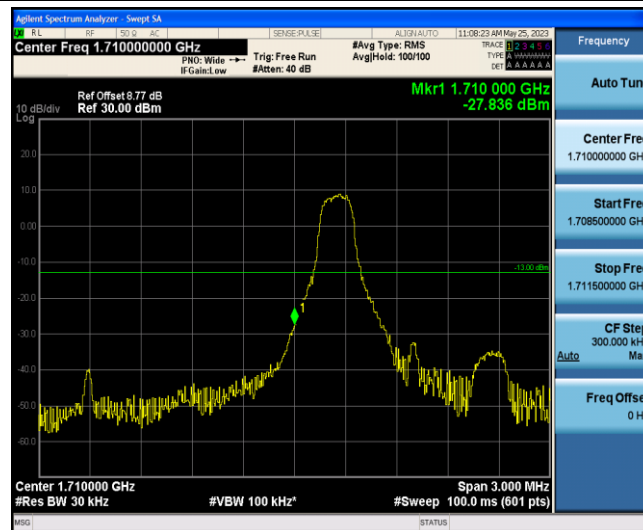
Band66-1.4MHz-QPSK-131979-1-0-Low--27.84-PASS
