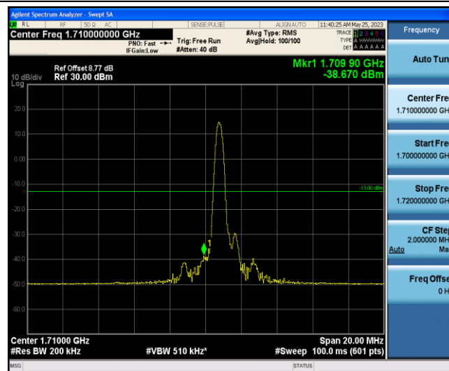
Band66-10MHz-16QAM-132022-1-0-Low--38.67-PASS
