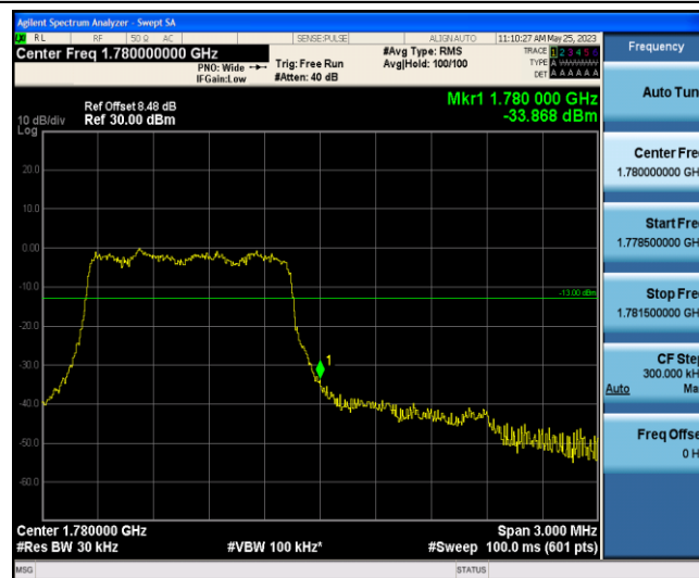
Band66-1.4MHz-16QAM-132665-6-0-High--33.87-PASS
