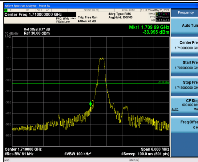
Band66-3MHz-QPSK-131987-1-0-Low--34.00-PASS
