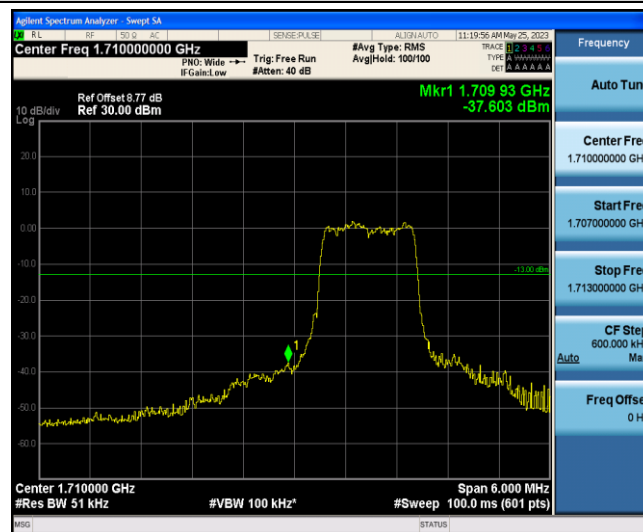
Band66-3MHz-16QAM-131987-6-0-Low--37.60-PASS
