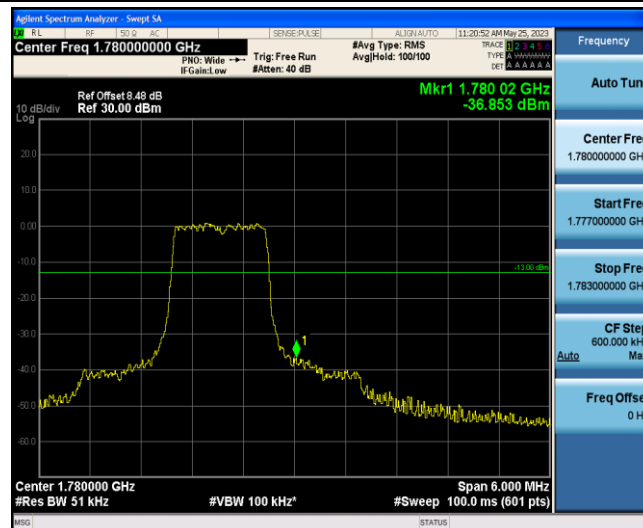
Band66-3MHz-QPSK-132657-6-0-High--36.85-PASS
