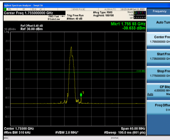
Band4-20MHz-16QAM-20300-1-5-High--39.63-PASS
