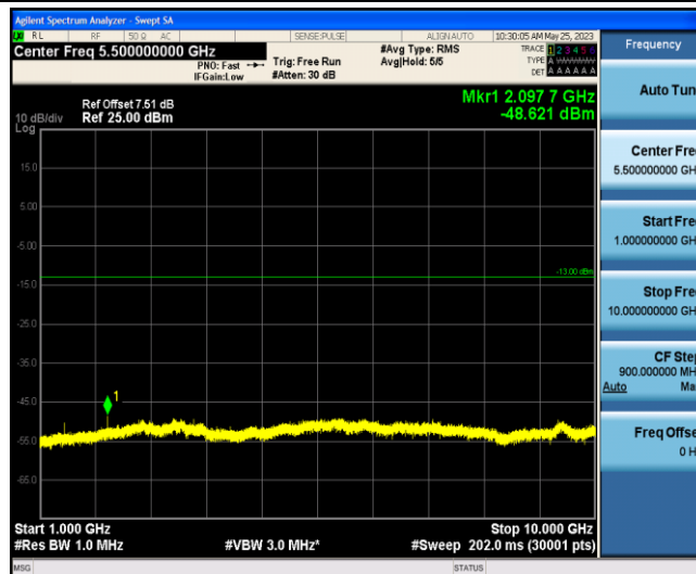
Band12-1.4MHz-QPSK-23017-1-0-Low-1000-10000--48.62-PASS
