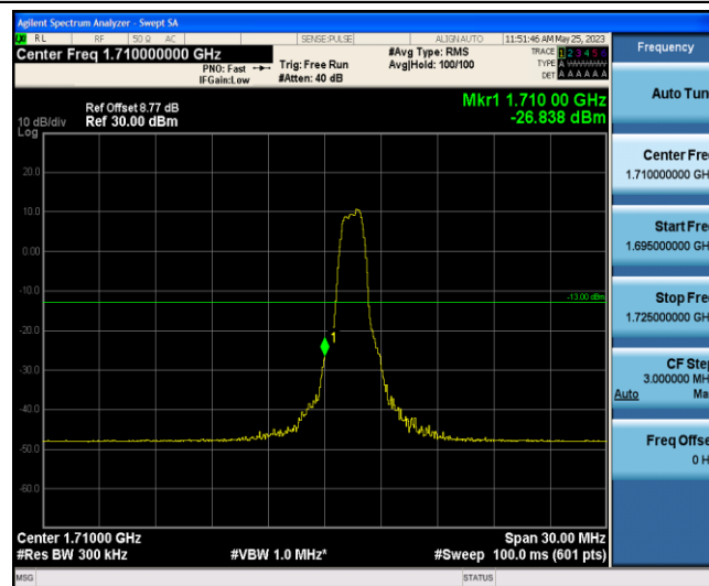
Band66-15MHz-16QAM-132047-6-0-Low--26.84-PASS
