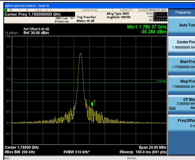
Band66-10MHz-QPSK-132622-1-5-High--35.28-PASS
