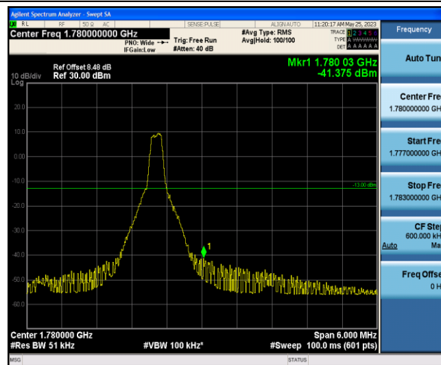
Band66-3MHz-QPSK-132657-1-5-High--41.37-PASS
