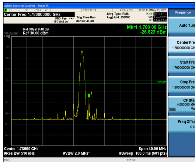
Band66-20MHz-QPSK-132572-1-5-High--26.82-PASS
