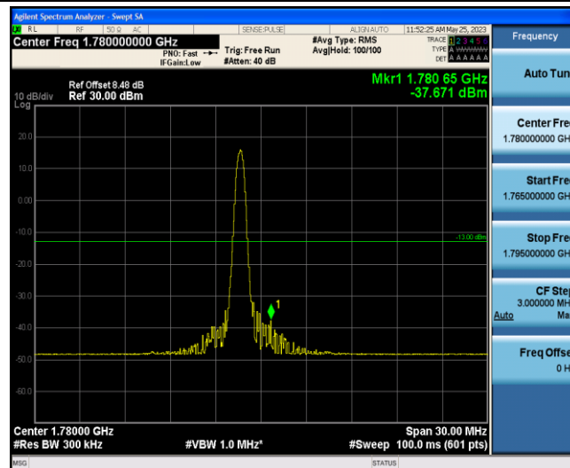
Band66-15MHz-16QAM-132597-1-5-High--37.67-PASS
