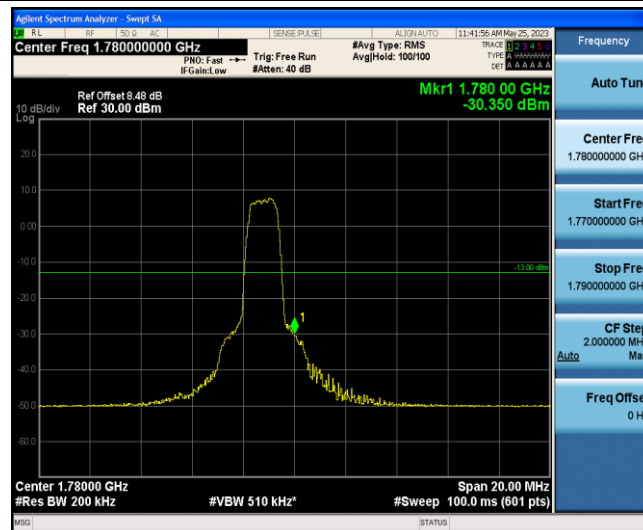
Band66-10MHz-QPSK-132622-6-0-High--30.35-PASS
