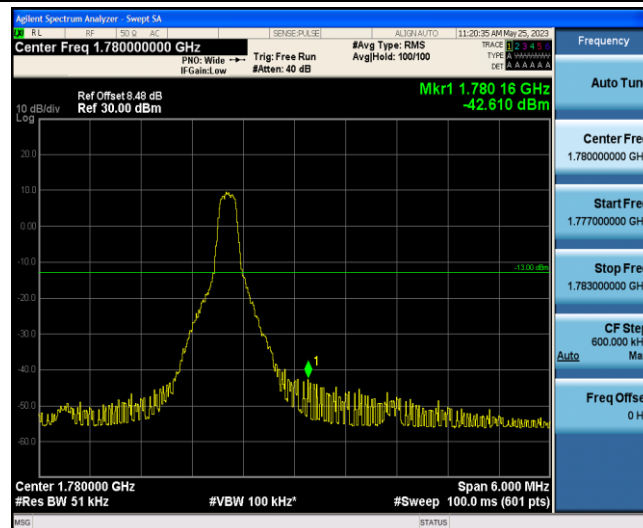
Band66-3MHz-16QAM-132657-1-5-High--42.61-PASS
