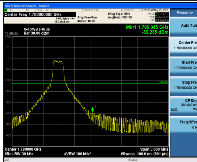
Band66-1.4MHz-QPSK-132665-1-5-High--39.24-PASS
