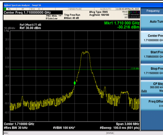
Band66-1.4MHz-16QAM-131979-1-0-Low--30.22-PASS
