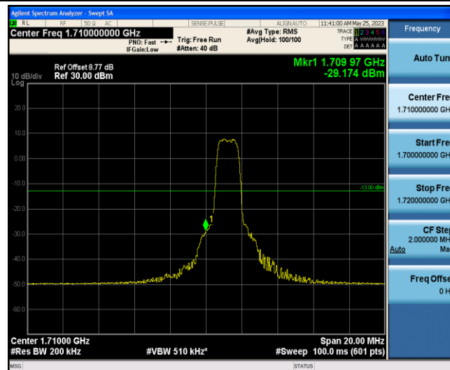
Band66-10MHz-16QAM-132022-6-0-Low--29.17-PASS
