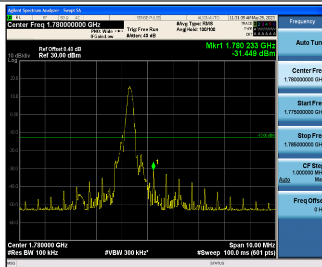
Band66-5MHz-16QAM-132647-1-5-High--31.45-PASS
