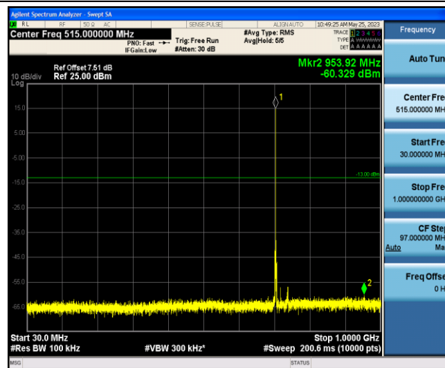
Band12-5MHz-16QAM-23155-1-0-Low-30-1000--60.33-PASS
