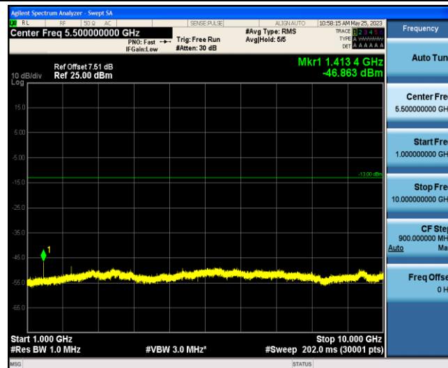
Band12-10MHz-QPSK-23130-1-0-Low-1000-10000--46.86-PASS
