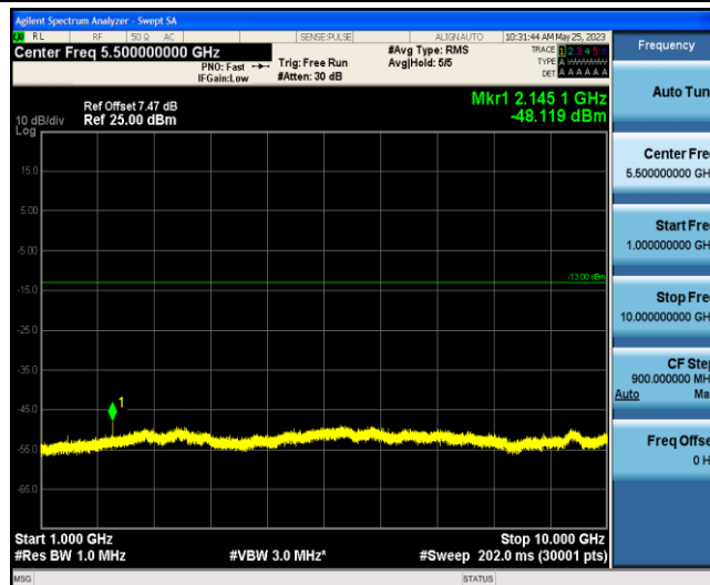
Band12-1.4MHz-16QAM-23173-1-0-Low-1000-10000--48.12-PASS
