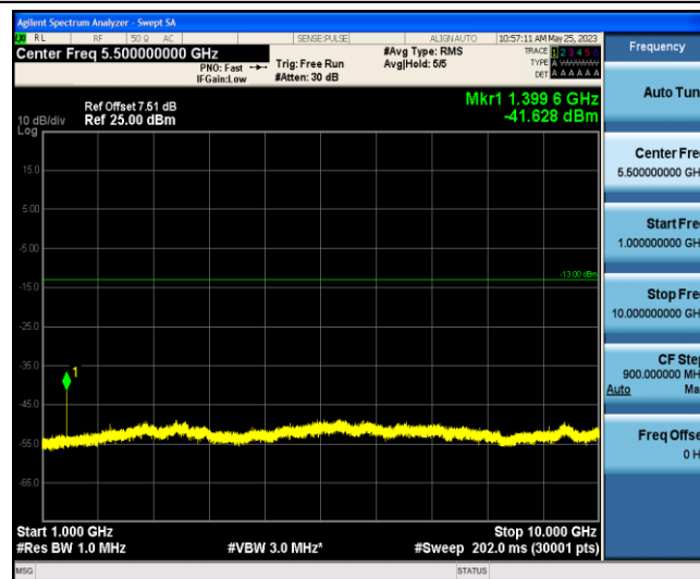
Band12-10MHz-16QAM-23060-1-0-Low-1000-10000--41.63-PASS
