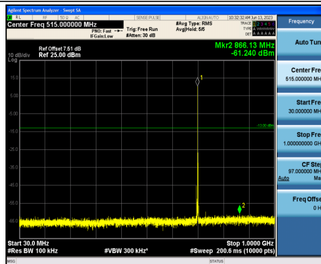
Band12-1.4MHz-16QAM-23095-1-0-Low-30-1000--61.24-PASS
