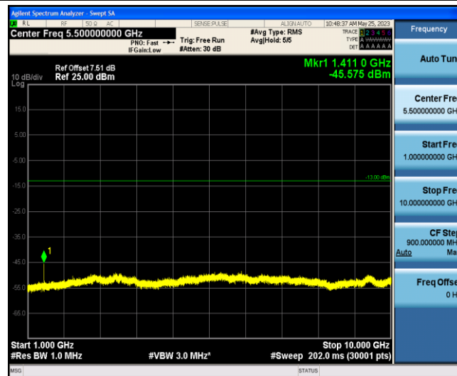
Band12-5MHz-QPSK-23095-1-0-Low-1000-10000--45.58-PASS
