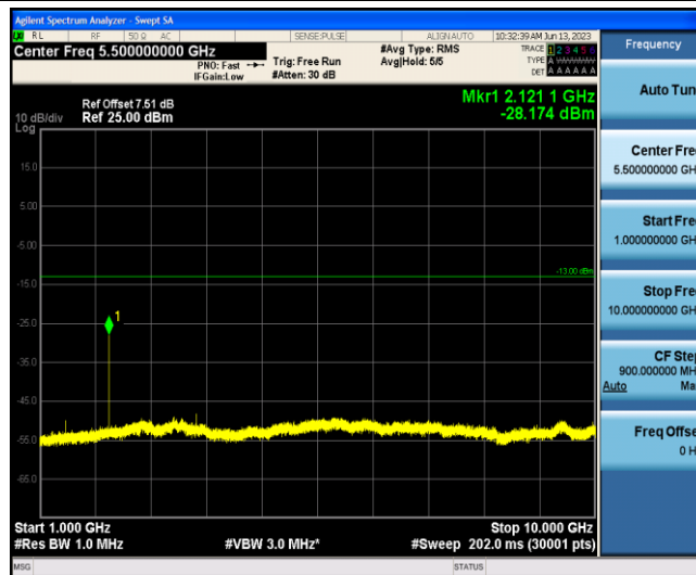
Band12-1.4MHz-16QAM-23095-1-0-Low-1000-10000--28.17-PASS
