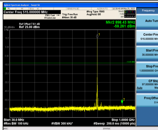
Band12-3MHz-16QAM-23095-1-0-Low-30-1000--59.26-PASS
