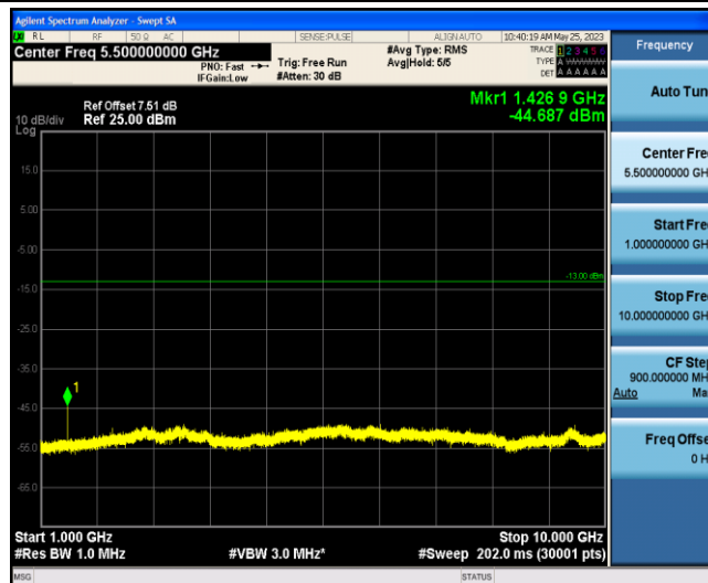
Band12-3MHz-QPSK-23165-1-0-Low-1000-10000--44.69-PASS
