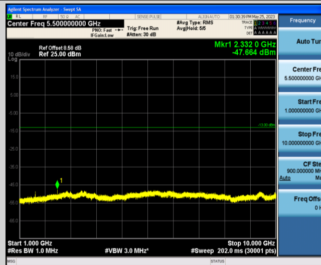
Band13-5MHz-QPSK-23205-1-0-Low-1000-10000--47.66-PASS
