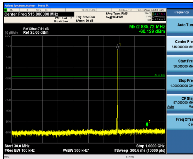
Band12-3MHz-16QAM-23025-1-0-Low-30-1000--60.13-PASS
