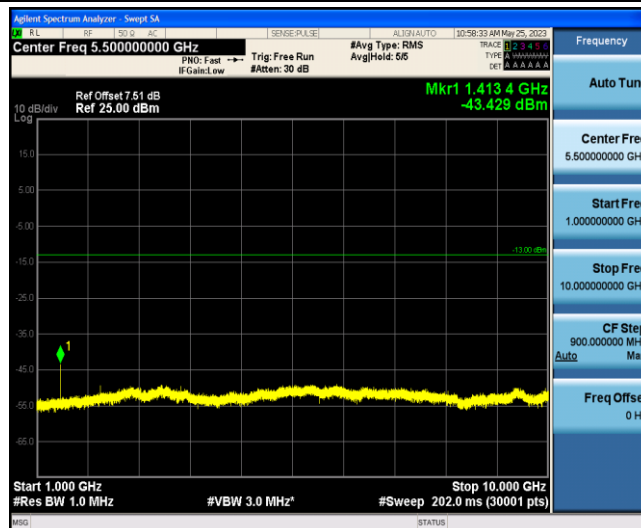
Band12-10MHz-16QAM-23130-1-0-Low-1000-10000--43.43-PASS
