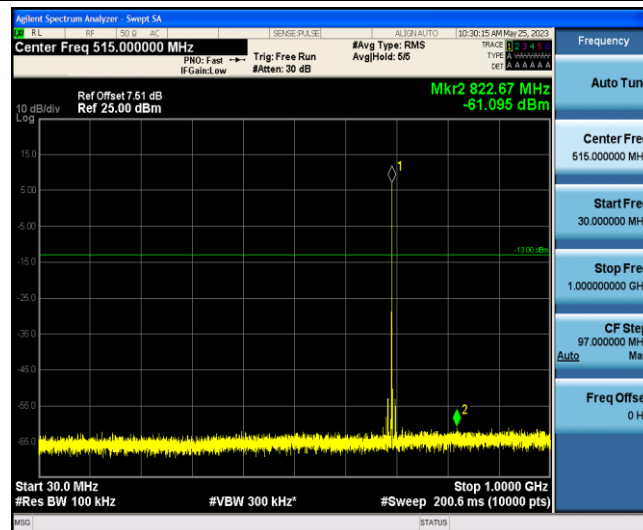
Band12-1.4MHz-16QAM-23017-1-0-Low-30-1000--61.1-PASS
