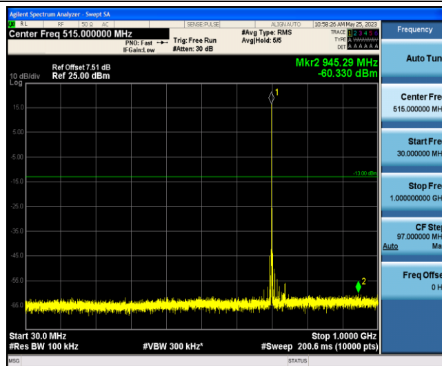
Band12-10MHz-16QAM-23130-1-0-Low-30-1000--60.33-PASS
