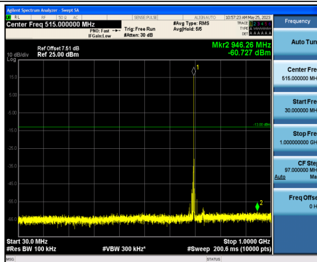
Band12-10MHz-QPSK-23095-1-0-Low-30-1000--60.73-PASS
