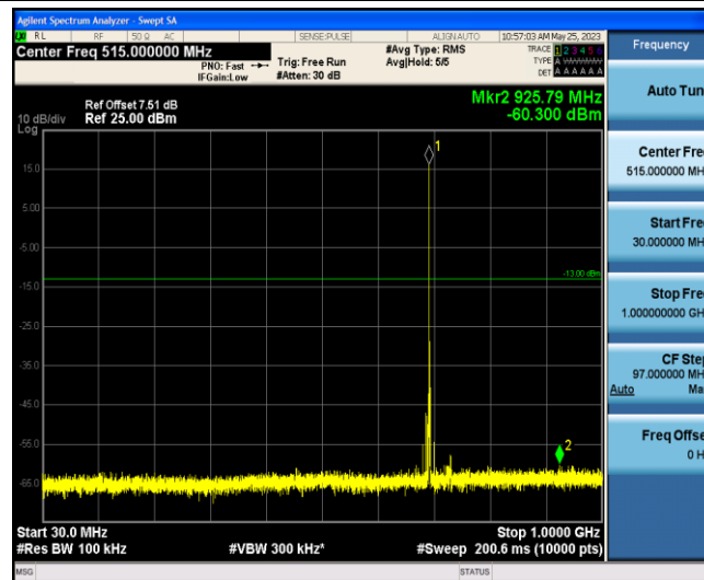
Band12-10MHz-16QAM-23060-1-0-Low-30-1000--60.3-PASS
