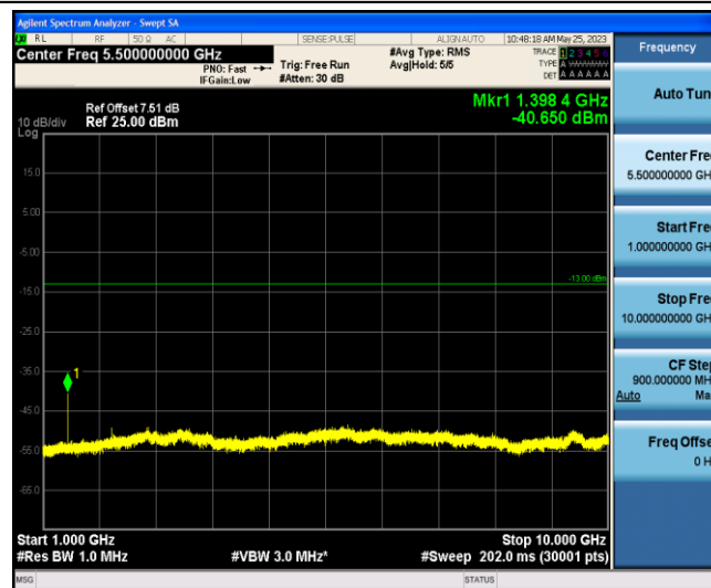
Band12-5MHz-16QAM-23035-1-0-Low-1000-10000--40.65-PASS
