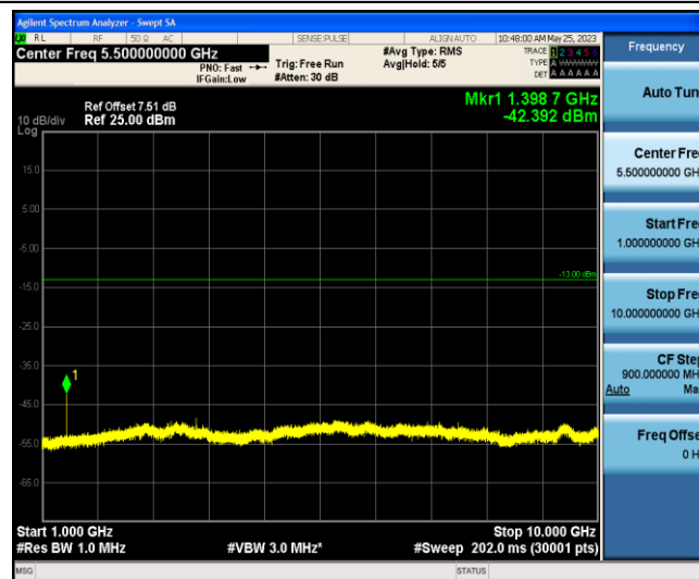
Band12-5MHz-QPSK-23035-1-0-Low-1000-10000--42.39-PASS
