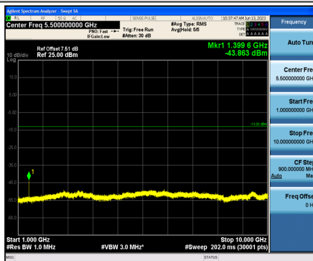
Band12-10MHz-QPSK-23060-1-0-Low-1000-10000--43.86-PASS
