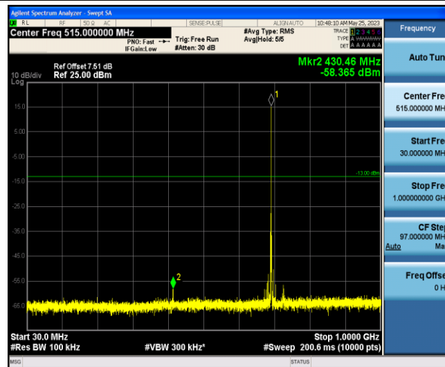
Band12-5MHz-16QAM-23035-1-0-Low-30-1000--58.37-PASS
