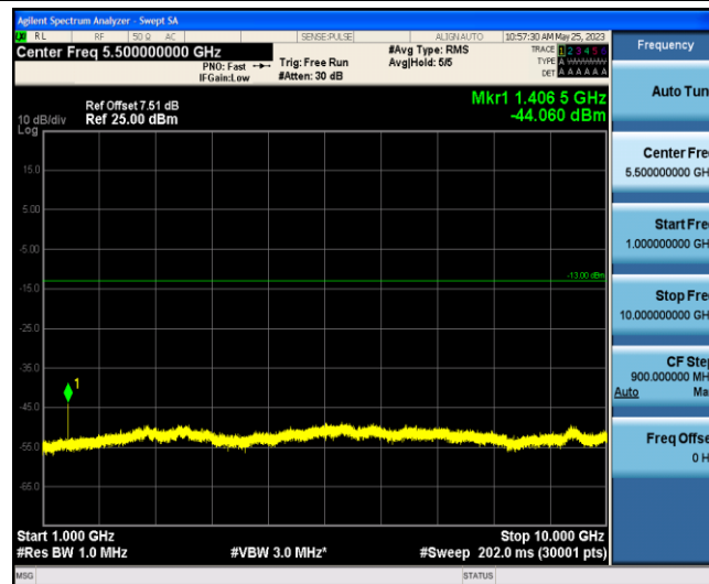
Band12-10MHz-QPSK-23095-1-0-Low-1000-10000--44.06-PASS
