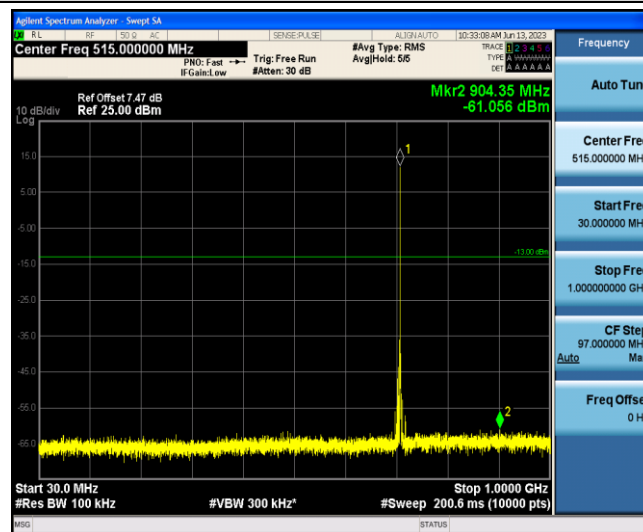
Band12-1.4MHz-QPSK-23173-1-0-Low-30-1000--61.06-PASS
