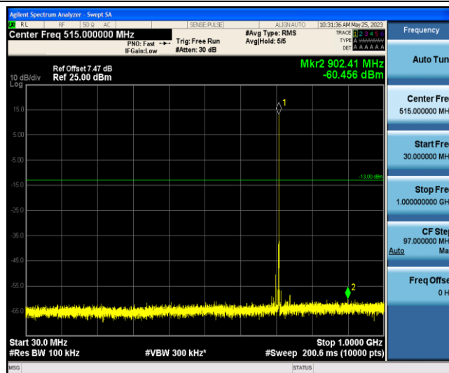
Band12-1.4MHz-16QAM-23173-1-0-Low-30-1000--60.46-PASS
