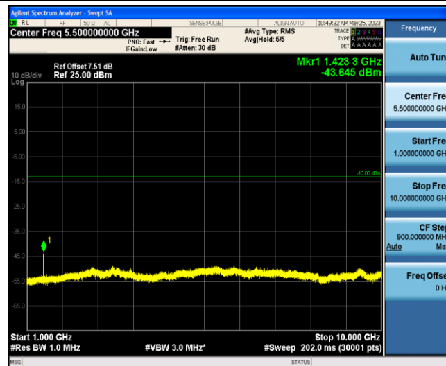
Band12-5MHz-16QAM-23155-1-0-Low-1000-10000--43.65-PASS
