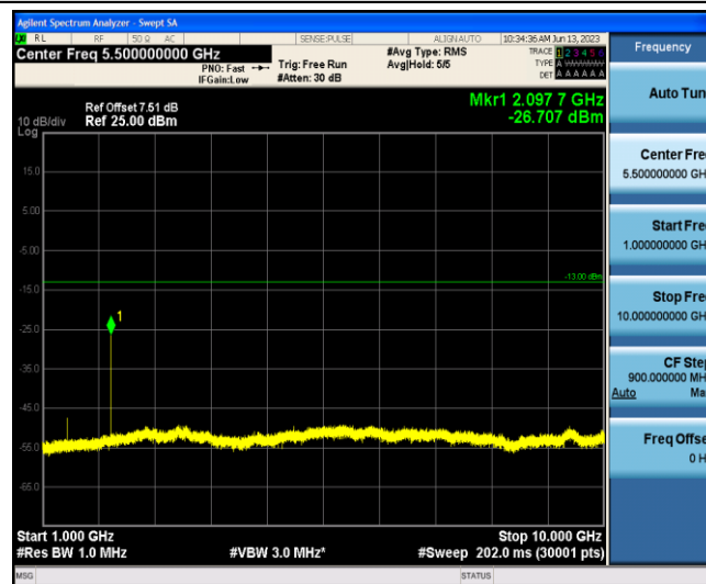
Band12-3MHz-16QAM-23025-1-0-Low-1000-10000--26.71-PASS
