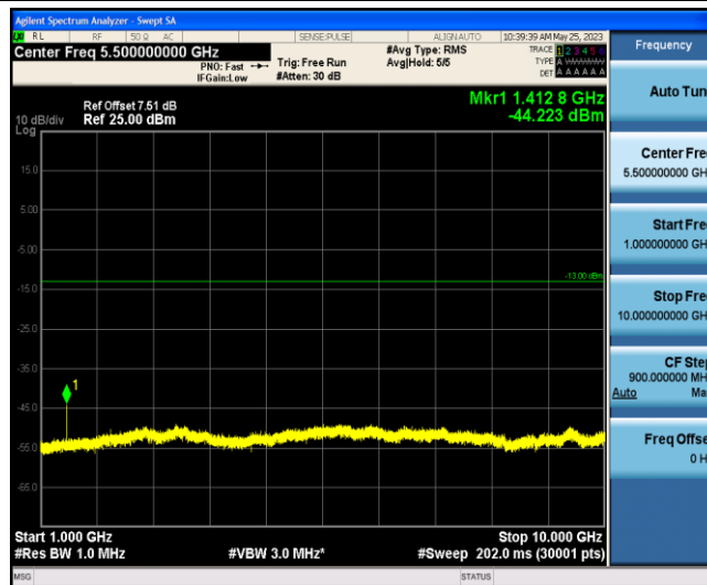
Band12-3MHz-QPSK-23095-1-0-Low-1000-10000--44.22-PASS
