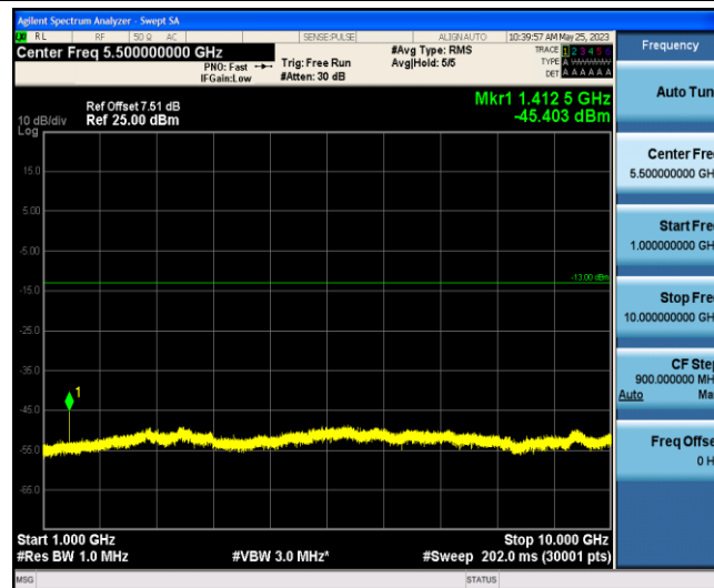
Band12-3MHz-16QAM-23095-1-0-Low-1000-10000--45.4-PASS
