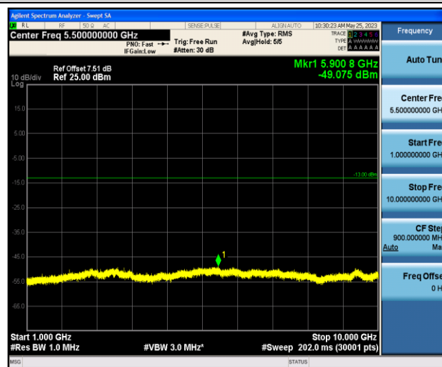
Band12-1.4MHz-16QAM-23017-1-0-Low-1000-10000--49.08-PASS
