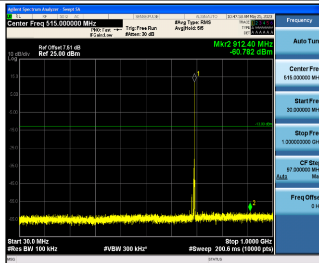
Band12-5MHz-QPSK-23035-1-0-Low-30-1000--60.78-PASS
