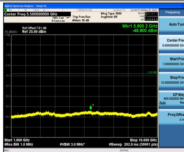
Band12-3MHz-16QAM-23165-1-0-Low-1000-10000--48.8-PASS
