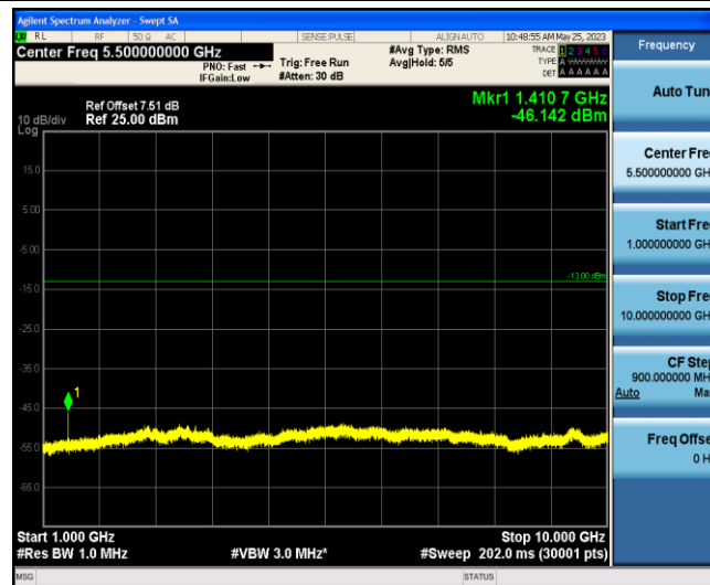
Band12-5MHz-16QAM-23095-1-0-Low-1000-10000--46.14-PASS
