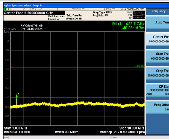
Band12-5MHz-QPSK-23155-1-0-Low-1000-10000--46.83-PASS
