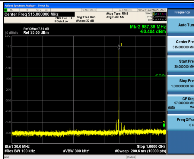
Band12-10MHz-16QAM-23095-1-0-Low-30-1000--60.4-PASS
