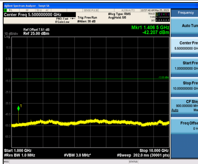
Band12-10MHz-16QAM-23095-1-0-Low-1000-10000--42.21-PASS
