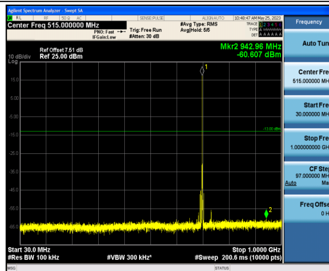
Band12-5MHz-16QAM-23095-1-0-Low-30-1000--60.61-PASS
