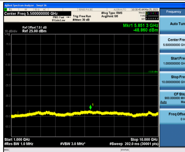
Band12-1.4MHz-QPSK-23095-1-0-Low-1000-10000--48.86-PASS
