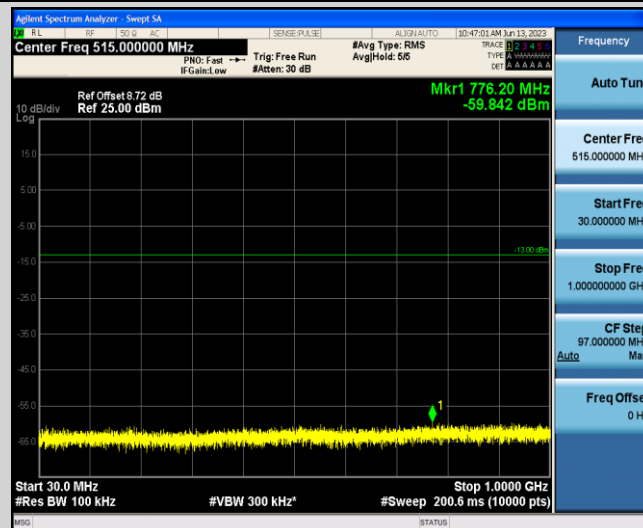
Band2-5MHz-16QAM-18625-1-0-Low-30-1000--59.84-PASS
