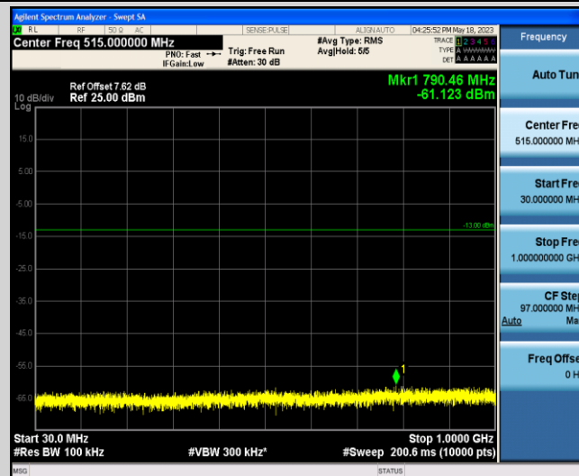
Band2-1.4MHz-16QAM-18607-1-0-Low-30-1000--61.12-PASS
