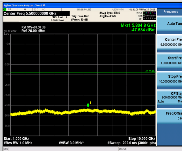
Band13-5MHz-16QAM-23205-1-0-Low-1000-10000--47.63-PASS
