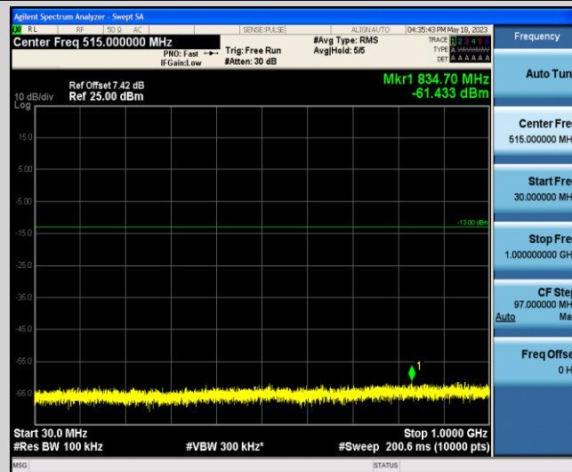
Band2-3MHz-16QAM-19185-1-0-Low-30-1000--61.43-PASS
