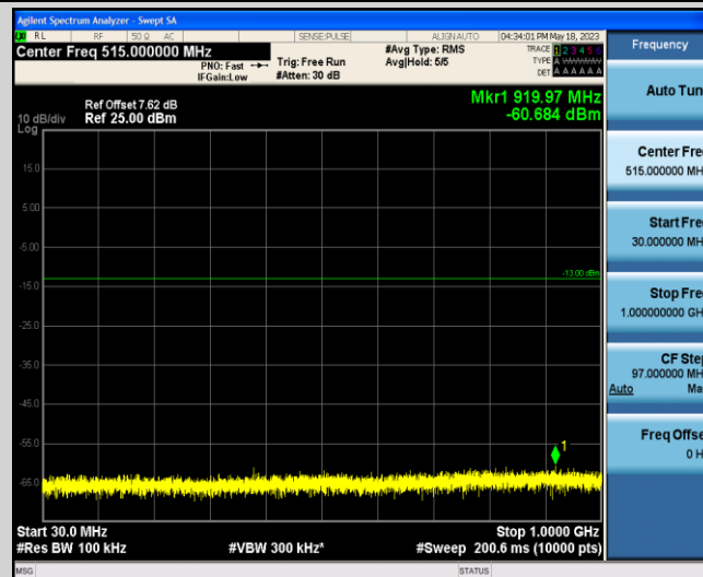
Band2-3MHz-QPSK-18615-1-0-Low-30-1000--60.68-PASS
