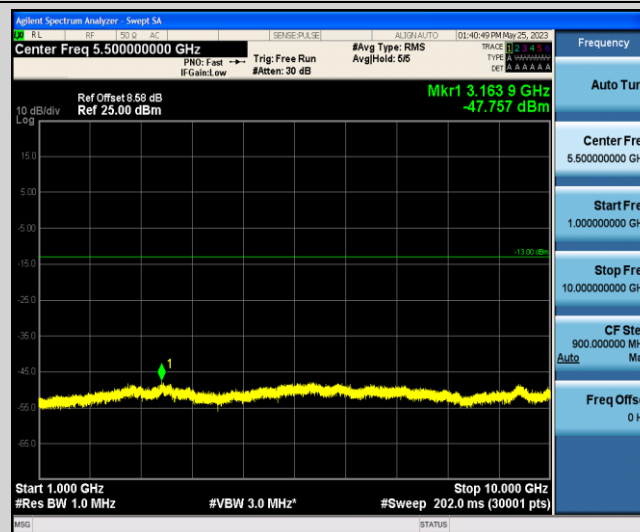
Band13-10MHz-16QAM-23230-1-0-Low-1000-10000--47.76-PASS
