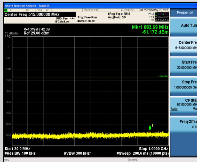
Band2-3MHz-QPSK-19185-1-0-Low-30-1000--61.17-PASS
