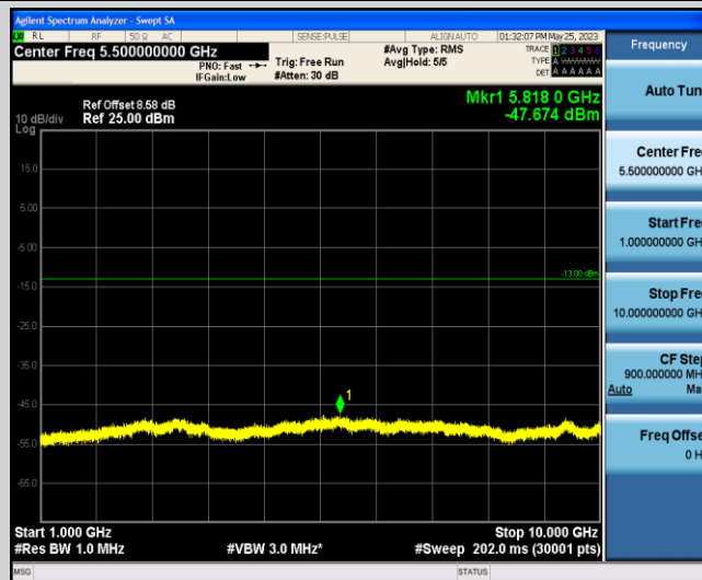
Band13-5MHz-16QAM-23230-1-0-Low-1000-10000--47.67-PASS
