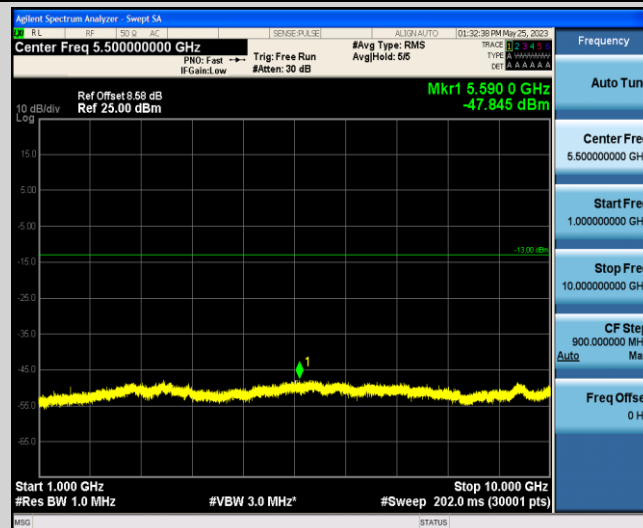
Band13-5MHz-QPSK-23255-1-0-Low-1000-10000--47.85-PASS
