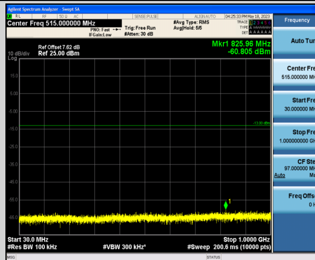
Band2-1.4MHz-QPSK-18607-1-0-Low-30-1000--60.81-PASS
