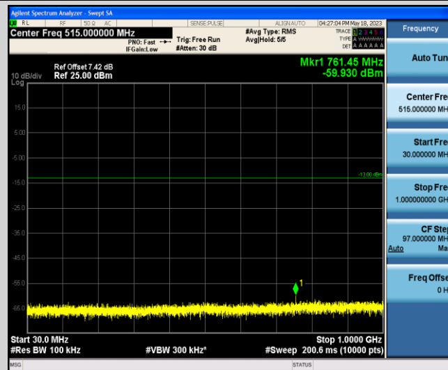
Band2-1.4MHz-QPSK-19193-1-0-Low-30-1000--59.93-PASS
