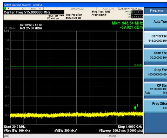
Band2-Stand-Alone-NaN-QPSK-18601-1@0-3.75kHz-30-1000--59.92--13-PASS
