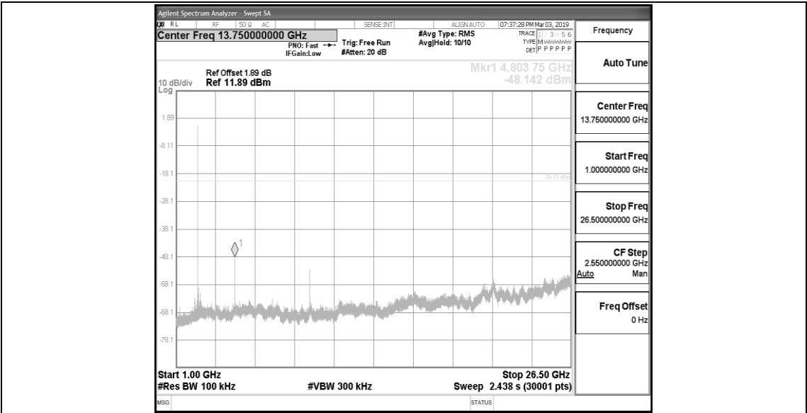
DH1_Ant1_2441_0~Reference
