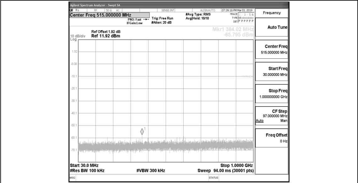
DH1_Ant1_2441_30~1000
