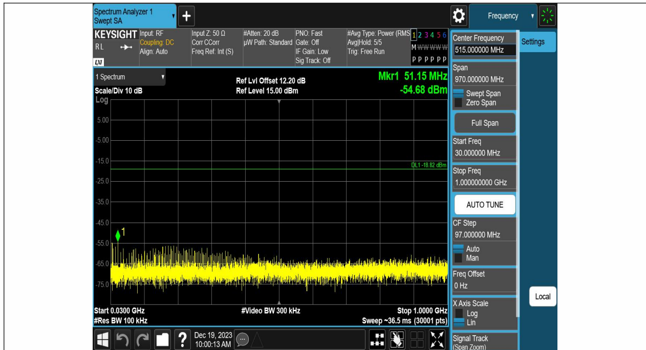
BLE_1M-Ant1-2440-30~1000-PASS
