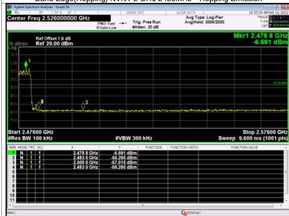
Band Edge(Hopping) NVNT 2-DH1 2480MHz Hopping Emission
