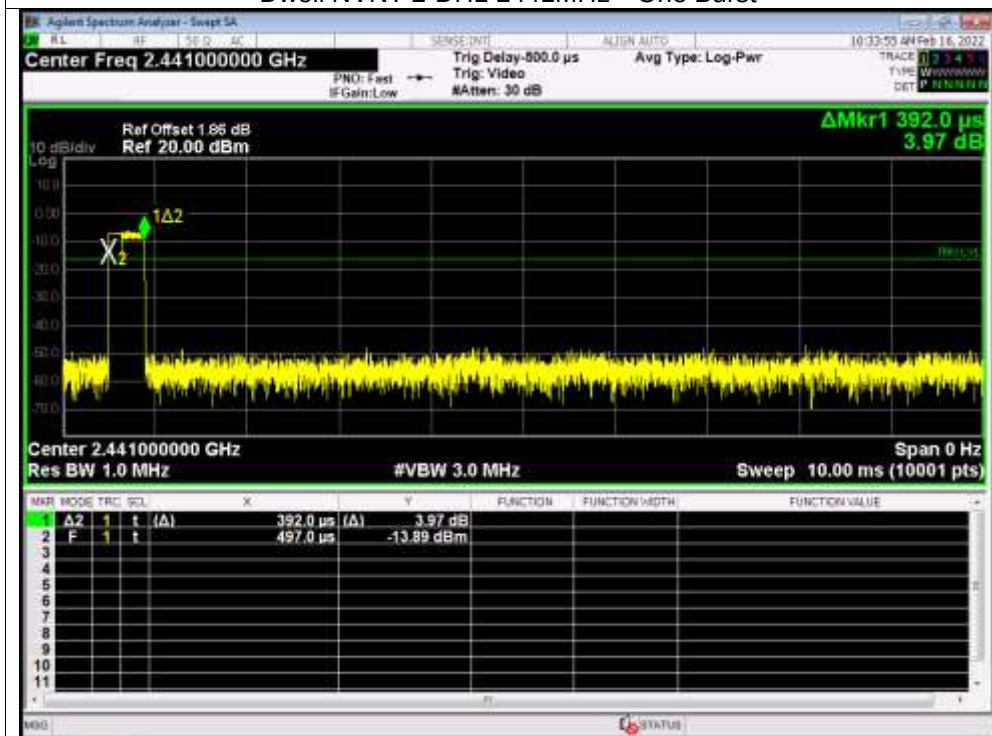
Dwell NVNT 2-DH1 2441MHz One Burst
