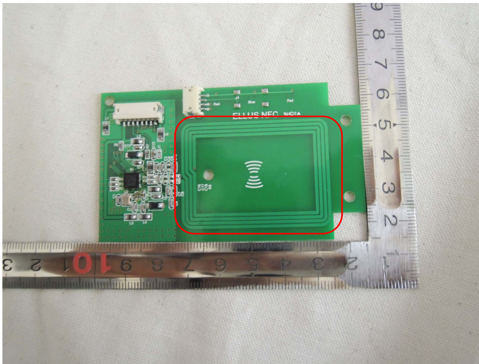
Antenna part
