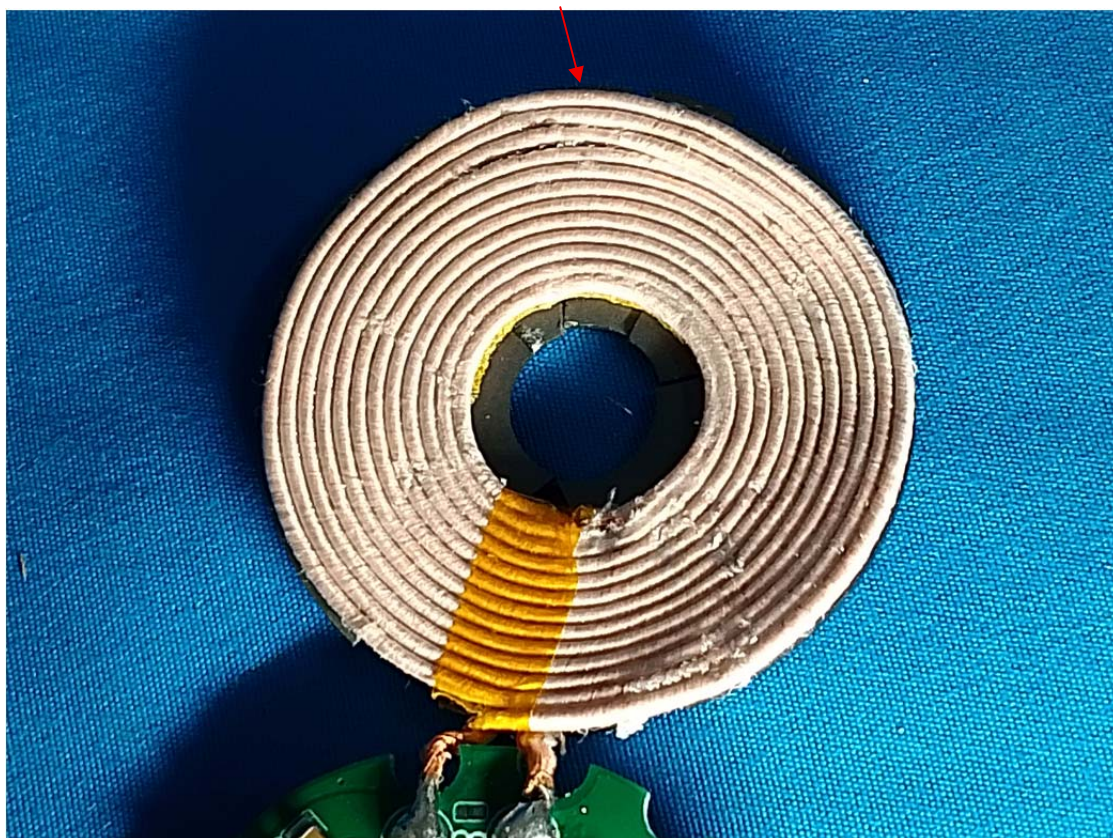
WPT Coil
