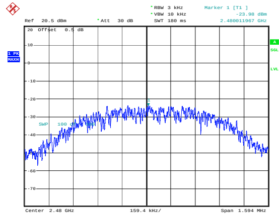
BLE_1M_High_Channel
