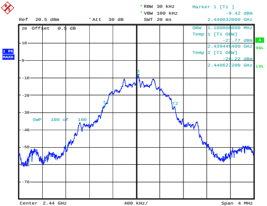
BLE_1M_Middle_Channel
