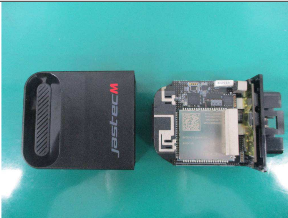
View of Board (1)
