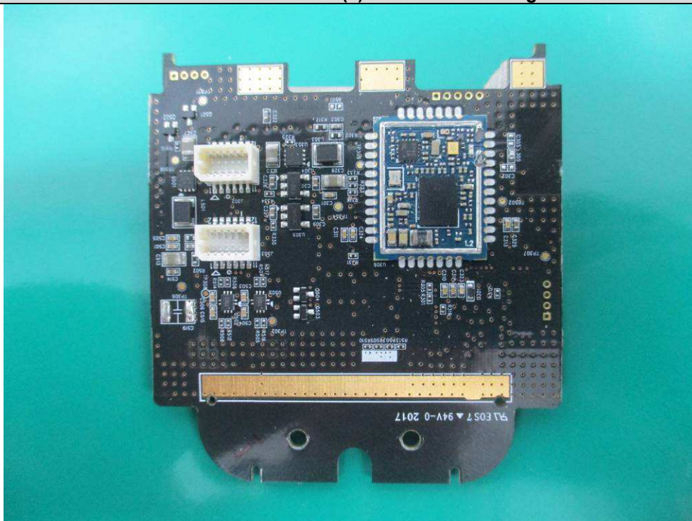
Rear View of Board (2) - Without Shielding
