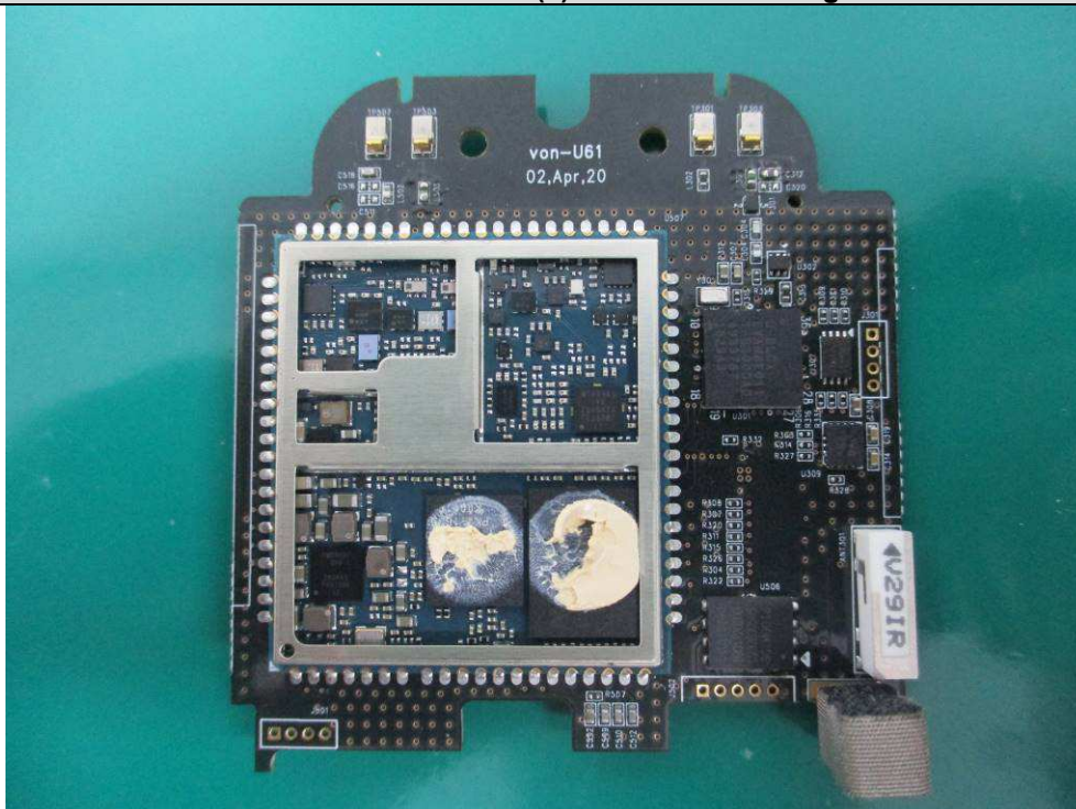
Front View of Board (2) - Without Shielding
