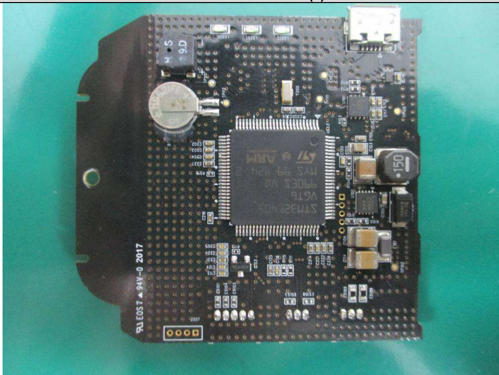
Rear View of Board (3)
