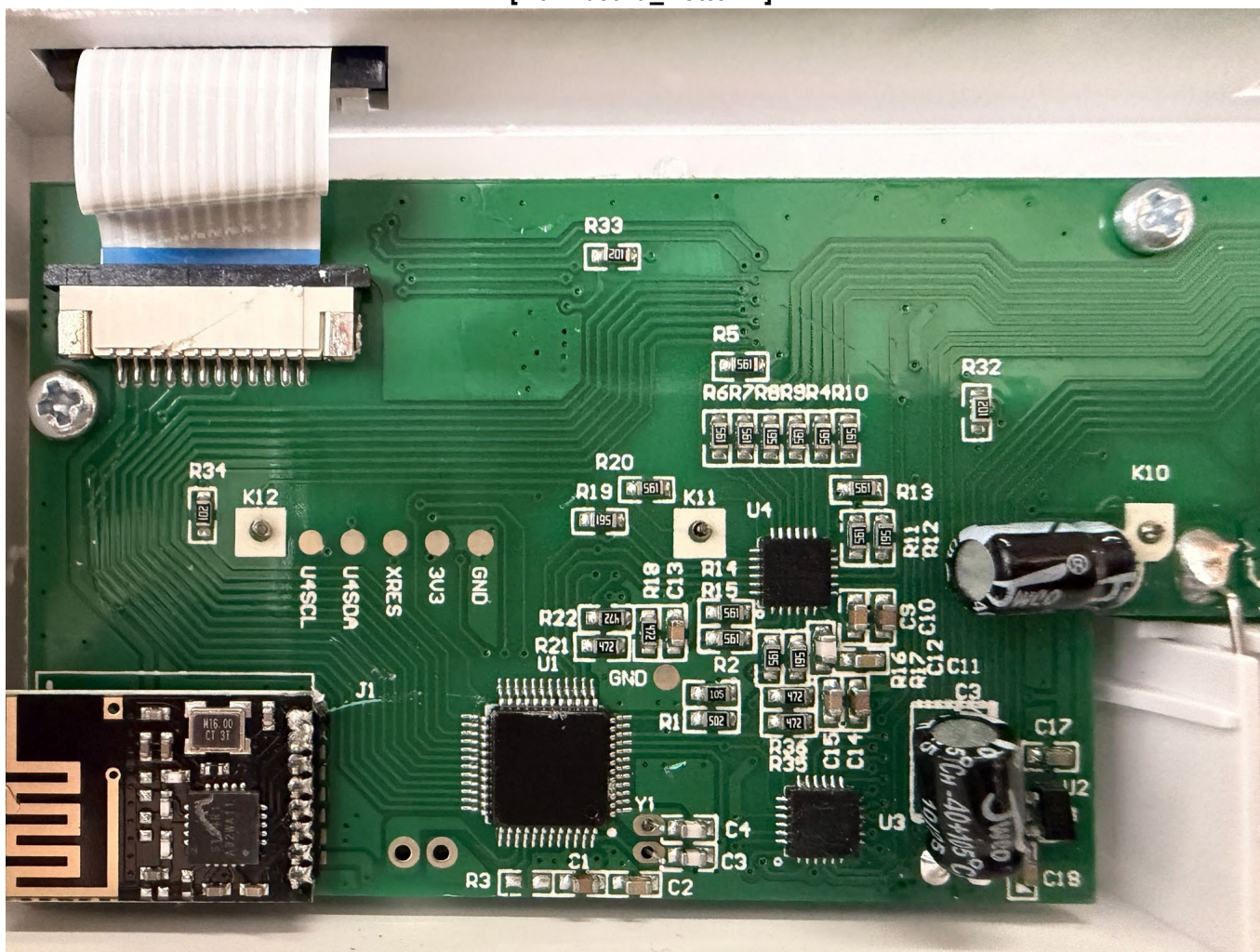
[Main board_Bottom2]
