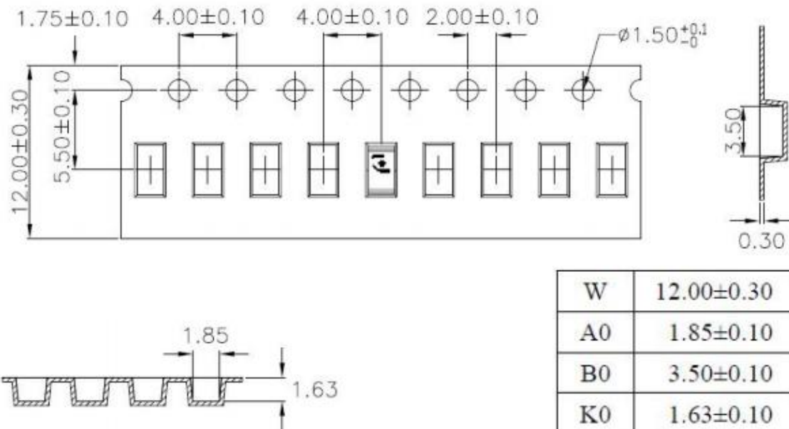
a. Tape Drawing & Tape Dimensions (unit: mm)
