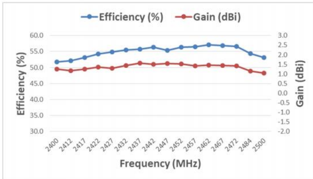
7-3. 3D Efficiency vs. Frequency
