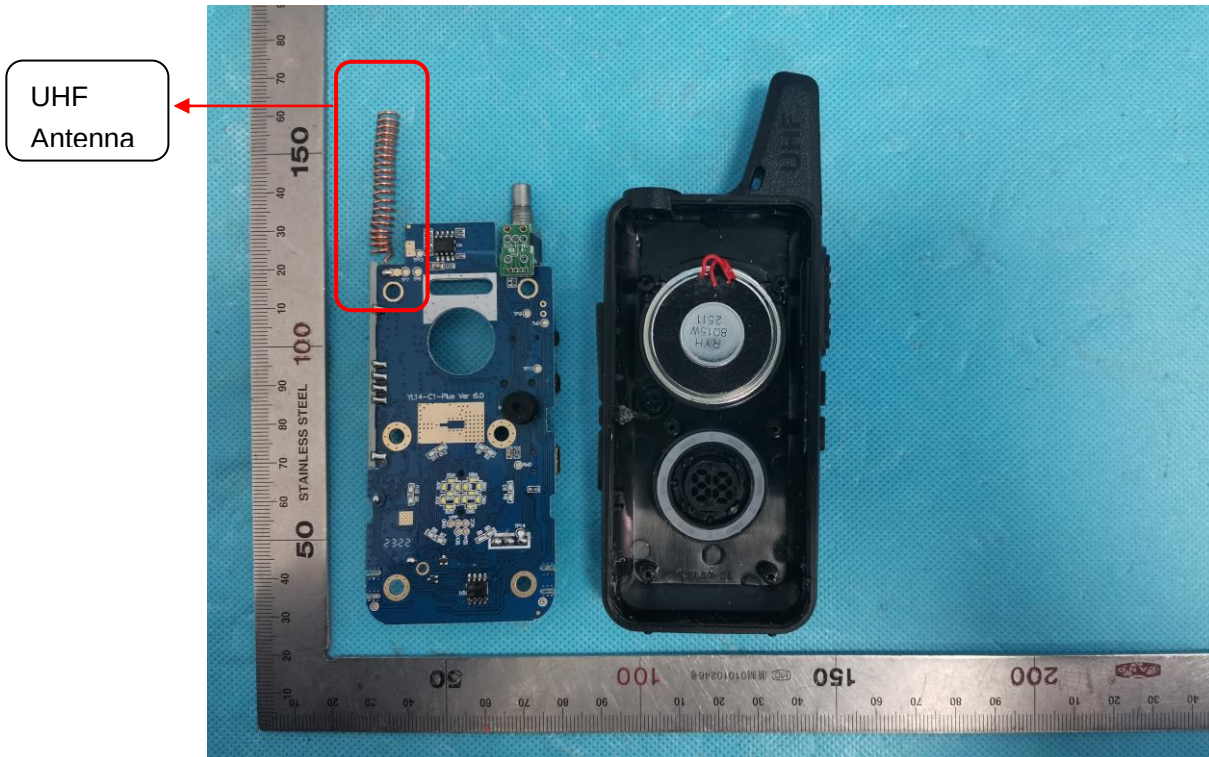
INTERNAL VIEW OF EUT (FIGURE 1)
