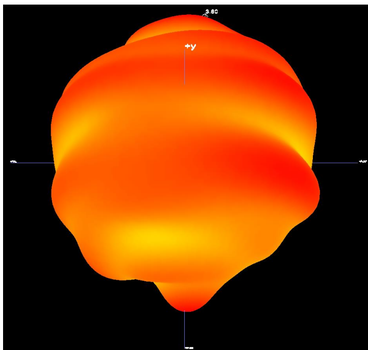
B1.2 3D Pattern for 2440MHz
