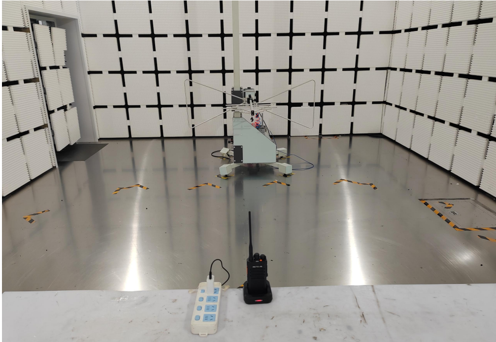
Radiated Emissions Measurement (Below 1GHz)
