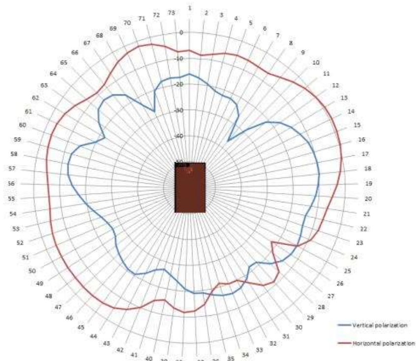
Figure 21: Radiation pattern, PCB horizontal, single layer IFA
