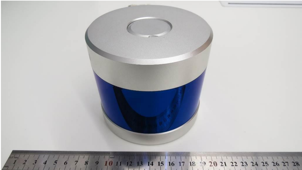
(11) EUT Photo (Pandar20A, Pandar20B)
