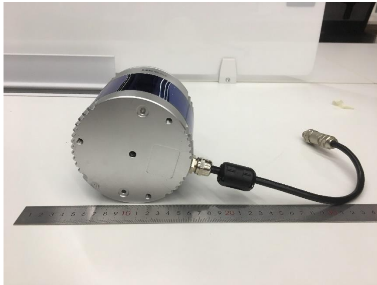
(3) EUT Photo (Pandar64)
