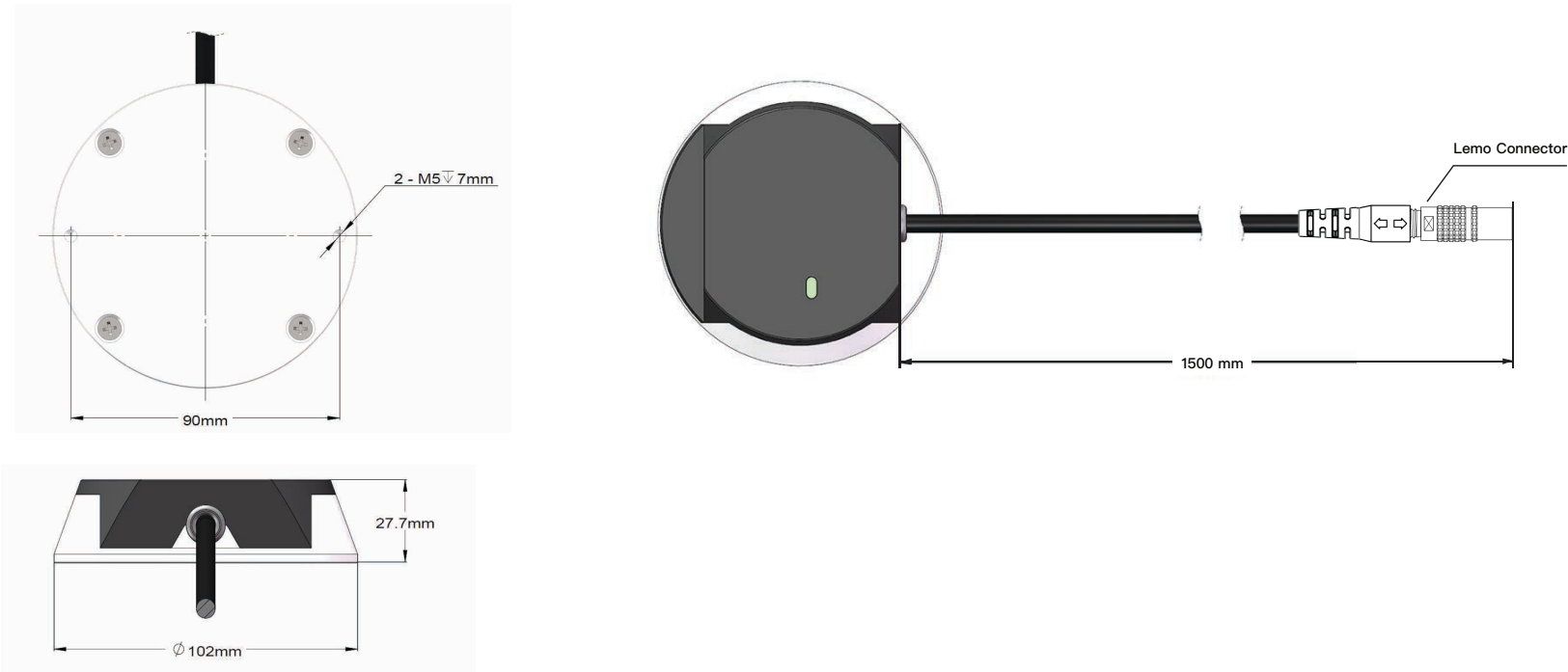
Figure 2.6 Connecting Box
