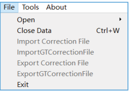
Figure VII.5 File Menu
