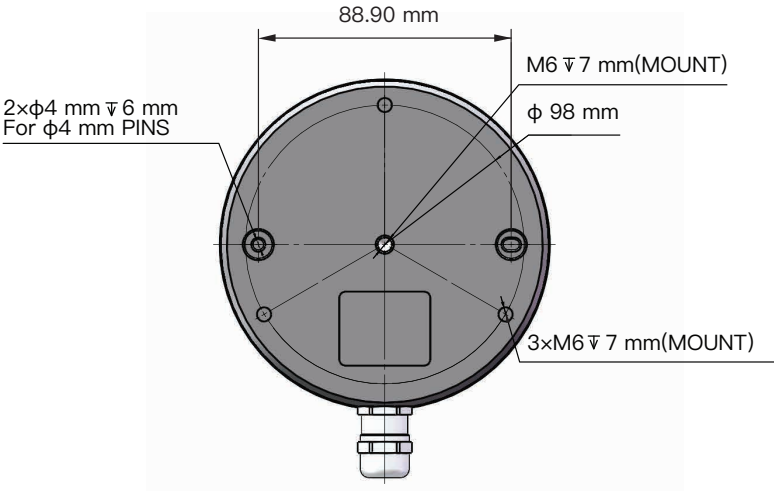
Figure 2.2 Pandar20A/B Mounting Base
