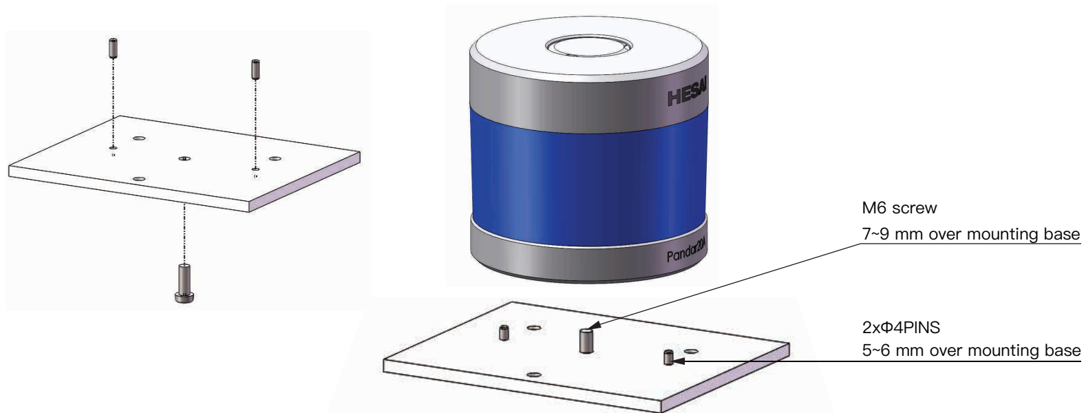
Figure 2.3 Diagram of Quick Installation
