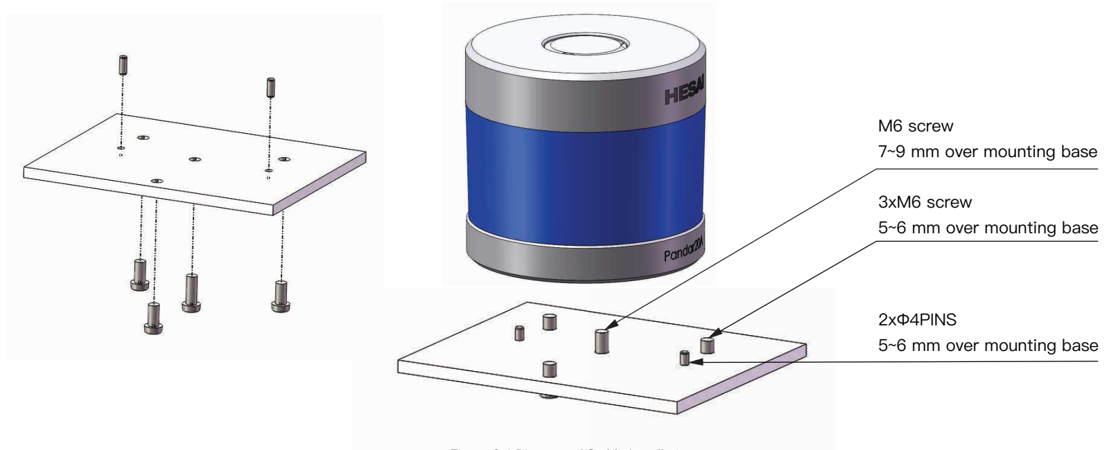
Figure 2.4 Diagram of Stable Installation
