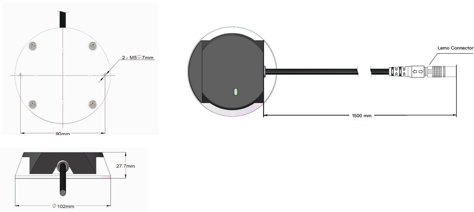
Figure 2.6 Connecting Box
