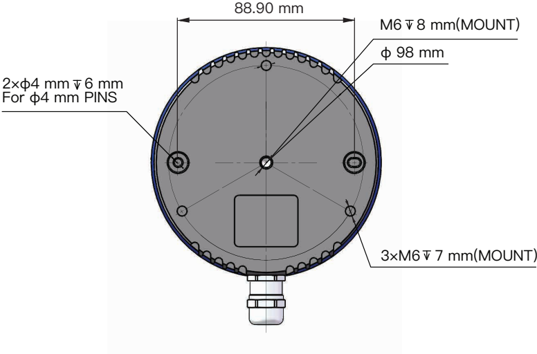
Figure 2.2 Pandar64 Mounting Base
