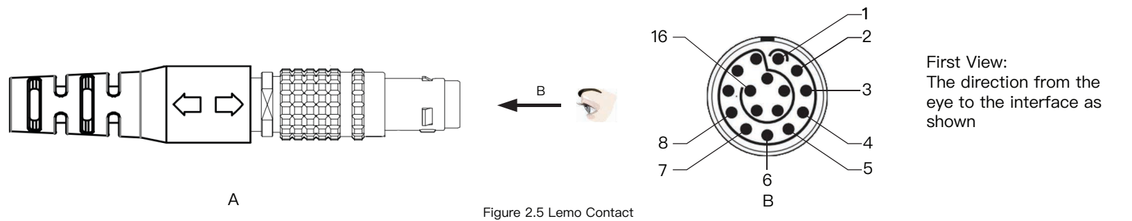
Figure 2.5 Lemo Contact
