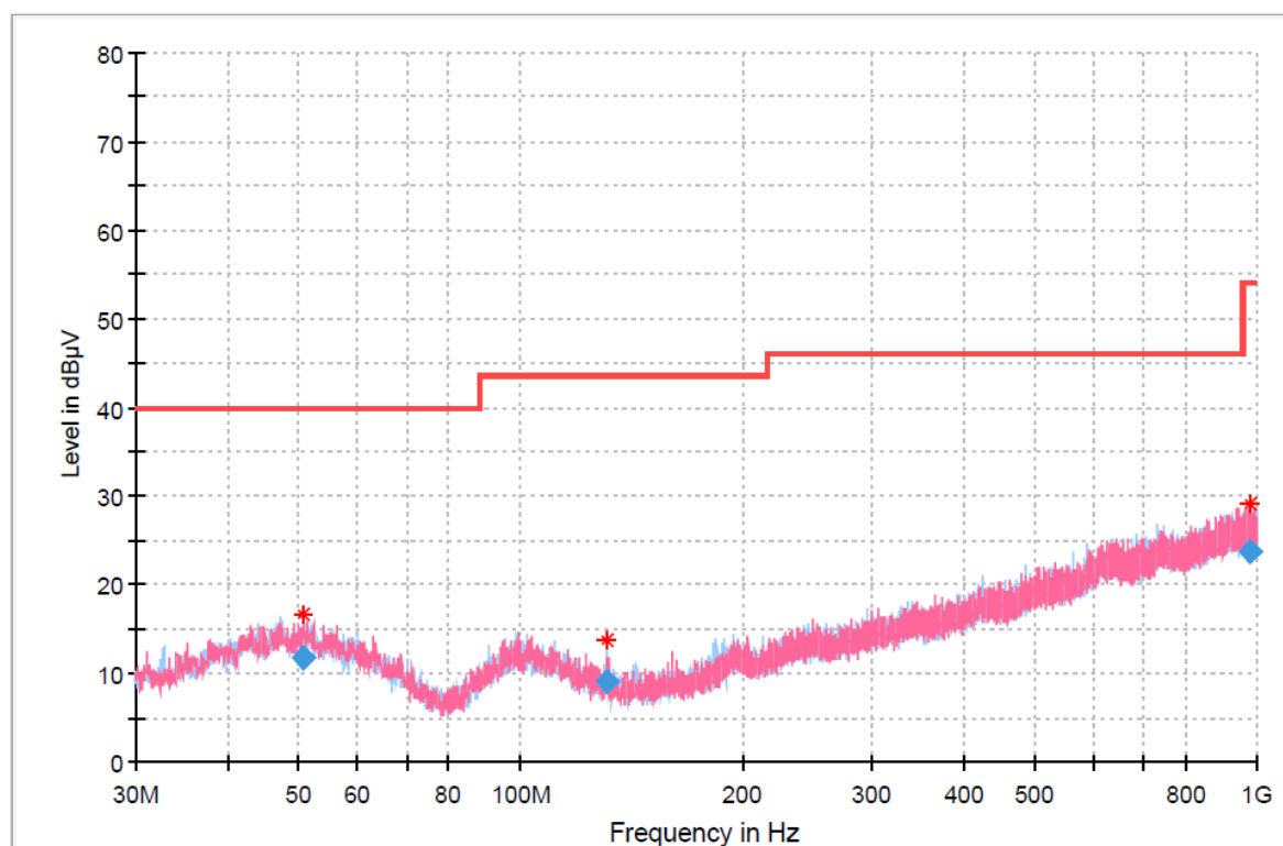
Worst case – RSE (Below 1 GHz)_TM 1
