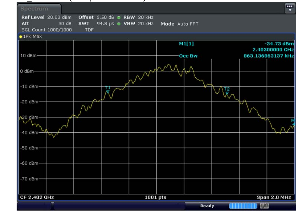
GFSK_2 402 MHz(Occupied Bandwidth)
