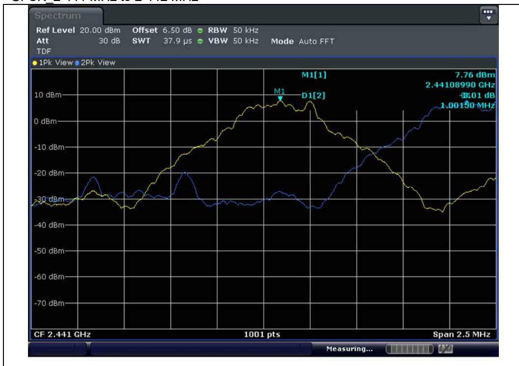
GFSK 2 441 MHz to 2 442 MHz
