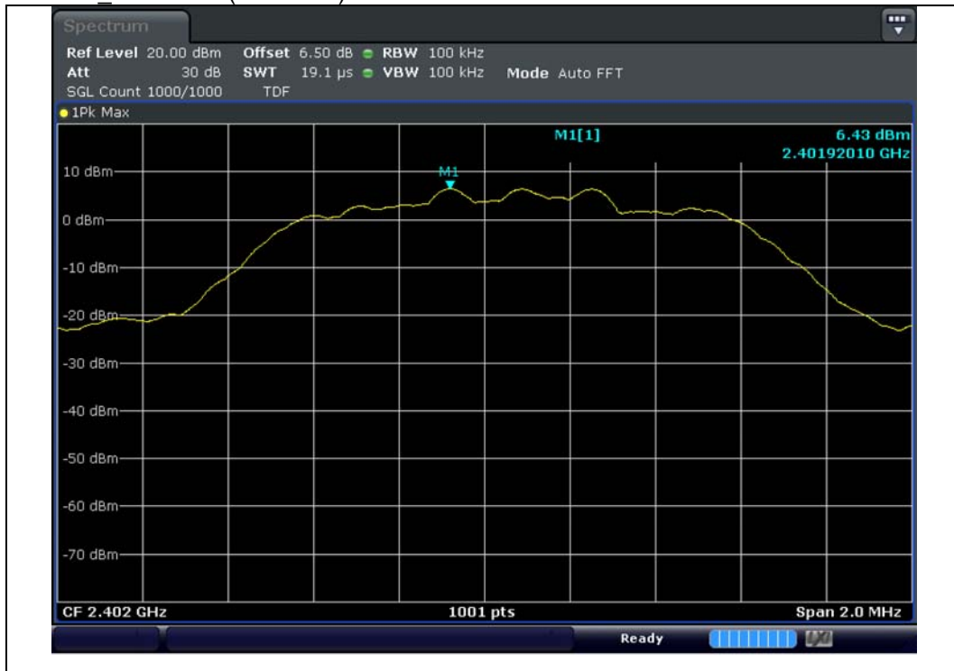
8DPSK_2_402 MHz(reference)
