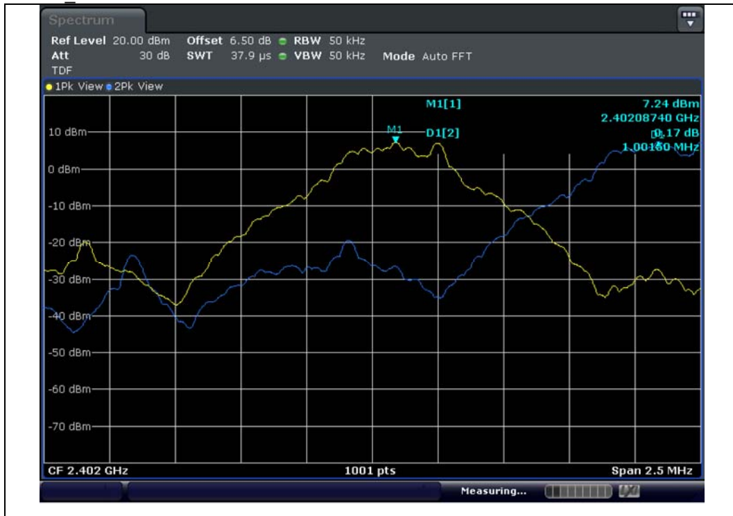
GFSK 2 402 MHz to 2 403 MHz
