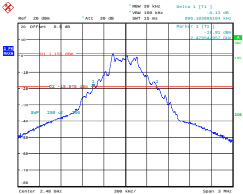
GFSK_High 0.896MHz
