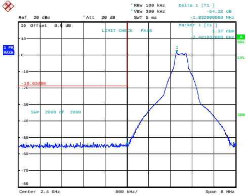
GFSK_Low 54.22dB
