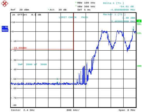
GFSK_Hopping_Lower 54.61dB
