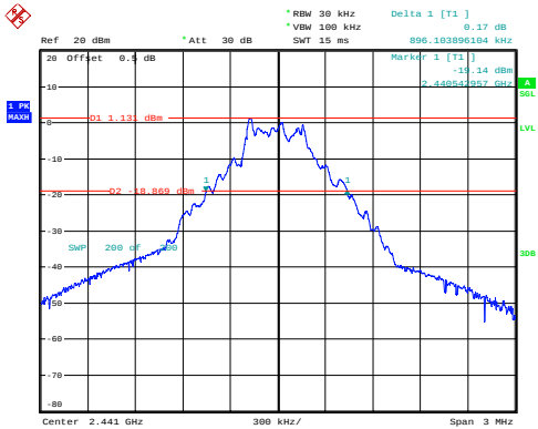
GFSK_Middle 0.896MHz
