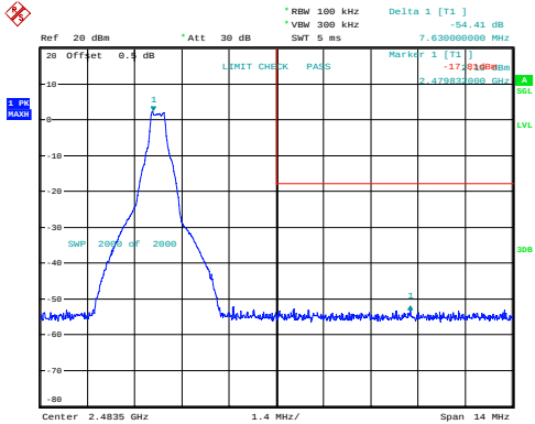
GFSK_High 54.41dB
