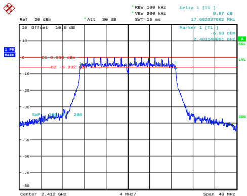
n20_2412MHz_Chain 0 17.662MHz
