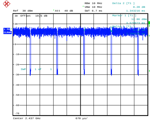
n20_2437MHz_Chain 0 1.298ms,1.343ms
