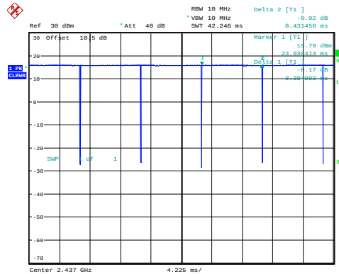
b_2437MHz_Chain 0 8.385ms,8.431ms
