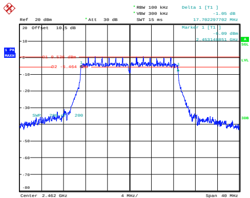
n20_2462MHz_Chain 0 17.702MHz
