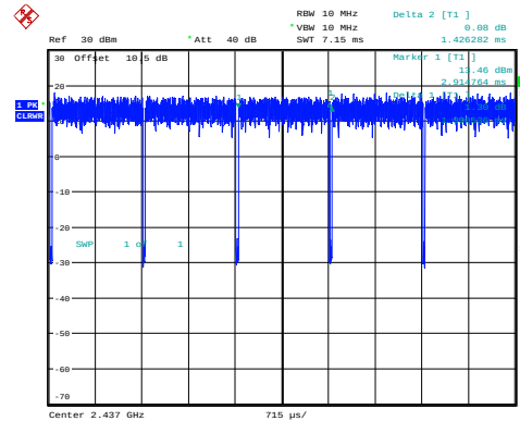
g_2437MHz_Chain 0 1.391ms,1.426ms
