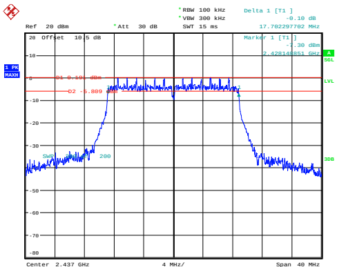
n20_2437MHz_Chain 0 17.702MHz
