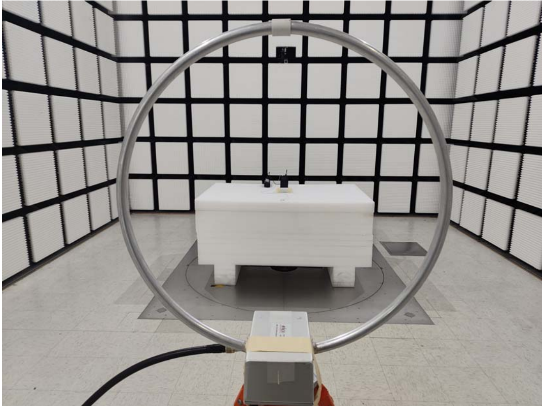
9kHz~30MHz _ Radiated Emission View - Perpendicular_ Adapter 1
