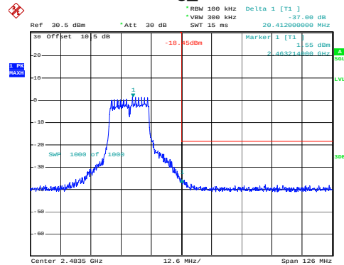
802.11g_2462MHz
