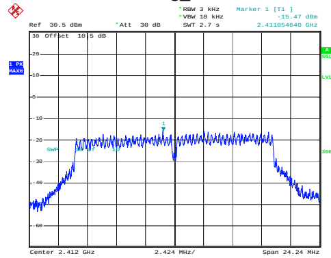
802.11g_2412MHz
