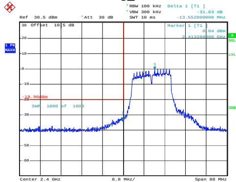
802.11g_2412MHz
